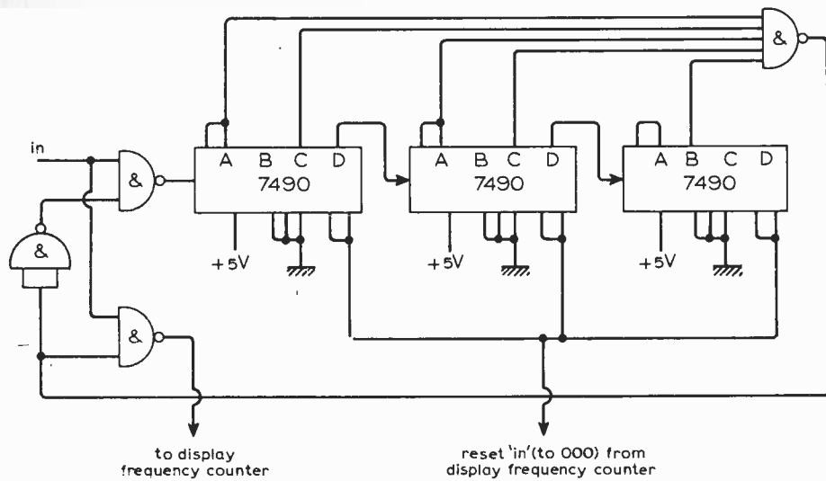
Circuit to subtract 455Hz from 'in' and gate remaining pulses to an external counter. To subtract 455kHz add preceding ÷ 1000 counter.
