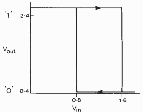
Fig. 2. Characteristics of Schmitt trigger NAND gate.
