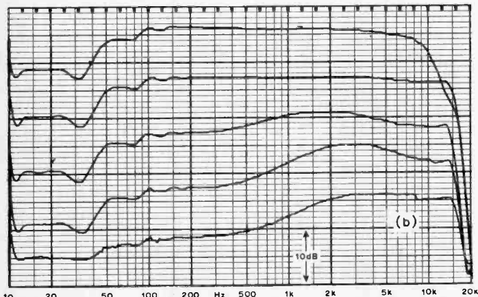
Fig. 9. Frequency sweeps recorded in 10dB steps with the Dolby noise reduction system switched in and played back with it in (a), and with it out (b).
