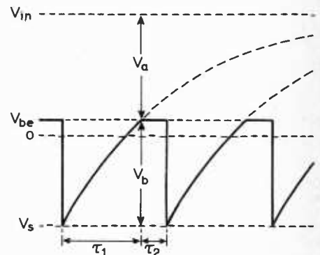
Fig. 3. Waveform at A.
