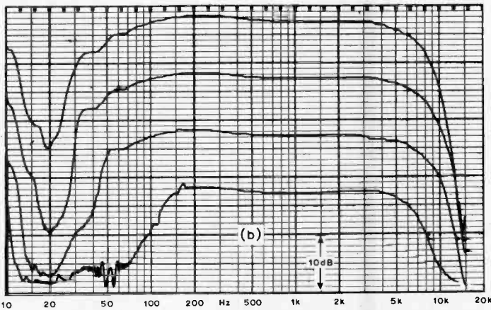
Fig. 10. Frequency sweeps recorded in 10dB steps and played back in (a) with the National NFD system out and (b) with it in.
