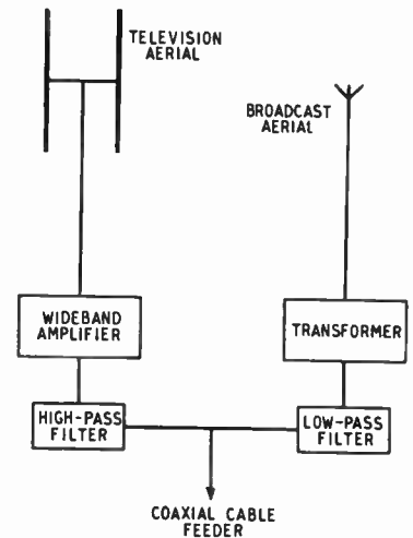
Fig. 4. Communal distribution system for both television and sound broadcasting.
