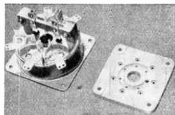
Webb's Radio screened and open style valveholders for the 829 type valve.
