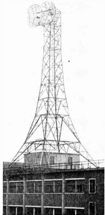
TOWERING 175 feet above London's streets is this new aerial, the first of six to be erected between the capital and Birmingham for the television link. The paraboloids have built-in electrical heaters for de-icing. This terminal station, designed by G.E.C., is at the Museum telephone exchange, Tottenham Court Road.
