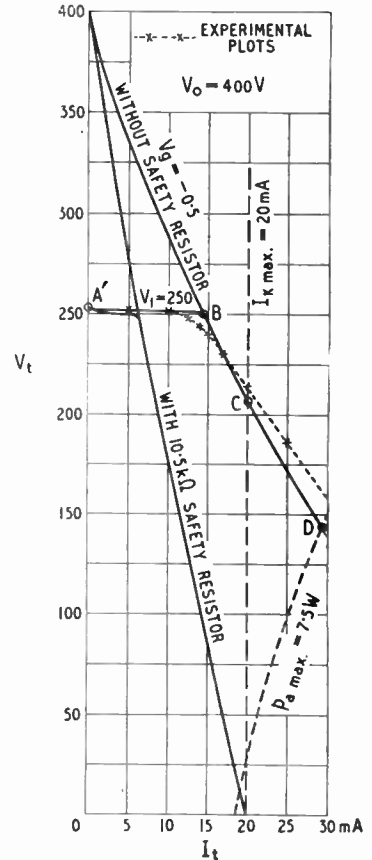
Fig. 2. I_a/V_t characteristics of EC52, illustrating properties and design of electronic tapping.
