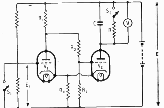
Fig. 2. Combined trigger and charging circuit.
