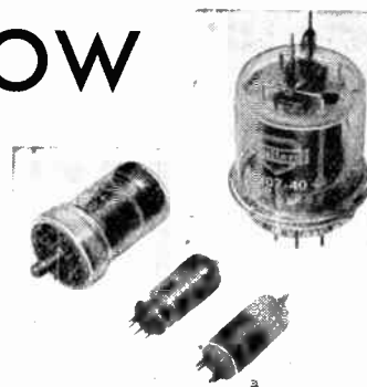
Mullard valves for V.H.F., the QV04-7, ECC91, EC91 and (at back) the QQV07-40.
