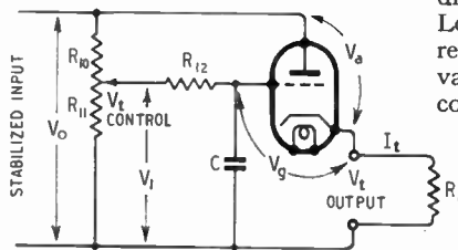
Fig. 1. Stable-voltage "electronic tapping," with output adjustable over nearly the whole range of V_0 .
