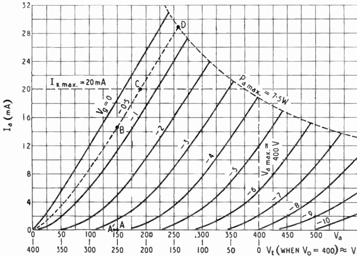
Fig. 2. I_a/V_t characteristics of EC52, illustrating properties and design of electronic tapping.
