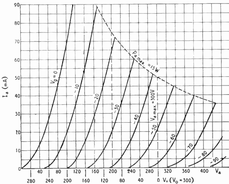
Fig. 5. Characteristic curves of low- \mu valve (PX4), for tapping to provide relatively heavy current.
