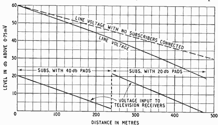
Fig. 2. Performance of the system shown in Fig. 1, giving line distribution characteristics (one subscriber per 15 metres).
