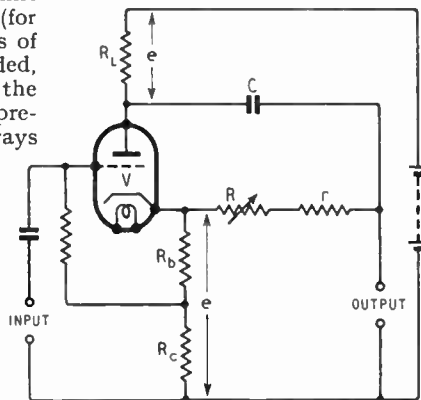
Fig. 4. Transformerless phase shifter. Typical values: V = EC91 ; R_L = R_C = 2.2 \text{ k}\Omega ; R_b = 100 \Omega ; H.T. supply 250 V, 10 mA. At input frequency about 100 kc/s, C = 50 \text{ pF} . R = 50 \text{ k}\Omega (carbon), r = 8.2 \text{ k}\Omega .
