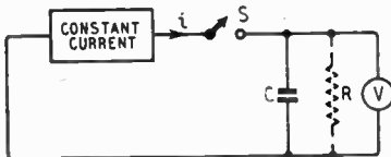
Fig. 1. Schematic circuit of interval timer.
