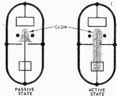
Fig. 4. Extent of glow discharge in the active and passive states.
