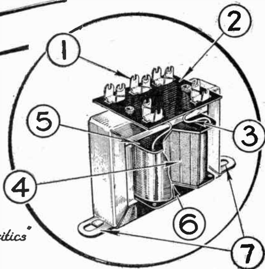
A.F. Voltage & Small-power Transformers & Chokes for all types of electronic apparatus, in all normal ratings and in a diversity of physical sizes.
