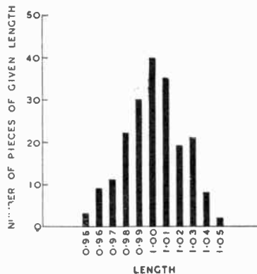
Fig. 1. A typical histogram.
