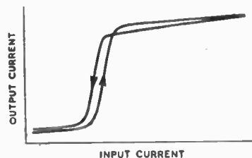
Fig. 5. Input-output characteristic of the Teleion.
