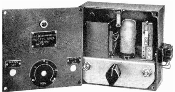
Type P.T.101A electronic process and delay timer.
