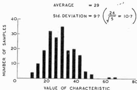
Fig. 4. Sampling from a skew distribution. (From BS600R:1942.)
