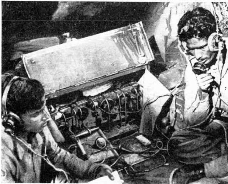
INDIAN SIGNALS. The general-purpose low-power No. 22 transceiver, which has facilities for both 'phone (5W) and CW (15W), in use in the Burma campaign. Men of the Fifth Indian Division are operating the set which has a frequency coverage of from 2-8 Mc/s.
