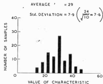
Fig. 4. Sampling from a skew distribution. (From BS600R:1942.)
