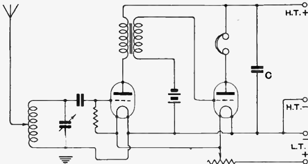
Fig. 1.—A normal 2-valve receiver with detector and low-frequency amplifier.
