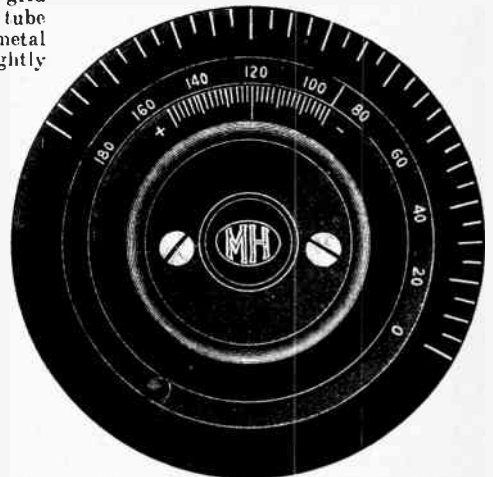
The McMichael vernier dial provides a direct rotation of the instrument spindle for coarse adjustment, whilst the vernier controlled by the centre knob gives a critical control.
