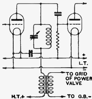
Fig. 5.—Tuned anode coupling between the last reflex valve and the detector.
