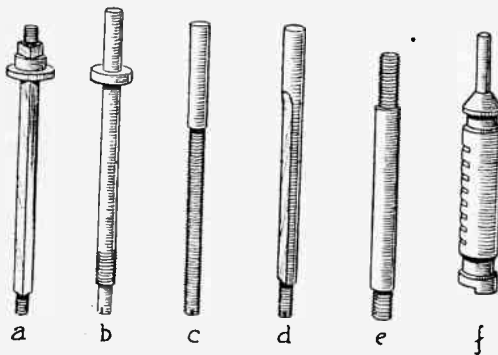
SPINDLES. (a) The square shaft with elaborate top collar and bearing. (b) A good form turned from large diameter rod to produce the collar. (c) The threaded stem. (d) Cut away shaft to which the plates are secured by collars having "D" shaped holes. (e) A threaded spindle passing through the top bearing is unsatisfactory. (f) Here the plates are soldered into slots on a sleeve, slipping over a plain spindle. A conical top thrust bearing is provided together with a cut away piece at the bottom to serve as the stop.
