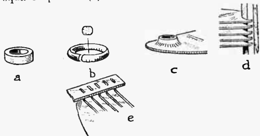
SPACING WASHERS. (a) The turned brass washer (b) Flattened wire ring. (c) Pressed up spacer used in conjunction with a thin stamped washer.
