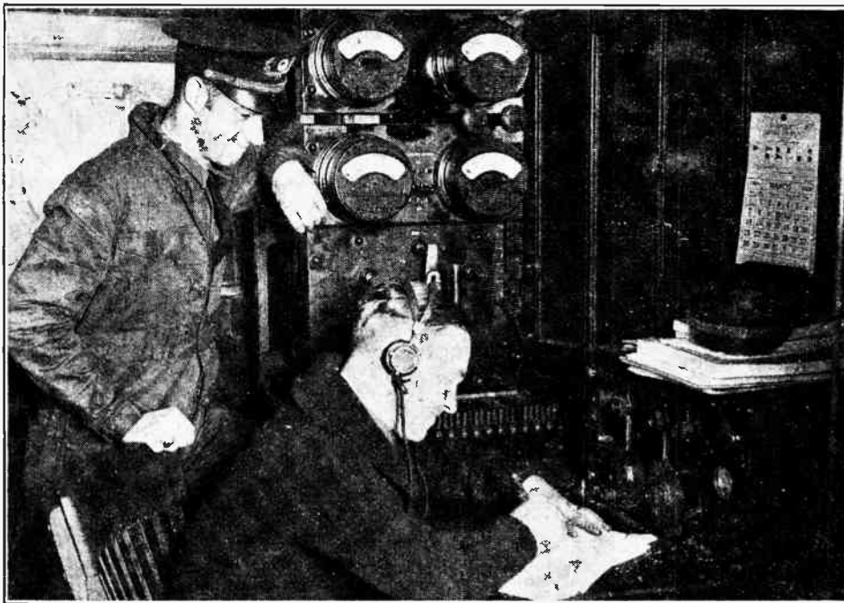
The commercial 1 kW. Marconi quenched-spark set of the "Chantier."
