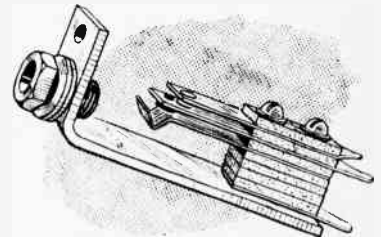
The tag connectors of the Igranic Pacent jack are turned alternatively in each direction to facilitate soldering.
