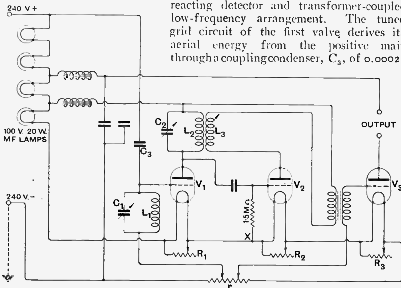
Fig. 1.—Complete circuit diagram of the receiver.
