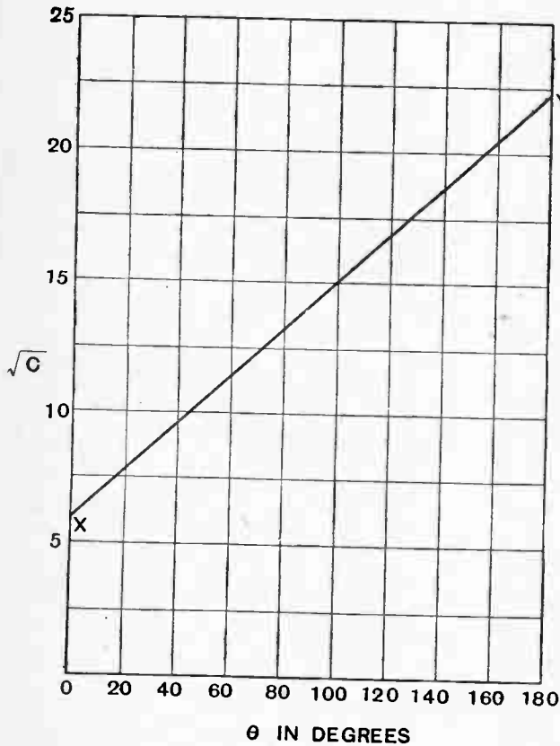
Fig. 2.—Curve showing relation between scale reading and square root of capacity for a square law condenser.
