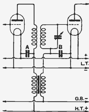
Fig. 1.—Method of coupling valves amplifying at both high and low frequencies.
