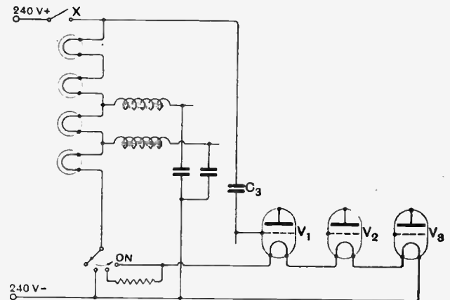
Fig. 6.—Connections of special switch to prevent current surges when switching on.
