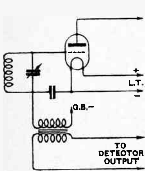
Fig. 8.—"Series" method of connecting detector output to first reflex valve.
