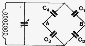
Fig. 4.—Equivalent electrical circuit for the capacities shown in Fig. 3.
