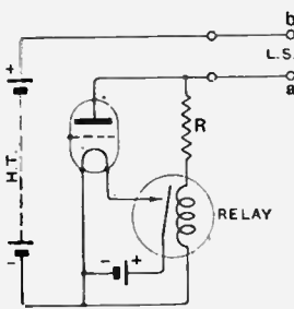
Fig. 4.—Connections of the relay circuit.
