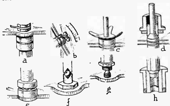
THRUST BEARINGS. (a) The fibre ring, a reliable method of controlling end play. (b) and (c) The spring washer should not be found in a precision instrument. (d) Adjustable conical thrust bearing. (e) The ballrace is perhaps unnecessarily elaborate. (f) A single ball now much used in British condensers. (h) Adjustable lower bearing with hollow spindle for linking up with the spindle of another condenser.
