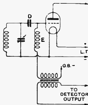
Fig. 9.—The "parallel" method of connection complementary to Fig. 8.
