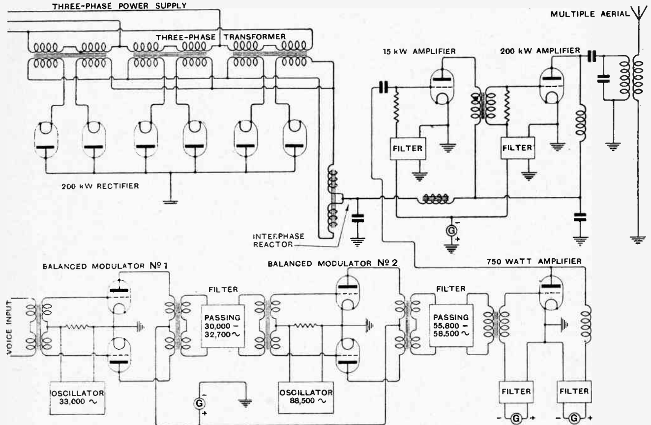
Fig. 2.—Simplified circuit of the transmitter at Rocky Point, Long Island.
