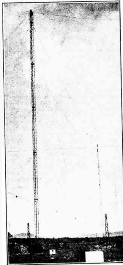
A MODERN HIGH POWER STATION. The aerial and earth screen at Rio de Janeiro. The aerial, which is 800 feet high, was erected by the Marconi Company, together with the earth screen and its supporting wires.
