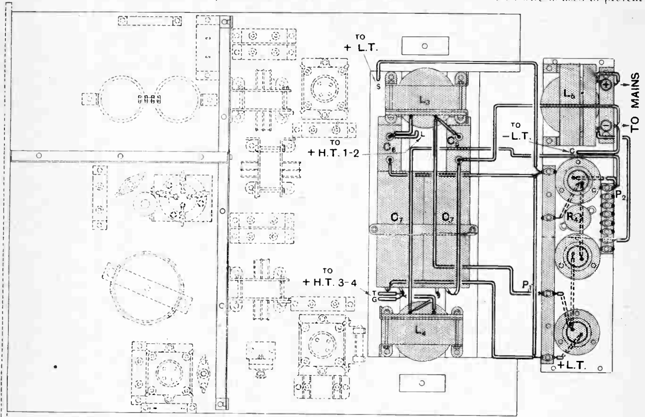
Fig. 6.—Wiring diagram of power unit.
