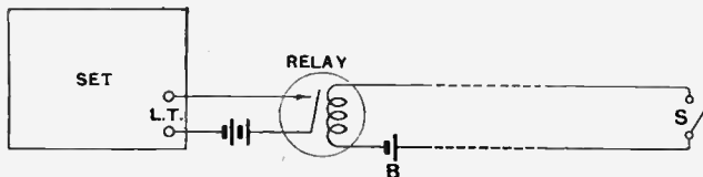
Fig. 2.—The simplest method of controlling L.T. current by means of a relay.
