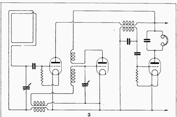
The phones are now transferred to the anode circuit of the first I.F. amplifier, which is converted to a second detector by the insertion of a leaky grid condenser. This test will provide a check on the operation of this valve, and also of the frequency-changing arrangement as a whole, although loud signals should not be expected.
