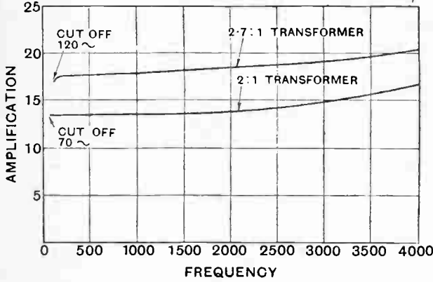
Fig. 5.—Approximate overall characteristic of amplifier in Fig. 4 with resistance R in anode circuit of detector. 2.7:1=50 henries, 2:1=100 henries.
