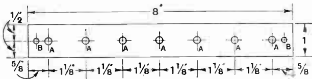
Fig. 6.—The terminal panel. A, \frac{3}{8} in. dia.; B, \frac{1}{2} in. dia.
