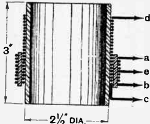
Fig. 2.—Sectional sketch showing details of the H.F. transformer.
