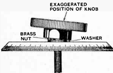
Condenser dial adjustment.
