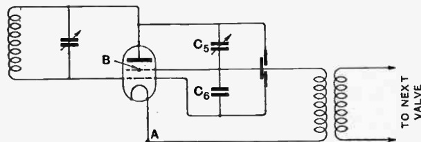
Fig. 5.—Complete circuit of the four-electrode H.F. amplifying valve and its associated coupling circuits.
