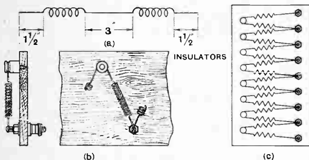
Fig. 2.—Details of simple potential divider
