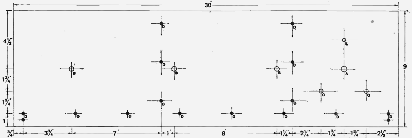
Fig. 5.—The ebonite front panel. A 1/4", B 1/4", C 1/4", D 1/4" and countersunk.
