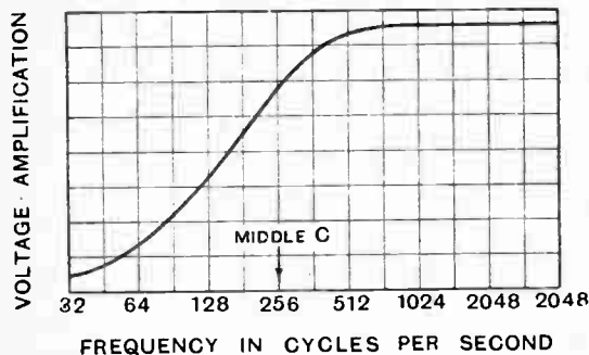
Fig. 1.—Form of voltage amplification curve of double note amplifier under following conditions: Detector valve "R" followed by 3:1 transformer (primary 40 henries); first amplifier, D.E.5, followed by 4:1 transformer (primary 15 henries).
