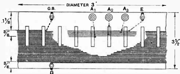
Fig. 2.—Constructional details of the input transformer. The tapped primary winding is connected to the aerial circuit and the larger coil is connected to the grid and filament of the first valve.
