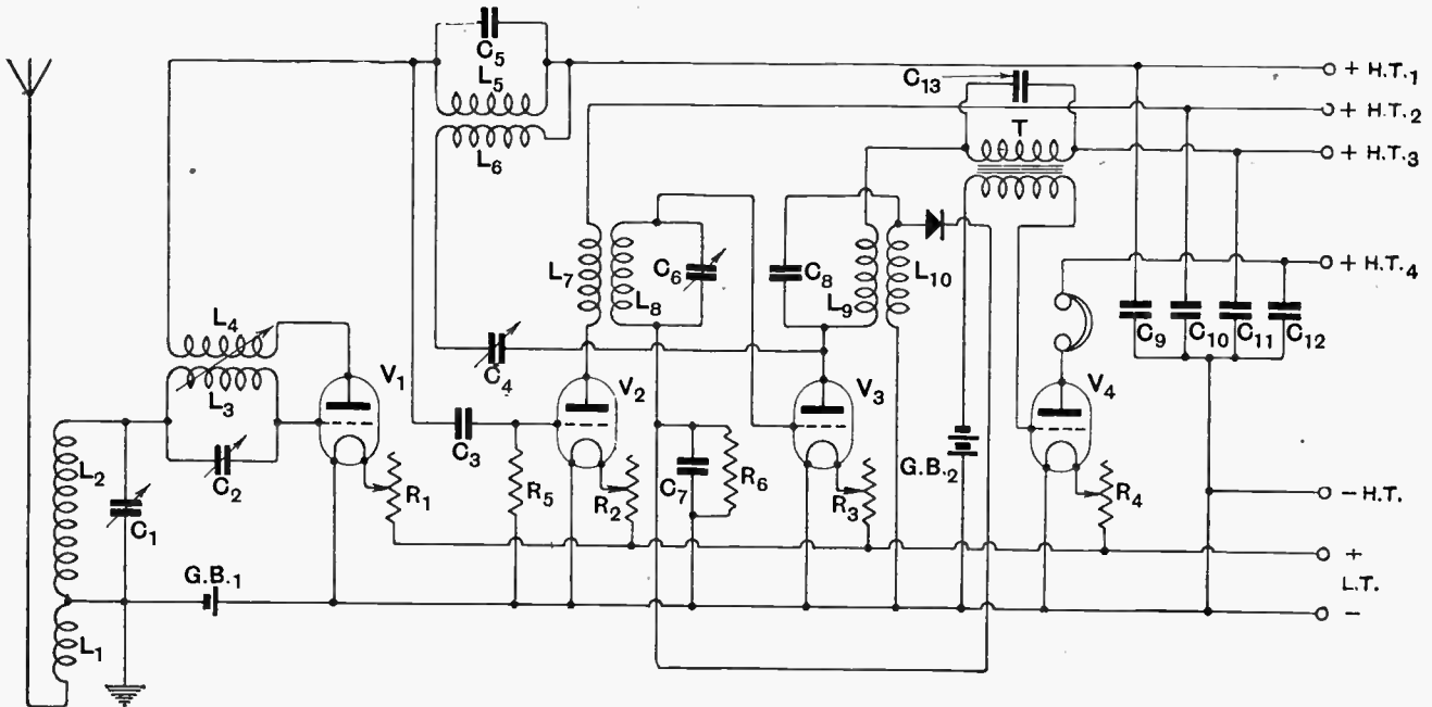
Fig. 2.—A four-valve reflex superheterodyne receiver.
