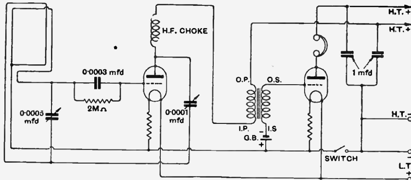
Fig. 1.—Capacity reaction in a frame aerial receiver.
