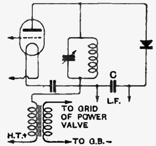
Fig. 7.—In a circuit of this type a steady potential will be applied to the crystal, due to the anode current and the D.C. resistance of the tuned anode coil.
