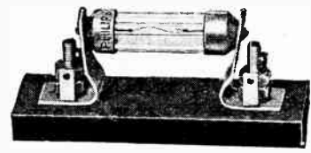
The Philips filament protecting fuse.
