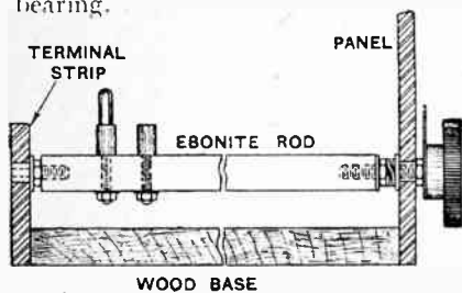
Variable mounting for plug-in coil
