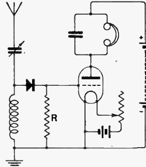
Fig. 5.—Simple crystal receiver with valve amplifier.
