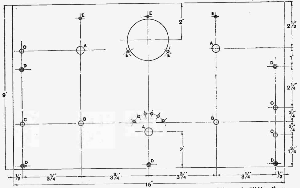
Fig. 2.—Dimensional details of the front panel. Drilling sizes are as follow: A, 7/16in. dia.; B, 1/2in. dia.; C, 7/32in. dia.; D, 1/4in. dia. and countersunk for No. 4 wood screws; E, 1/2in. dia.
