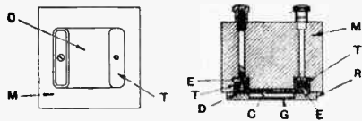
Details of the Reisz microphone. (No. 250,430.)
