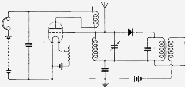
Fig. 1.—Reflex circuit with valve reaction.
