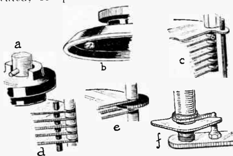
STOPS. (a) Moulded end piece with stop pin. (b) A stop under the dial is difficult to fit and requires a pair of screw heads on the instrument panel. (c) Extensions on two of the fixed plates to support an ebonite rod. (d) Ebonite rod carried in holes in the fixed plates. (e) Insulating washer as stop and pin stop.
