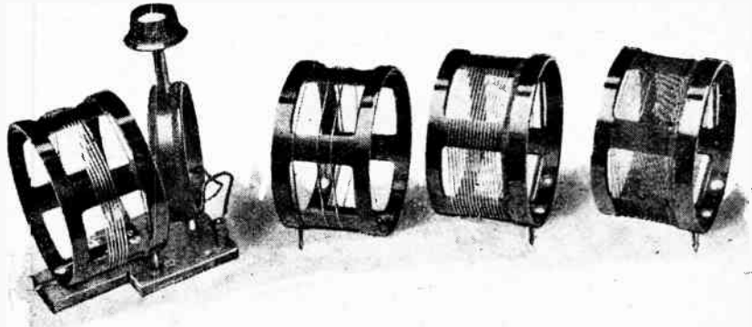
The Bremer Tully short-wave tuning outfit comprises a set of well-designed short-wave inductances covering a range of 12.5 to 200 metres.
