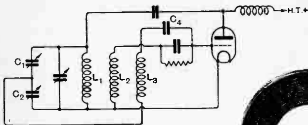
Fig. 1.—The basic circuit of the transmitter.
