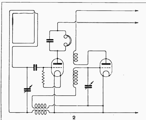
The first detector and its associated circuits may be tested by connecting the phones in series with its anode. Unless near to a broadcasting station, it may be necessary to couple an aerial system to the frame. The operation of the oscillator may be checked by noting if a beat note with the incoming carrier wave is produced when its tuning is varied.
