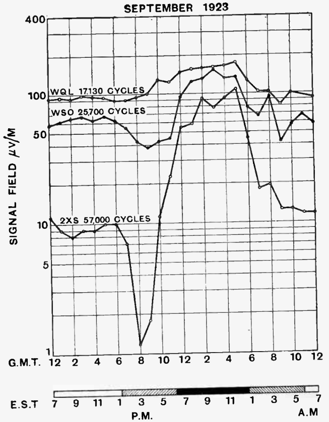
Fig. 8.—Average diurnal variation in field strength of three American stations received at New Southgate, London, during the month of September, 1923. Antenna currents were as follow: WQL, 600 amps.; WSO, 600 amps.; 2XS, 300 amps.
