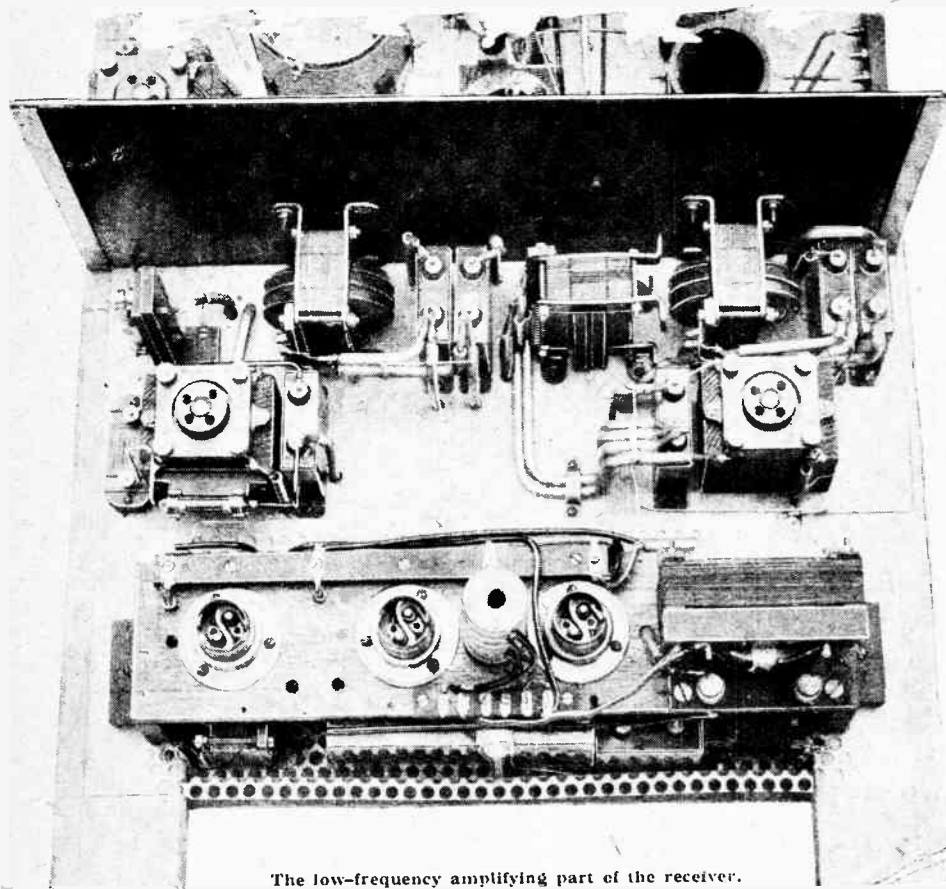
The low-frequency amplifying part of the receiver.
