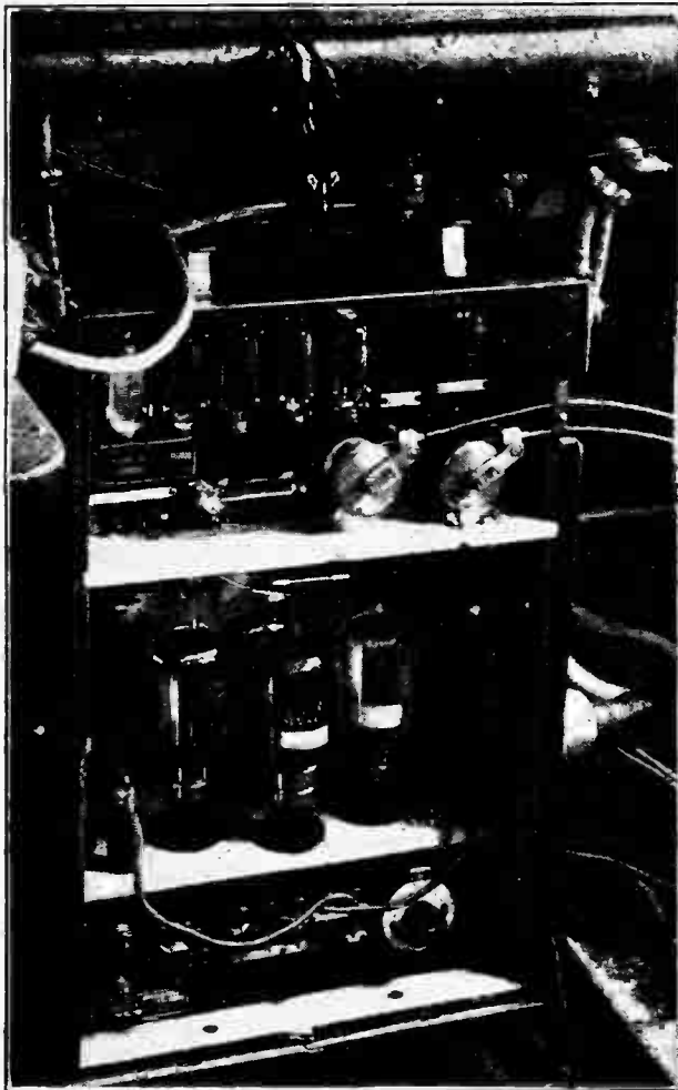
Standard Marconi A.D.6 aircraft transmitter and receiver used in the tests.
