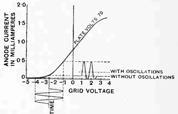
Fig. 1.—Diagram showing how the mean value of the plate current is increased by applying an oscillating E.M.F. to the grid when the valve is operated at the lower bend of the anode characteristic.
