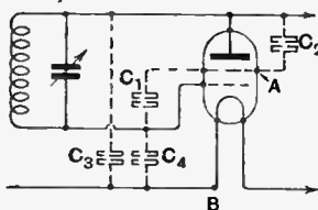
Fig. 3.—Inter-electrode capacities in the four-electrode valve.
