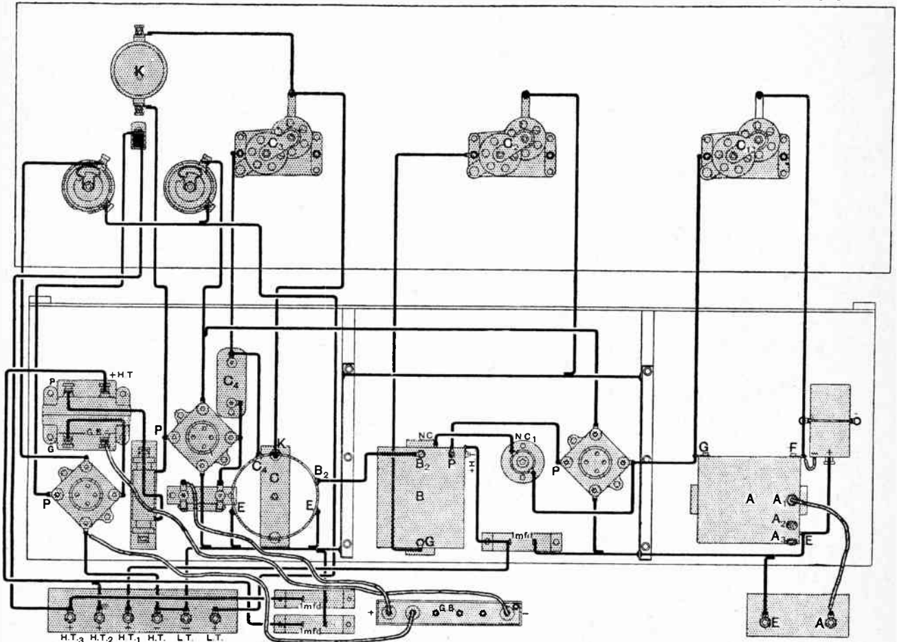
Fig. 7.—Wiring diagram. C 1 , C 2 and C 3 , 0.0005 mfd. tuning condensers; A, B and C, the three secondary windings; NC 1 , balancing condenser; C 4 , 0.0003 mfd. fixed condenser; K, reaction condenser; GB, grid bias battery.
