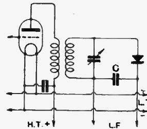
Fig. 6.—Connections of a crystal rectifier in a reflex receiver with H.F. transformer coupling to the preceding valve.
