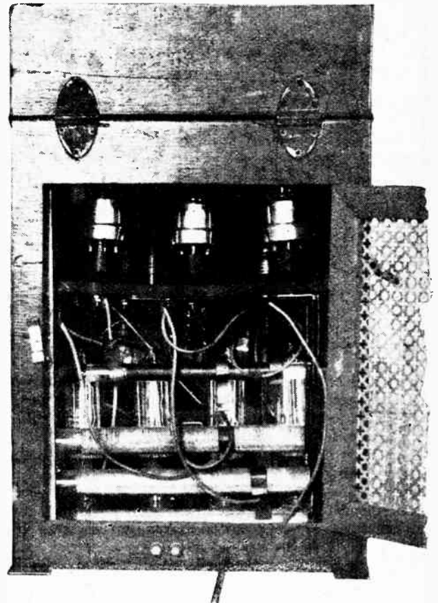
Fig. 3.—Back view of cabinet showing ventilating door and tubular filament resistances.
