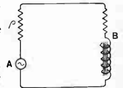
Fig. 6.—Equivalent electrical circuit of loud-speaker in the anode circuit of a power valve.
