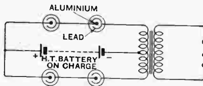
Fig. 2.—Electrolytic rectifier connections for battery charging.
