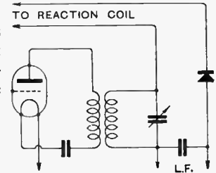
Fig. 11.—Showing how reaction may be used in a reflex receiver employing a crystal detector.
