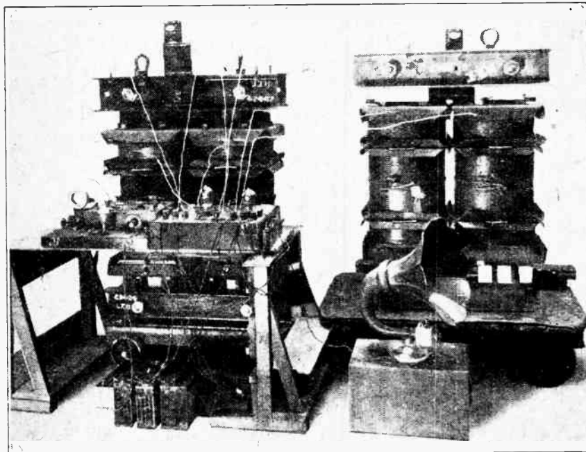
A progressive increase in size characterises the new types of intervalve transformer which have recently made their appearance on the British market. Pursuing this line of development to its logical conclusion, Messrs Ferranti, Limited, have recently tested a receiver in which the L.F. valves are coupled with two of their 150 kVA power transformers. It is stated that nearly perfect results were obtained!
