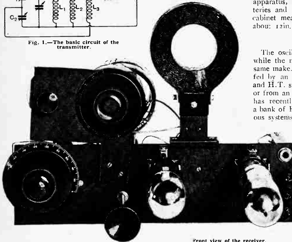
Front view of the receiver.
