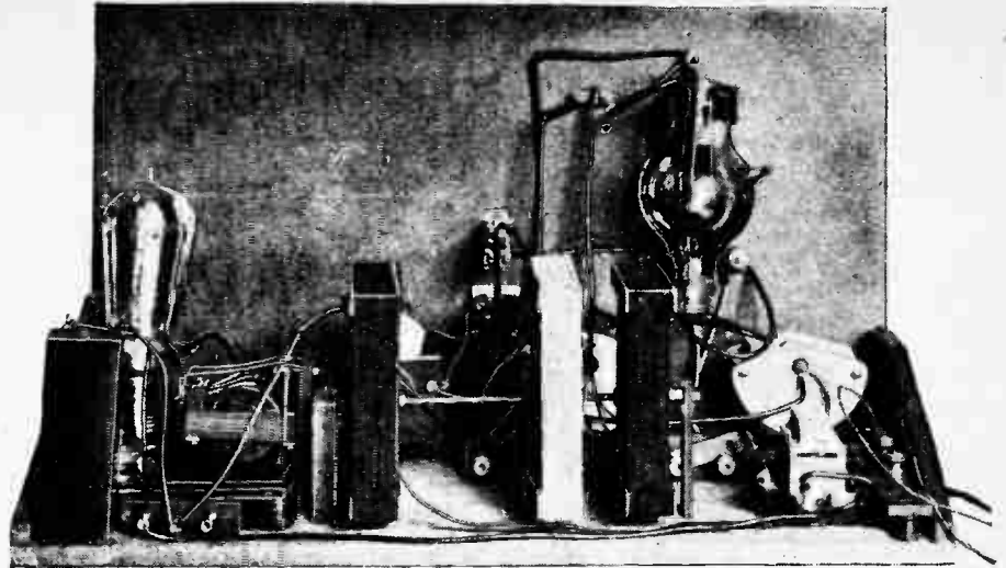
The arrangement of the transmitting apparatus.
