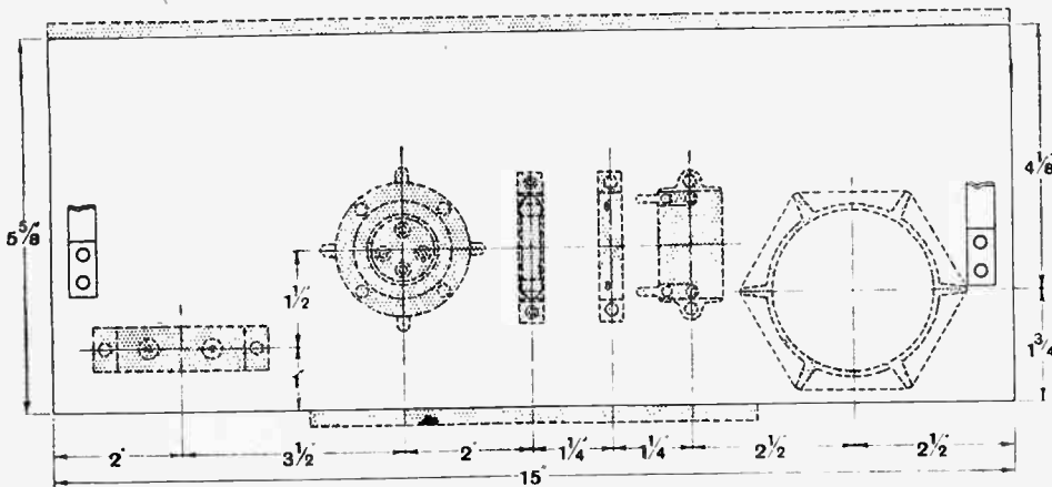
Fig. 3.—Layout of baseboard. All components should be well spaced as shown.
