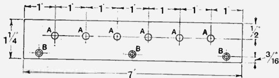
Fig. 4.—Details of terminal strip. A, \frac{7}{32} in. dia.; B, \frac{1}{8} in. dia and countersunk for No. 4 wood screws.
