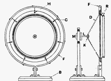
Cone diaphragm of special construction. (No. 241,869.)
