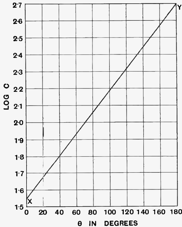
Fig. 9.—The relationship between scale degrees and the logarithms of capacity values.
