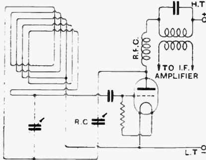
Fig. 1.—Modifying a superheterodyne.
