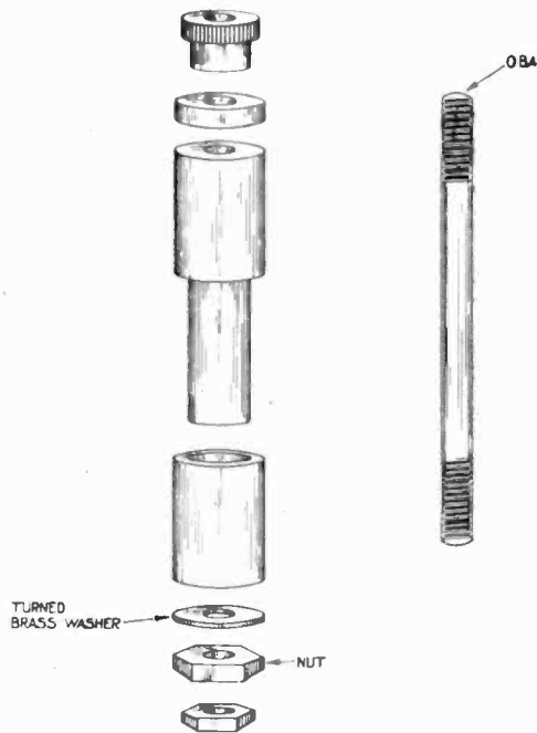
Fig. 3. Insulating Bushes.
