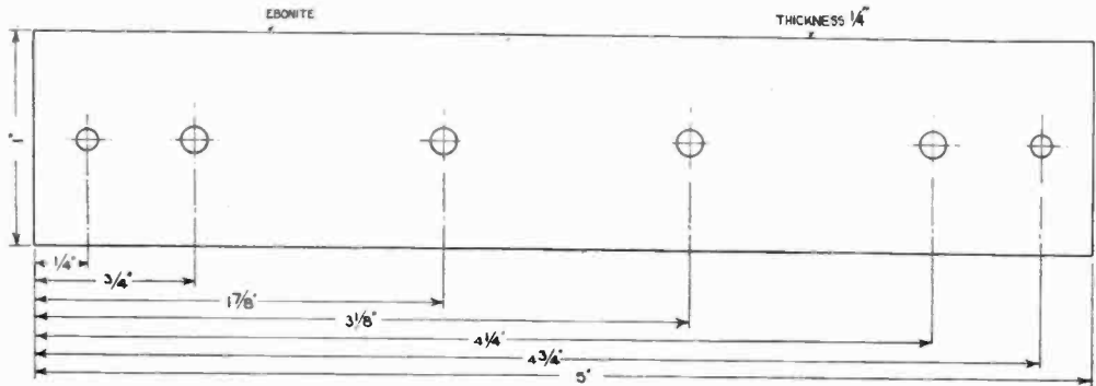
Fig. 5. The ebonite piece for mounting the terminals. The thickness is \frac{1}{4} ".
