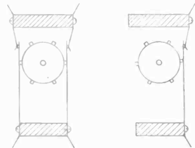
Fig. 3. Sectional view of simple barrel switches.
