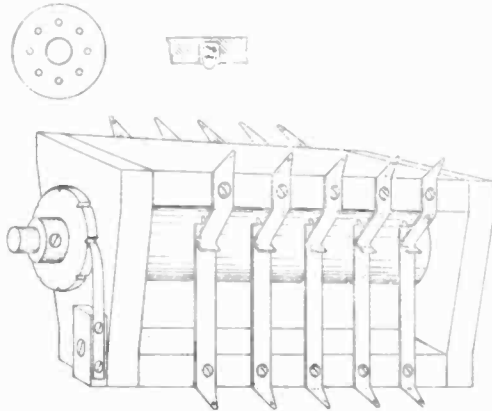
Fig. 2. A simple rotating switch.
