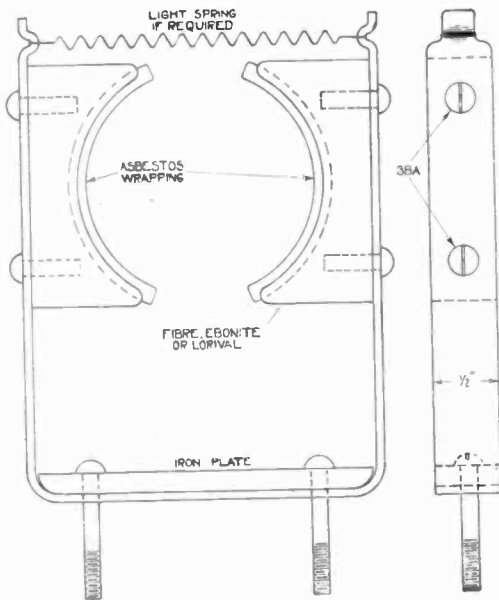
Fig. 4. Clips for supporting valves.
