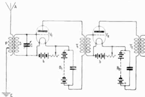
Fig. 96. Arrangement of two or more amplifying valves for magnifying the feeble oscillations in the aerial wire A. V_1 , V_2 , are the thermionic amplifiers T_1 , T_2 , the coupling transformers and B_1 , B_2 , the plate batteries.
