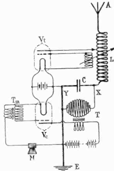
Fig. 104. A type of quiescent aerial with valve transmitter. The microphone M controls the supply of plate voltage in the transmitting valve V.
