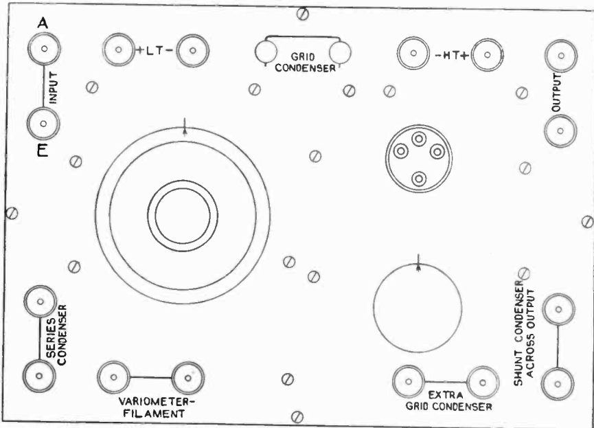
Fig. 3. Top of instrument showing terminal markings.
