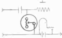
VARIABLE GRID CURRENT AND CONDENSER LEAK RECTIFICATION
