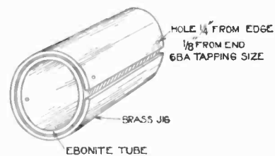
Fig. 3. The jig for the body.
