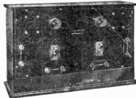
Two-Valve Broadcast Amplifier, No. M.H./B.R.2A.
