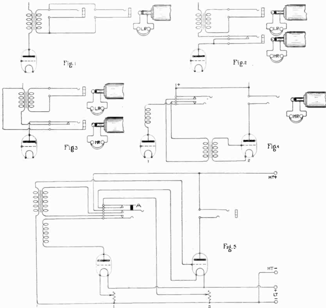
Figs. 1 to 5. Various arrangements for controlling L.F. Valves.
