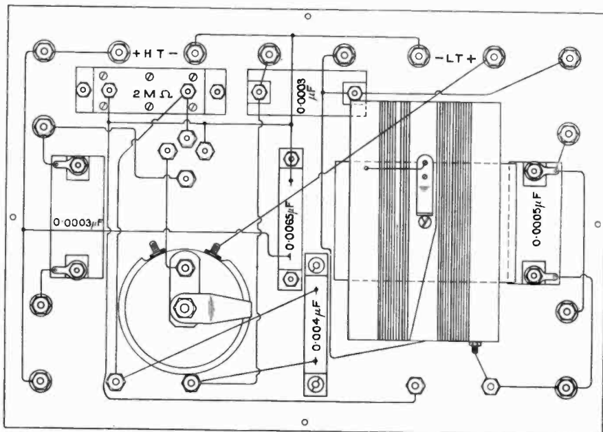
Fig. 4. Wiring diagram of the underside of panel.
