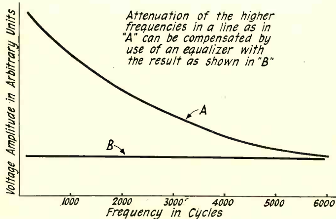
Graphic chart illustrating the use of equalizers in compensating for high frequency attenuation in line telephony
