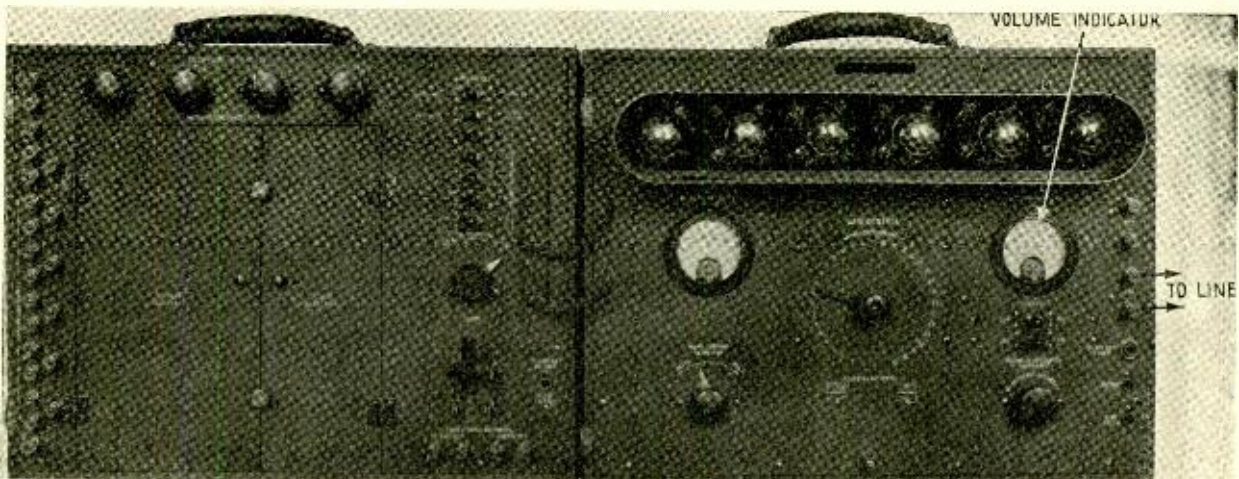
One type of line amplifier used for picking up events outside the regular broadcasting studio. To the left is the portable battery set and to the right is the amplifier set
