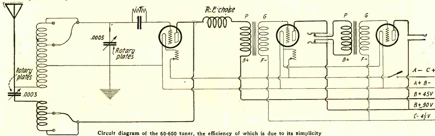
Circuit diagram of the 60-600 tuner, the efficiency of which is due to its simplicity
