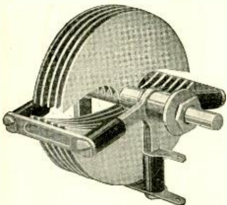
"Crofoot" Variable Condenser
