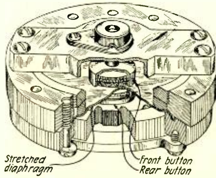
Double button carbon microphone
