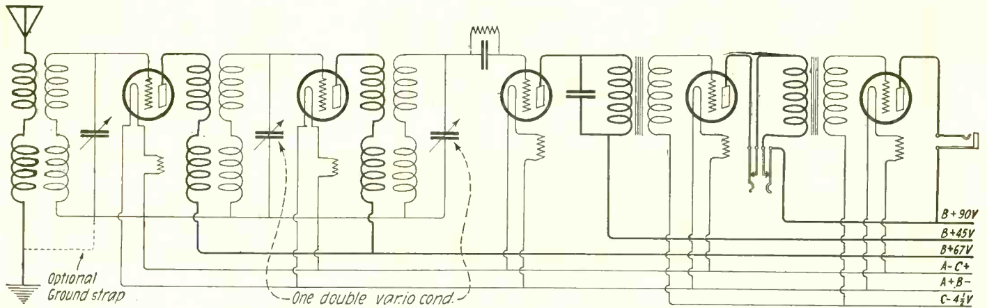
In the diagram note the second and third condensers. Their rotary plates are part of the common negative A lead. Their stationary are connected respectively to the grids of the second and third tubes
