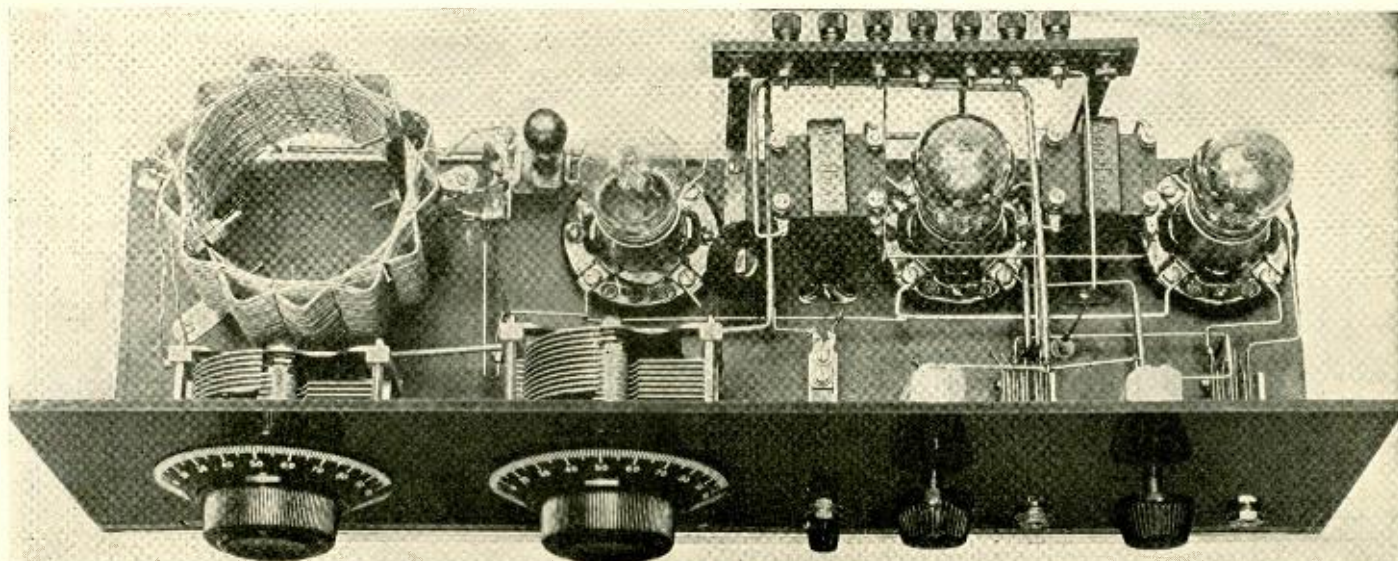
The clips for shorting the unused portions of the grid and plate coils and all other connections are clearly shown and no difficulty in placing the parts or hooking-up the set should be experienced
