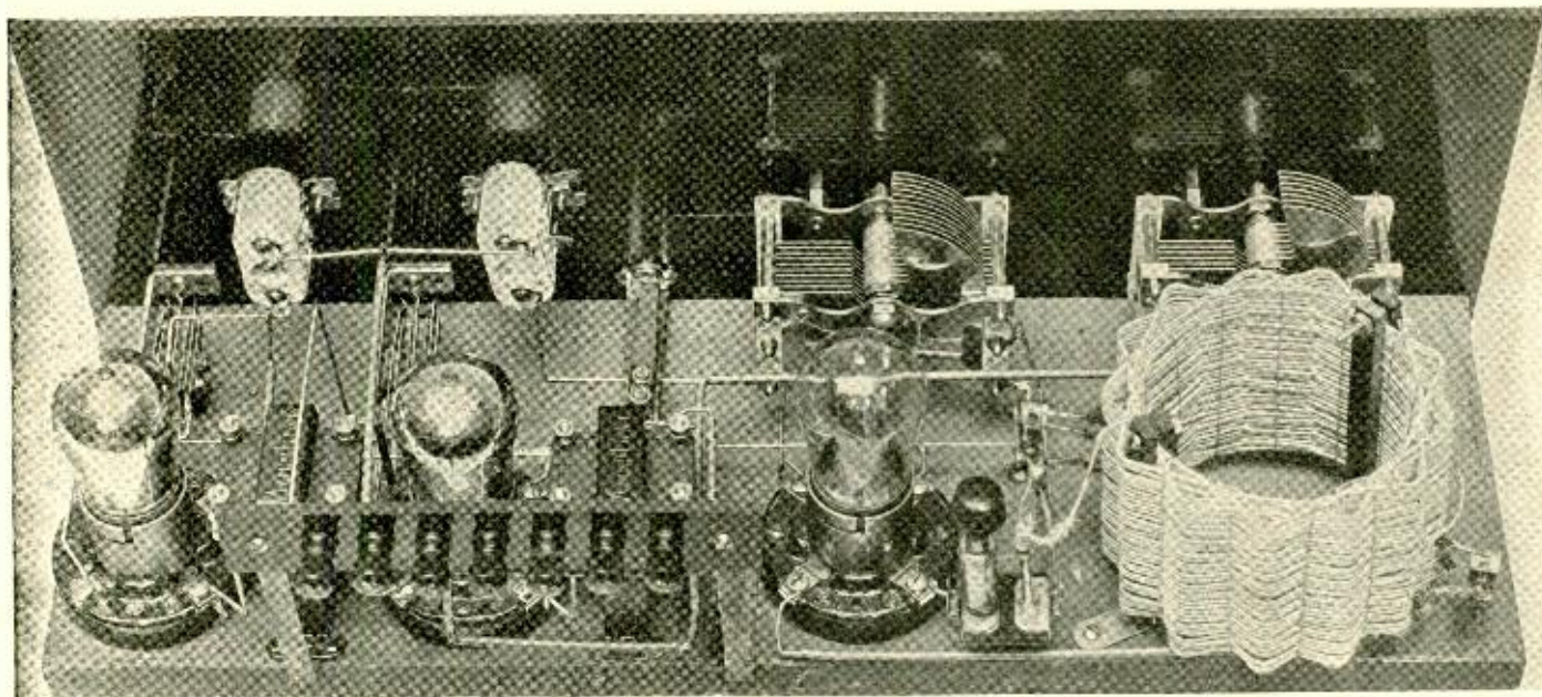
This illustration together with the one on the foregoing page should enable the most inexperienced to build the 60-600 receiver
