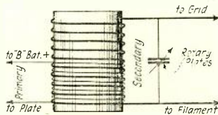
Diagram showing connections of the leads on the astatic transformer
