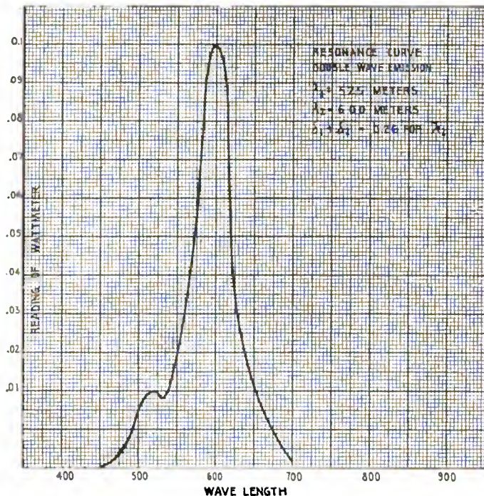
Figure 167—Resonance curve of the radiated wave of a radio transmitter, which complies with the U. S. regulations. The curve indicates that the antenna oscillates at two frequencies, one corresponding to a wave length of 600 meters, and the other to a wave length of 526 meters. The amplitude of the shorter wave is one-tenth of the longer wave and hence it meets the requirements of the U. S. Statute. Modern transmitters are generally adjusted for a single wave emission.
