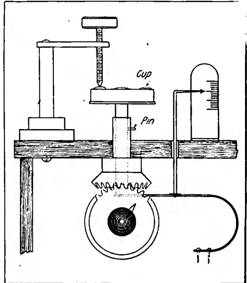
Figure 2—Showing construction plan of the detector holder
