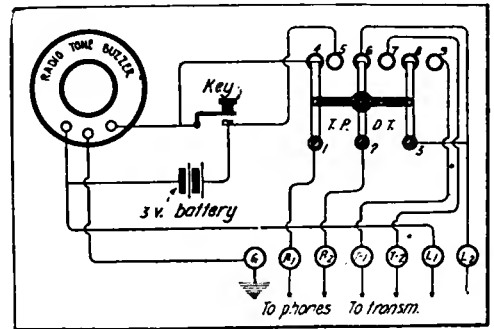
Figure 1—Circuit of field telephone and buzzer
