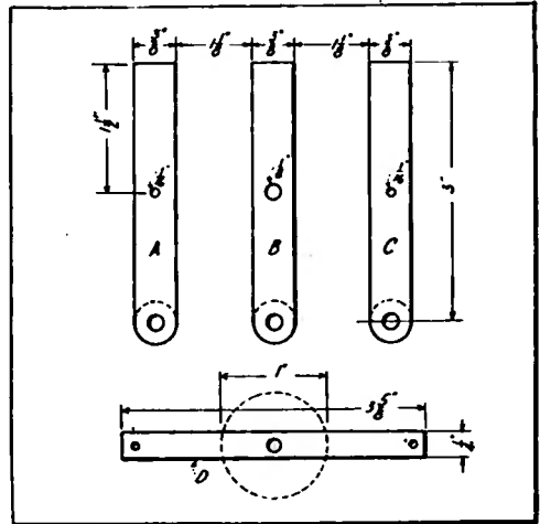
Figure 2—Showing position of cross arm
