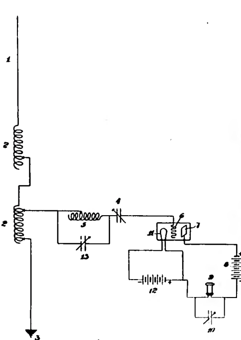
Figure 3—Receiving circuit to eliminate undesired signals
