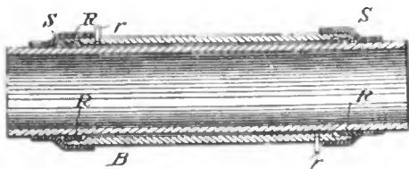
Figure 6—Section of quenched spark gap
