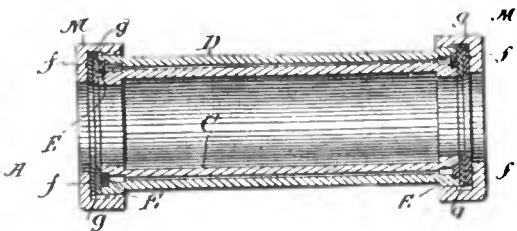
Figure 7—Modified construction of spark gap
