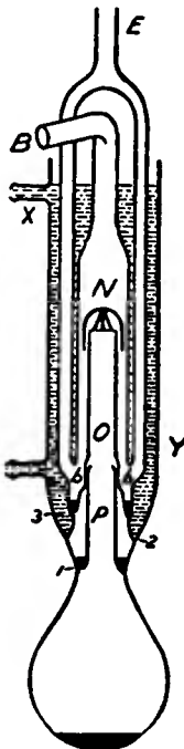
Figure 3—Diagram of high vacuum mercury vapor pump
