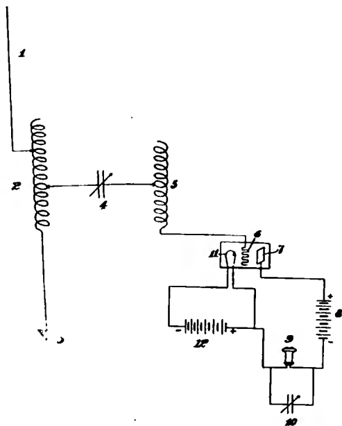
Figure 2—Amplifying receiving system devised by Bucher
