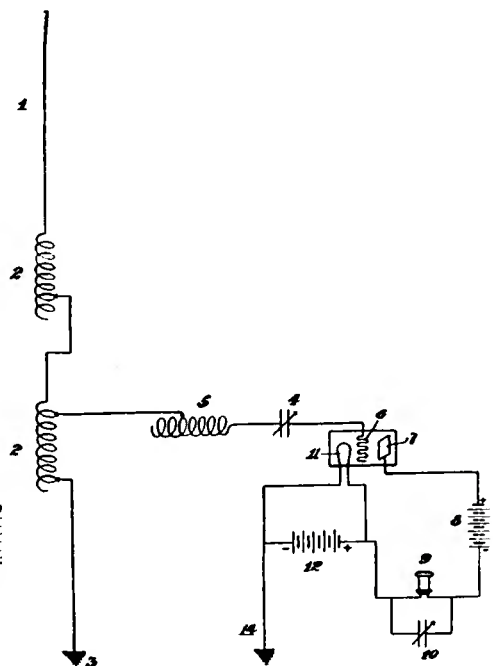
Figure 4—Receiving system with open circuit oscillator
