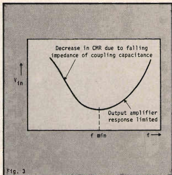
Fig. 3: Typical sinusoidal common mode rejection curve.
