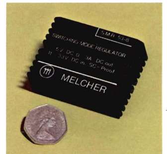
5V 3A DC/DC SMR53
