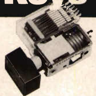
Series '200' Momentary, Locking, Interlocking, Cancel/Interlocking types. Barred Access and Blocking facilities. Up to 6 pole changeover.
