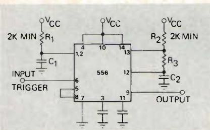
One burst generator - one of many uses for the 556 timer.
