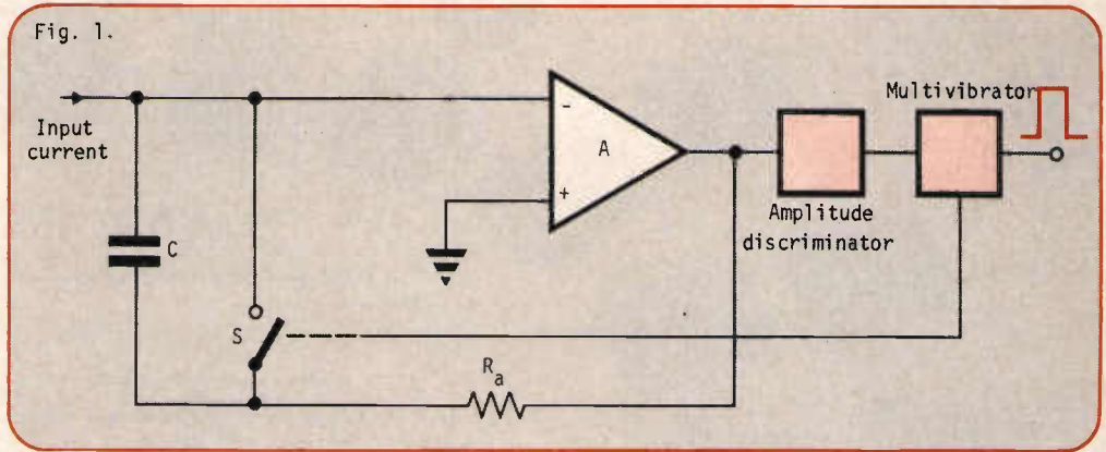
Fig. 1: Ordinary current-to-frequency converter requires switch with high insulation.
