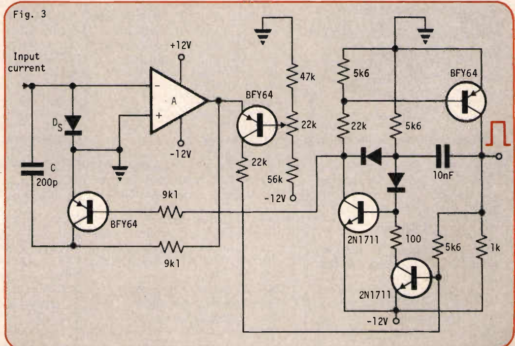
Fig. 3: A practical solution of the small-current-to-frequency converter.
