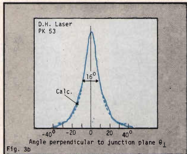
Fig. 3: For field emission pattern in the direction perpendicular to the junction for (a) five layer LGR lasers and (b) DH laser.
