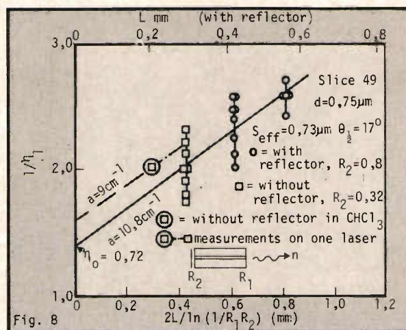
Fig. 8: Incremental quantum efficiency versus laser length for narrow beam LGR lasers. Fig. 9 As for Fig. 8 but for narrow beam DH lasers.
