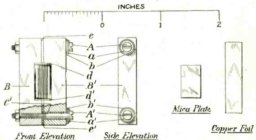
Fig. 1. Working Drawings
