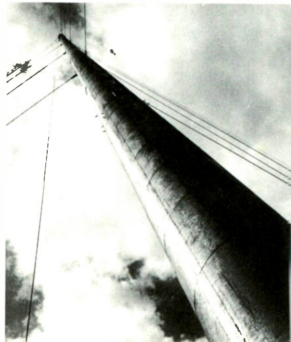
Nearly 1,300 ft of tubular steel, the Emley Moor mast which brought ITV to Yorkshire was the highest structure in Britain in 1956.
