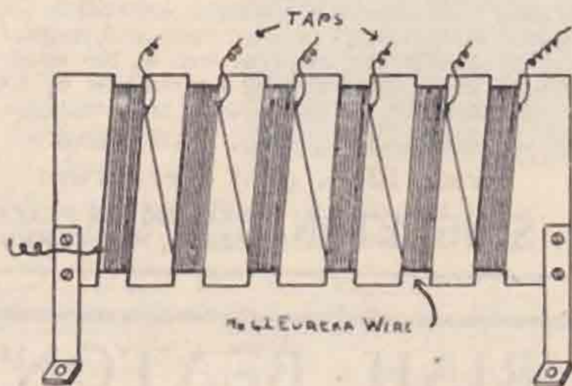
FIG. 3 GRIDLEAK
