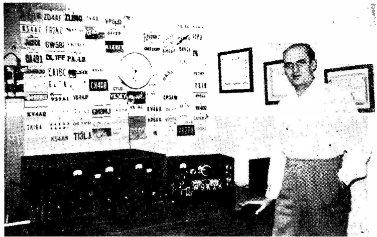
W9KXX, Waupaca, Wis., runs a Temco 600w. transmitter with an HRO receiver. His aerials are a two-element beam and a 40-metre ground plane.
