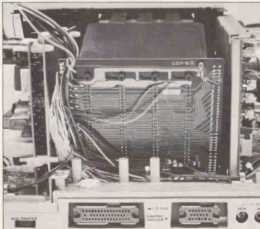
Expansion ports are on OP-1 adaptor; PCB is connector for memory modules.
