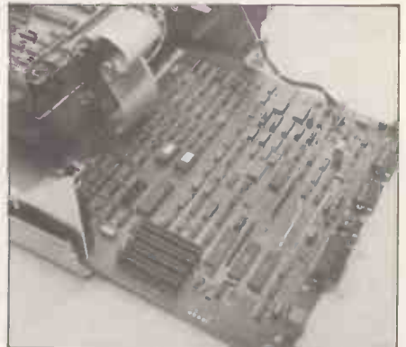
Main board contains 8088 and 128k RAM
