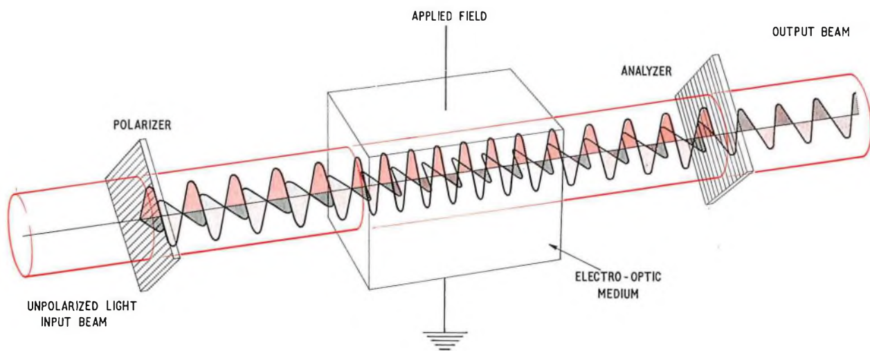
FIG. 1(a)—Electro-optic effect
