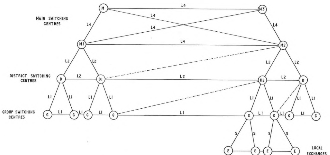
Fill-difference threshold of links L4 = 4 digits, L2 = 2 digits and L1 = 1 digit Links S form a synchronous star arrangement. The local exchanges are slaved to the parent group switching centre
