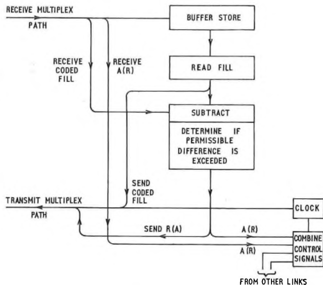
FIG. 5—Basic control system
