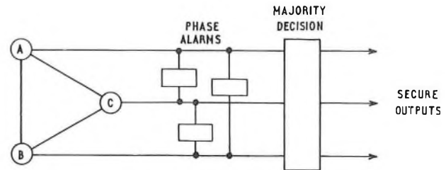
FIG. 8—Secure clock with phase alarms
