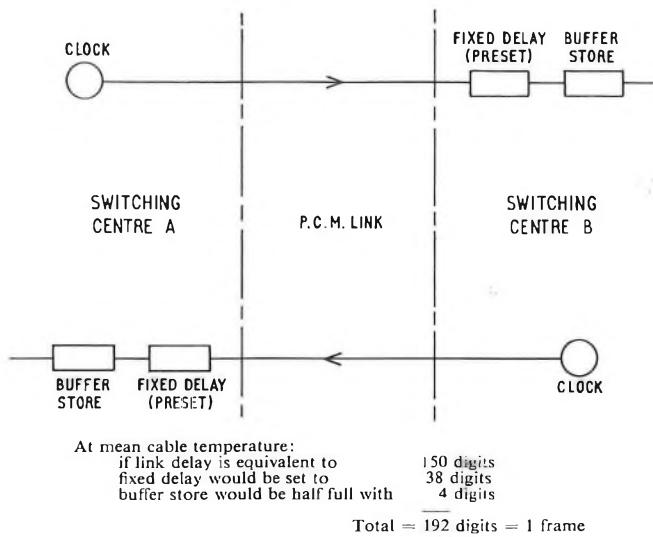
FIG. 4—Maintenance of frame delay between centres
