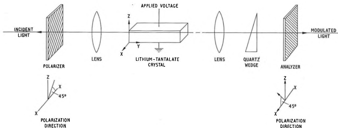
FIG. 2—Lithium tantalate modular—single transit mode
