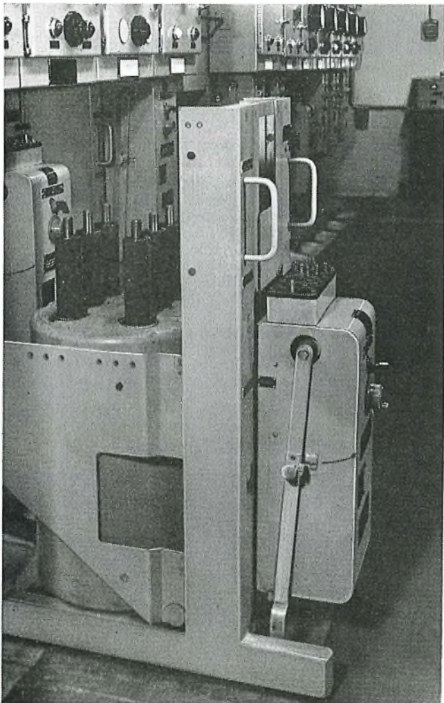
FIG. 2—An 11-kvolt oil circuit-breaker. Vertical-isolation and horizontal-withdrawal type
