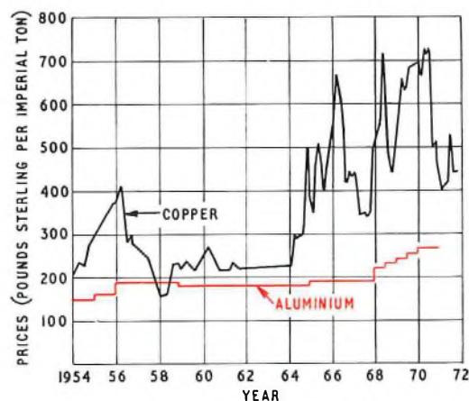
FIG. 1—Average prices of copper-wire bar and aluminium rod
