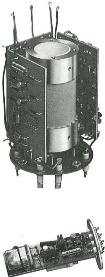
FIG. 2—Oscillator with oven and control circuits
