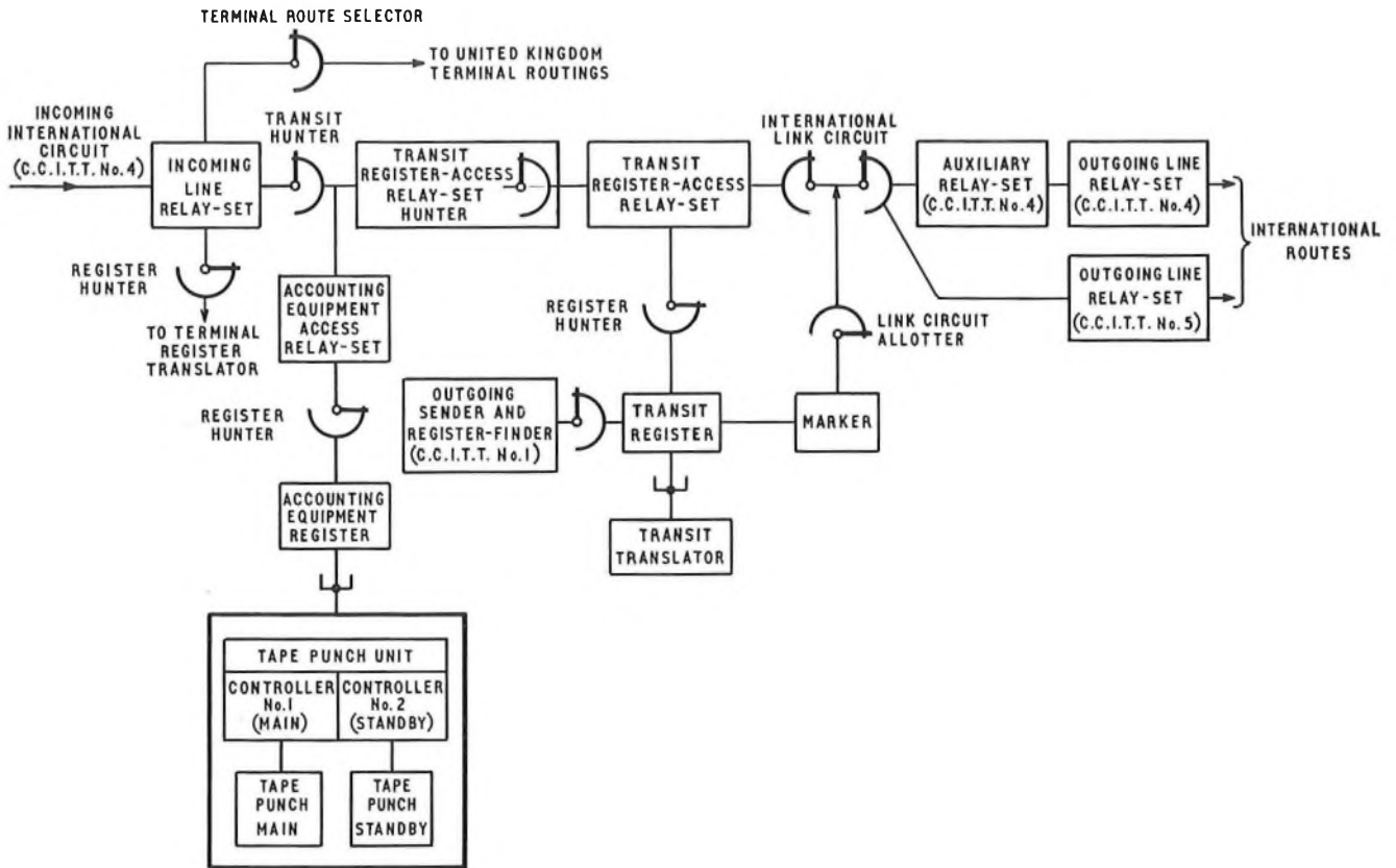
FIG. 1—Basic trunking for incoming routes using the C.C.I.T.T. No. 4 Signalling System
