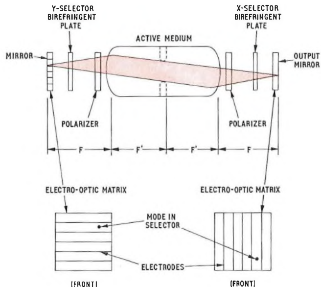
FIG. 8—Digital scanlaser with typical transverse mode illustrated
