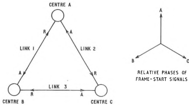
Fig. 6—Illustration of blocking in a ring of three switching centres
