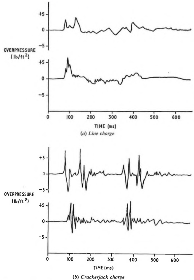
FIG. 4—Overpressure waveforms produced by simulated sonic booms
