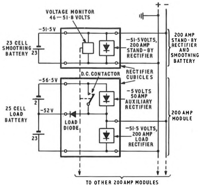
FIG. 16—Block diagram of Power Plant No. 233
