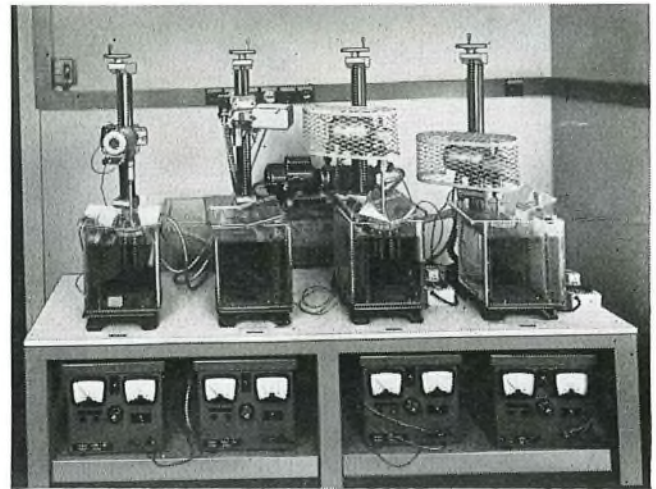
FIG. 3—Multi-vat electroforming equipment
