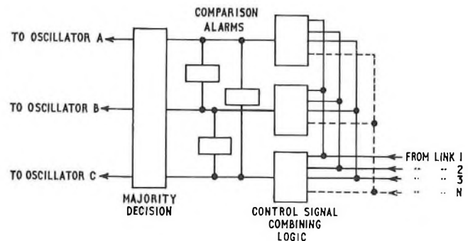
FIG. 9—Triplcation of control signal combining logic
