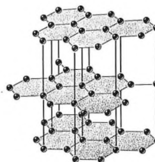
FIG. 5—Lattice of graphite showing atomic bonding within shaded planes and Van der Waals distances between planes
