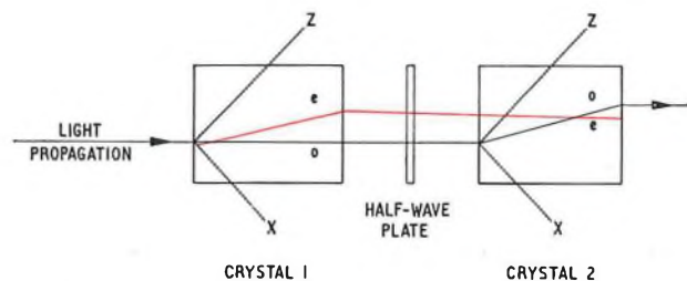
FIG. 3—A.D.P. two crystal birefringence compensation
