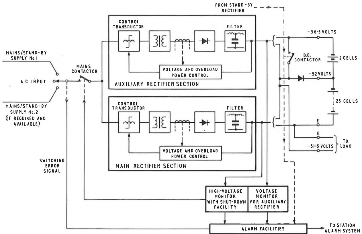
FIG. 17—Block diagram of load module
