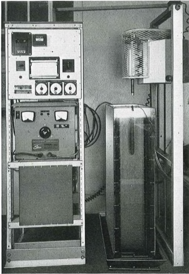
FIG. 2—Single unit electroforming equipment
