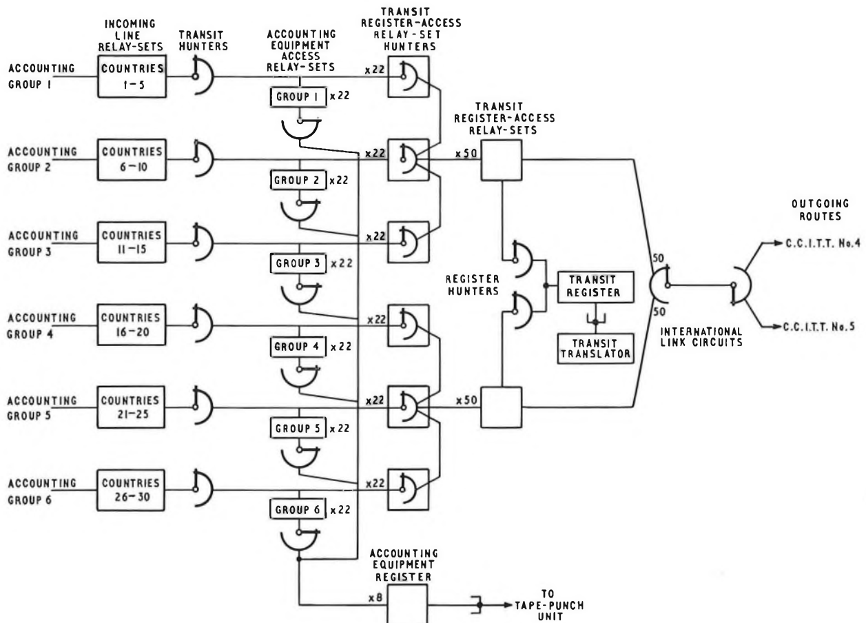
FIG. 3—Grouping of equipment for accounting purposes: incoming routes using the C.C.I.T.T. No. 4 Signalling System
