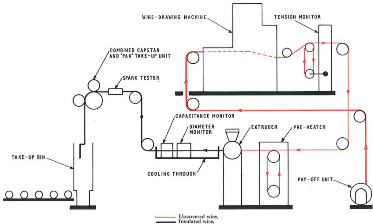
FIG. 2—Typical tandem-line layout for production of insulated aluminium conductors
