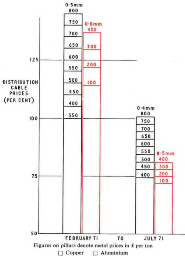
FIG. 5—Relative prices for copper- and aluminium-conductor cables for various copper and aluminium prices
