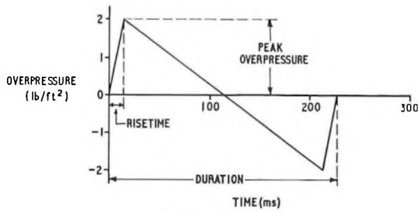
(a) Nominal N-wave
