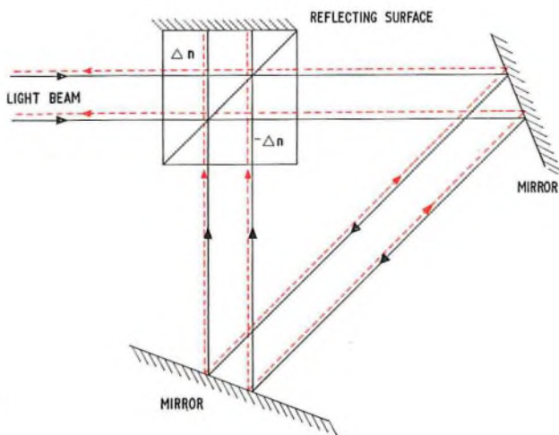
(b) Quadruple deflexion element
