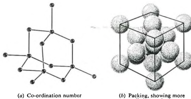
FIG. 3—Atomic lattice of diamond, silicon and germanium
