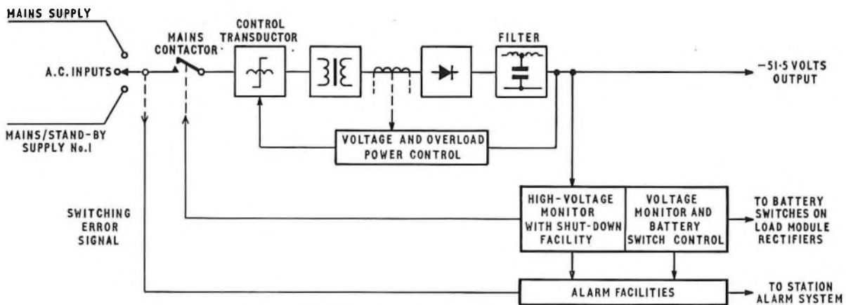
FIG. 18—Block diagram of stand-by rectifier
