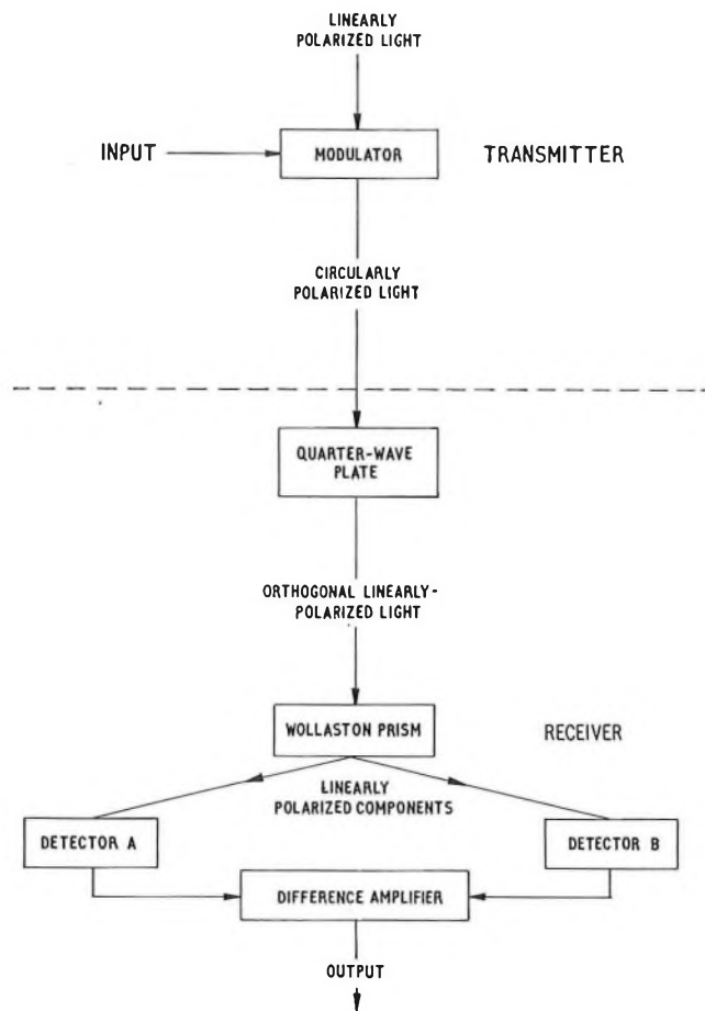
FIG. 4—Polarization modulation—demodulation transmission system
