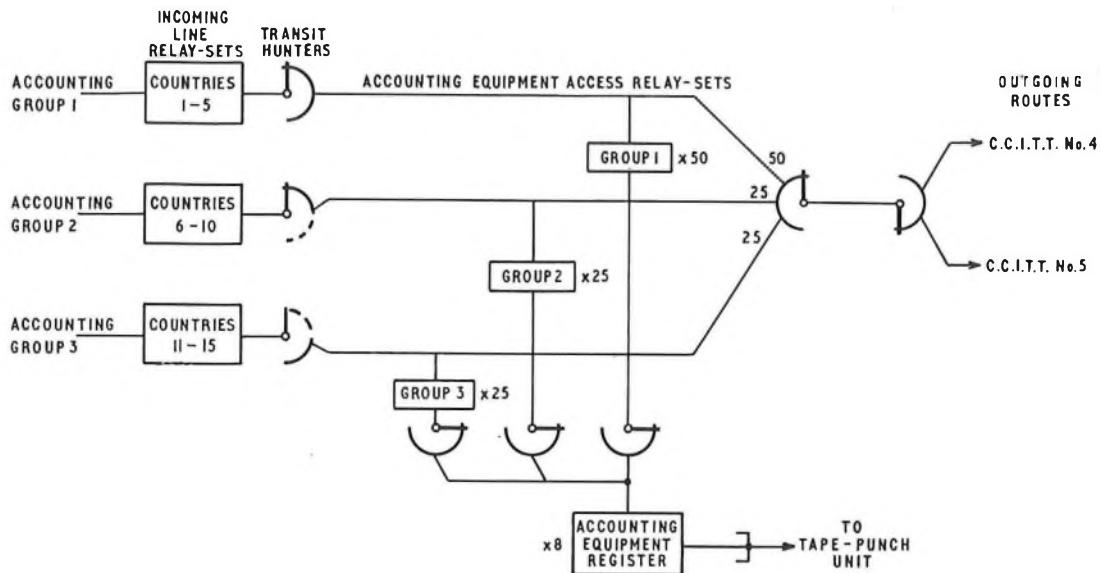
FIG. 4—Grouping of equipment for accounting purposes: incoming routes using the C.C.I.T.T. No. 5 Signalling System
