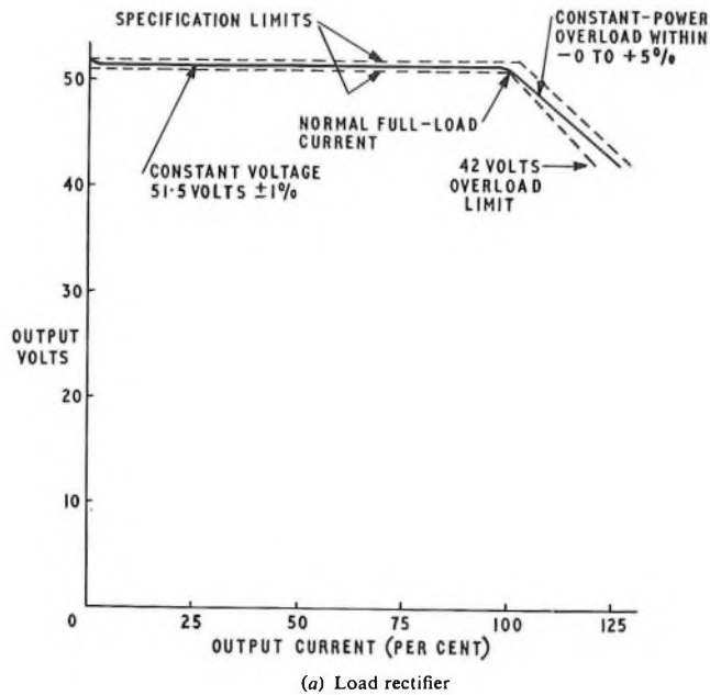
FIG. 20—Rectifier output characteristics
