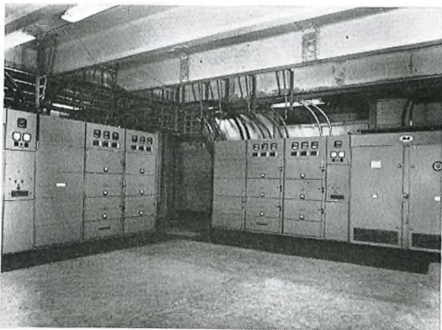
FIG. 3—Two of the 1-Mvolt-amp packaged sub-stations shown in position and on load
