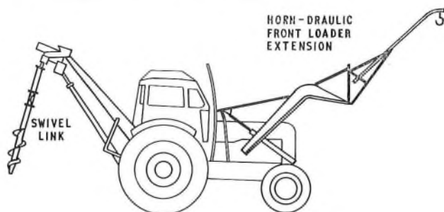
Lister post-hole borer type P.B.5
