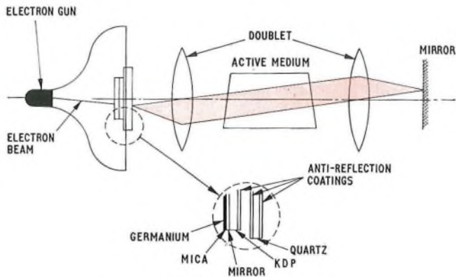
FIG. 7—Fast electron-beam scanlaser
