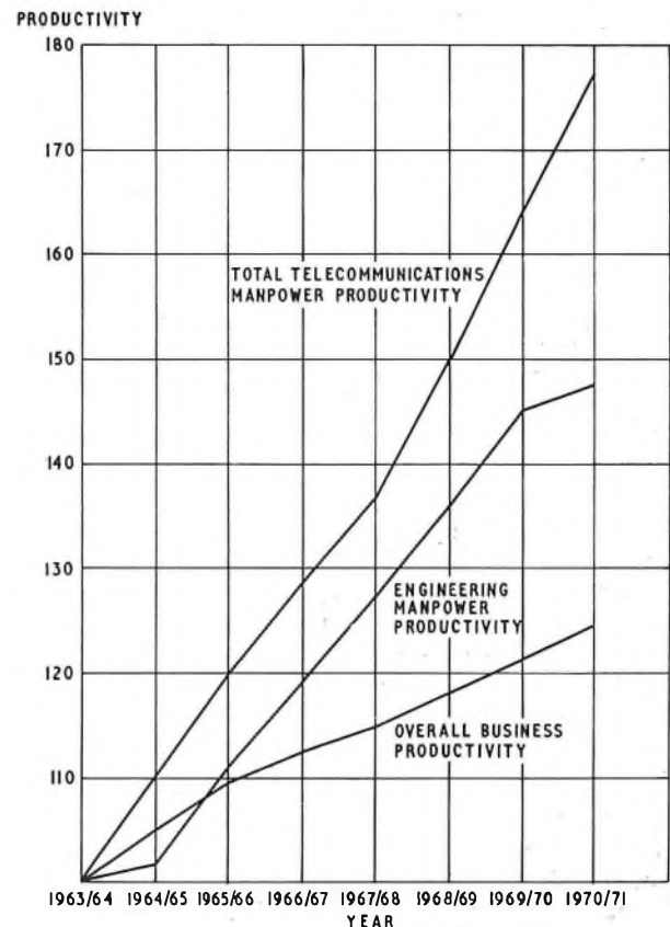
FIG. 2—Productivity improvement. (base 100 at 1963/64)
