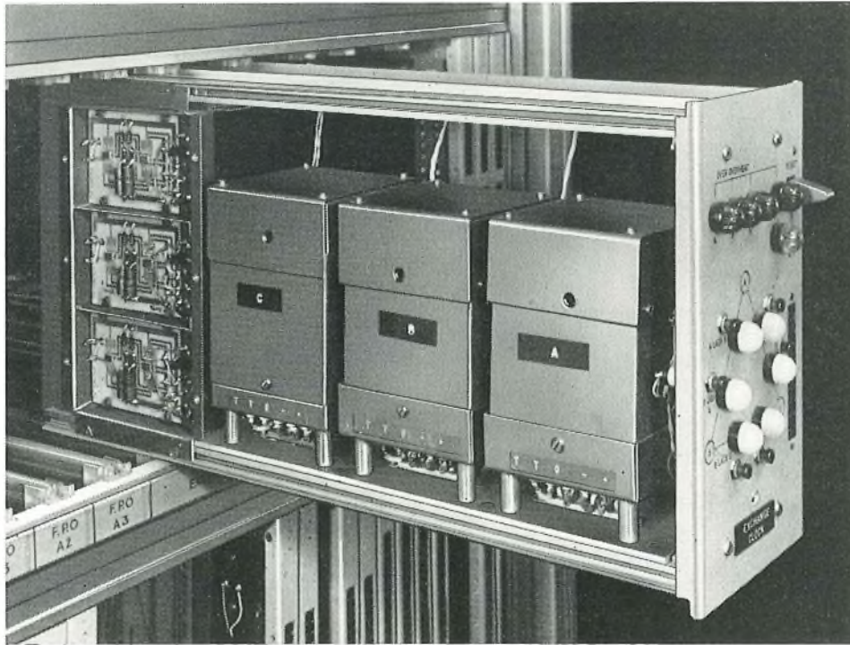
FIG. 1—Exchange clock showing oscillators and majority-decision logic circuits
