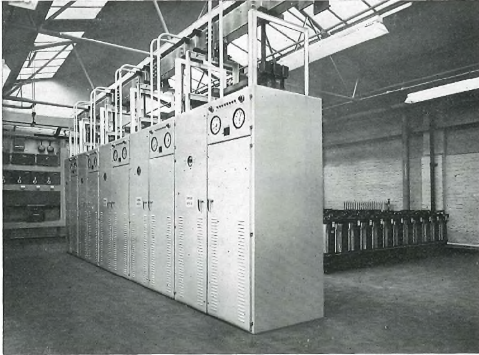
FIG. 14—Prototype installation of four 200-amp load modules and one 200-amp stand-by rectifier
