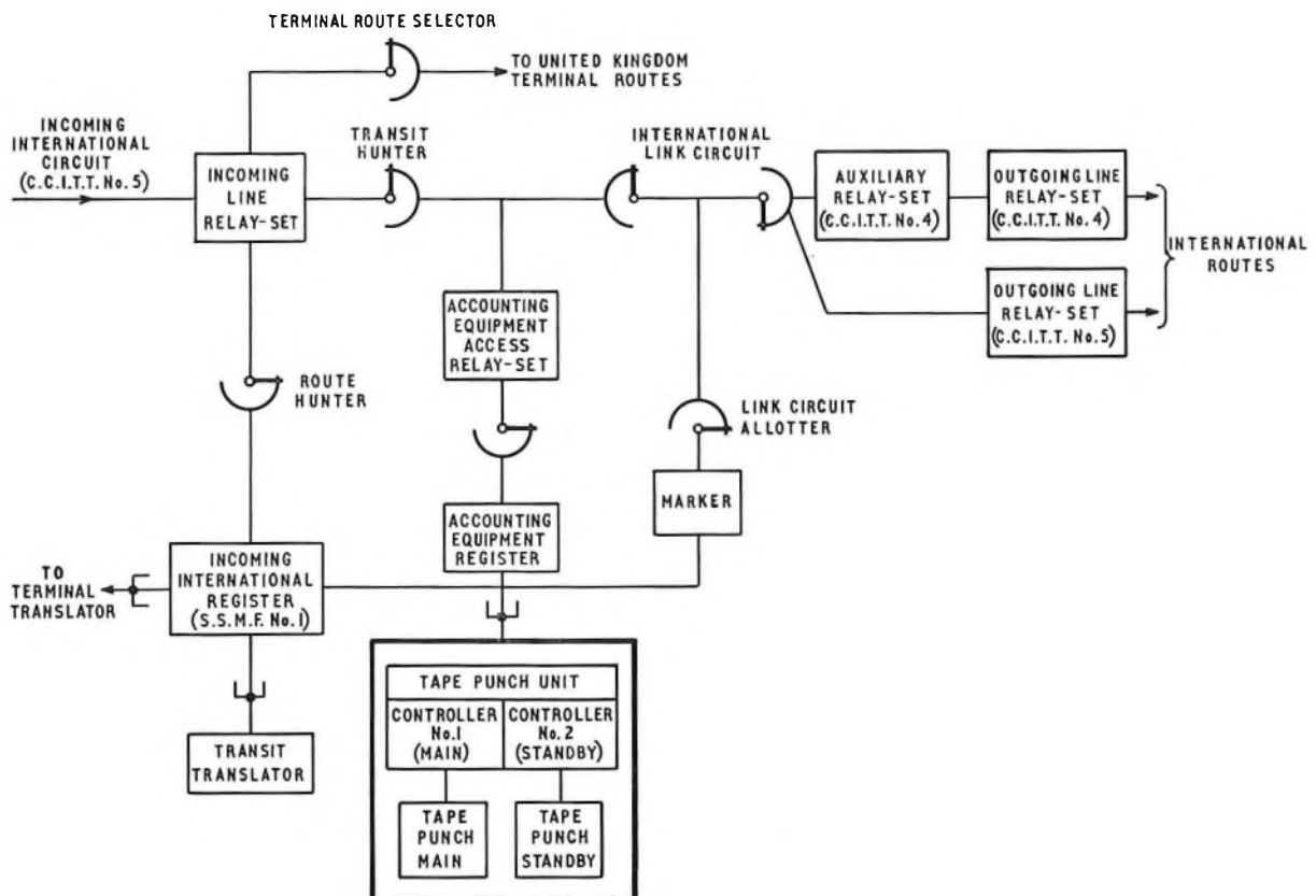
FIG. 2—Basic trunking for incoming routes using the C.C.I.T.T. No. 5 Signalling System
