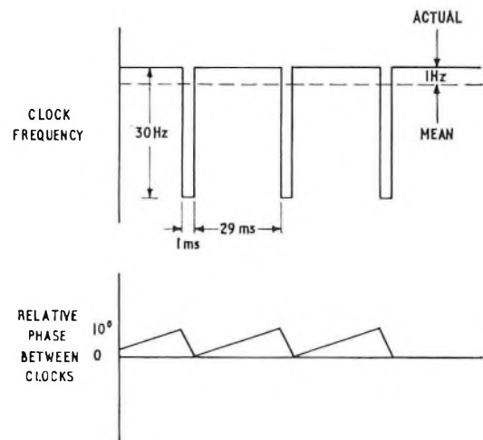
FIG. 3—Principle of clock control
