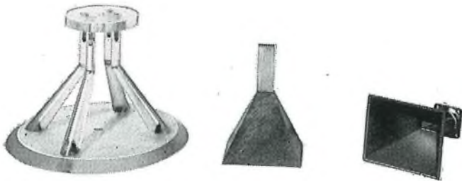
FIG. 4—Electroformed horn with master and perspex shield
