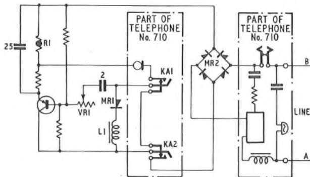
FIG. 2—AMPLIFIER CIRCUIT
