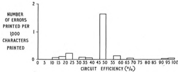
FIG. 4—UNDETECTED-ERROR RATE/CIRCUIT-EFFICIENCY CHARACTERISTIC FOR LONDON-BARBADOS-LONDON TEST
