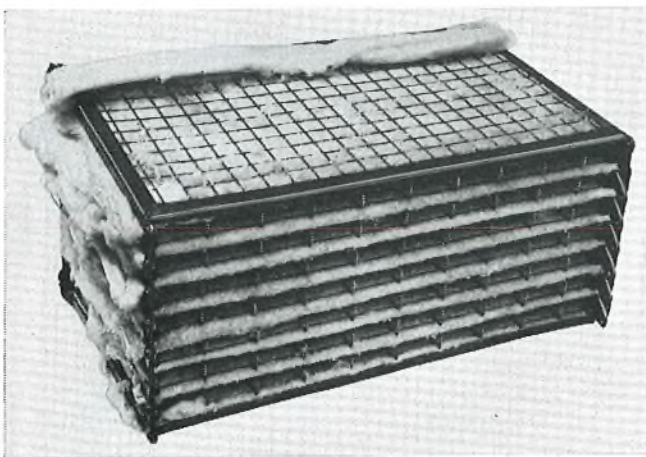
FIG. 4—"KONPAK" TYPE FILTER FRAME LOADED WITH COTTON FILTERING MATERIAL
