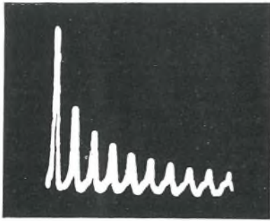
FIG. 1—TYPICAL SURGE-CURRENT CHARACTERISTIC
