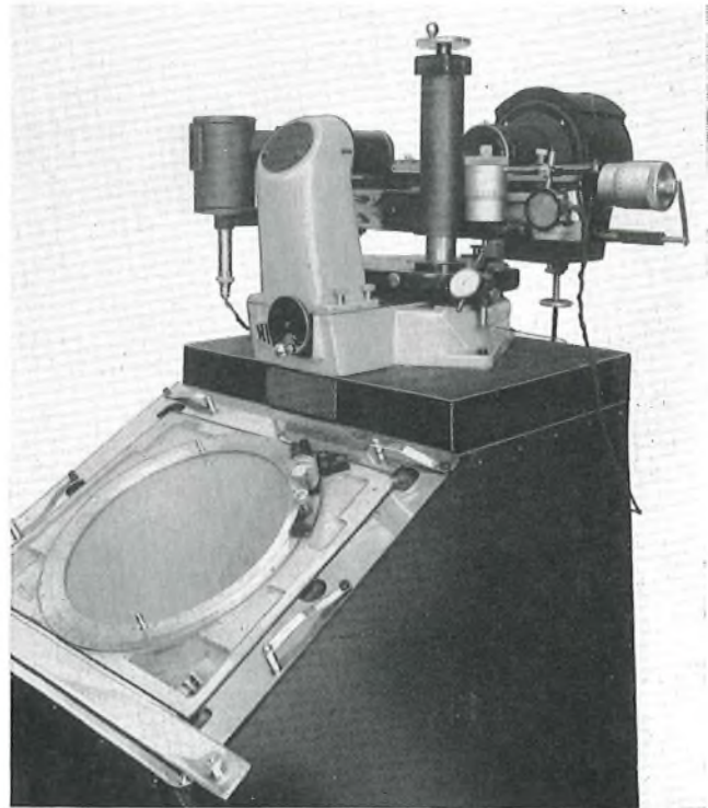
FIG. 1—UNIVERSAL PROJECTOR
