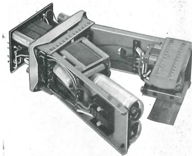
FIG. 1—TRANSISTOR AUDIO LINE AMPLIFIER (AMPLIFIER NO. 121)
