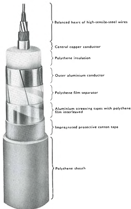
FIG. 1—LIGHT-WEIGHT SUBMARINE CABLE
