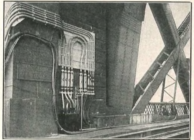
FIG. 9.—LOADING COILS AT JUBILEE ARCH.
