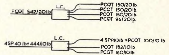
FIG. 10.—ARRANGEMENT OF AUDIO CABLES AT LOADING POINT.
