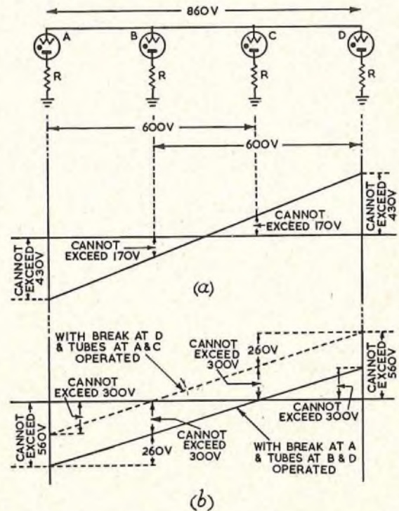
FIG. 3.—VOLTAGE DISTRIBUTION ALONG A COMMUNICATIONS WIRE FOR INDUCED VOLTAGES 600-860V.
