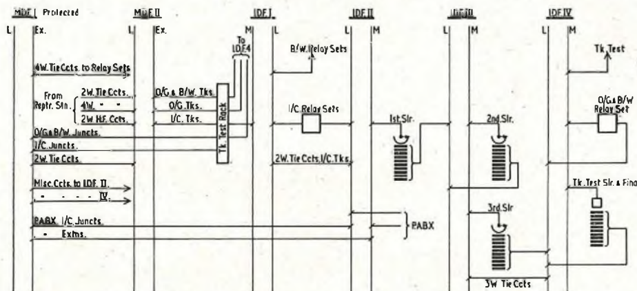
FIG. 4.—MAIN CABLING SCHEME.
