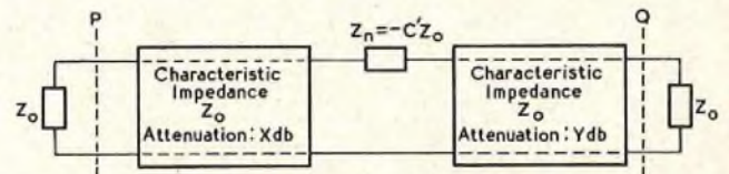
FIG. 9.—INSERTION OF A SERIES-CONNECTED NEGATIVE IMPEDANCE IN A TWO-WIRE TRANSMISSION CIRCUIT (PQ) TERMINATED WITH ITS CHARACTERISTIC IMPEDANCE.
