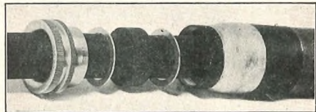
FIG. 14.—EXPLODED VIEW OF SEALING GLAND.
