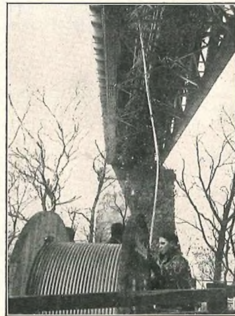
FIG. 6.—CABLING ON THE SOUTHERN APPROACH TO THE BRIDGE.
