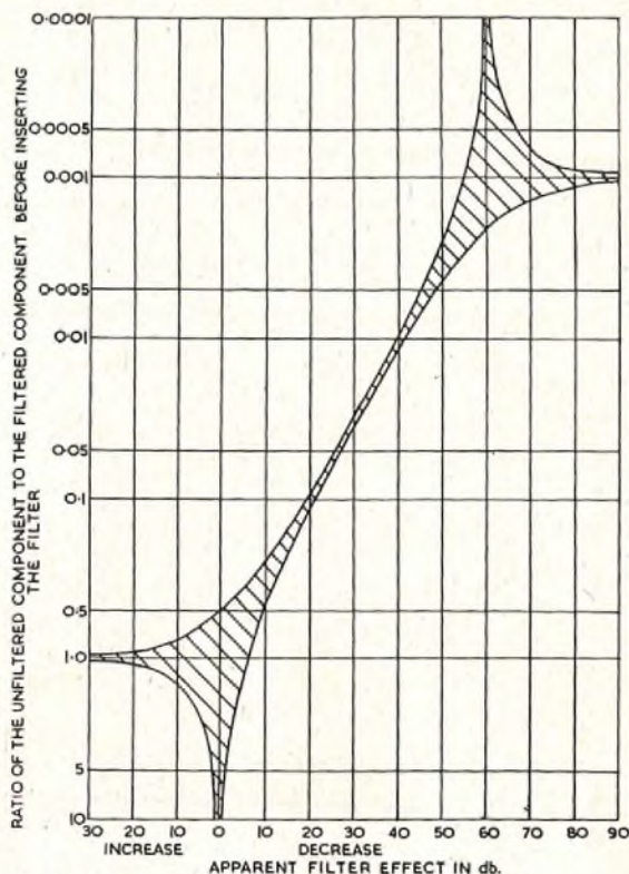
FIG. 6.—APPARENT EFFECT ON SITE OF A FILTER HAVING A DISCRIMINATION OF 60 DB.
