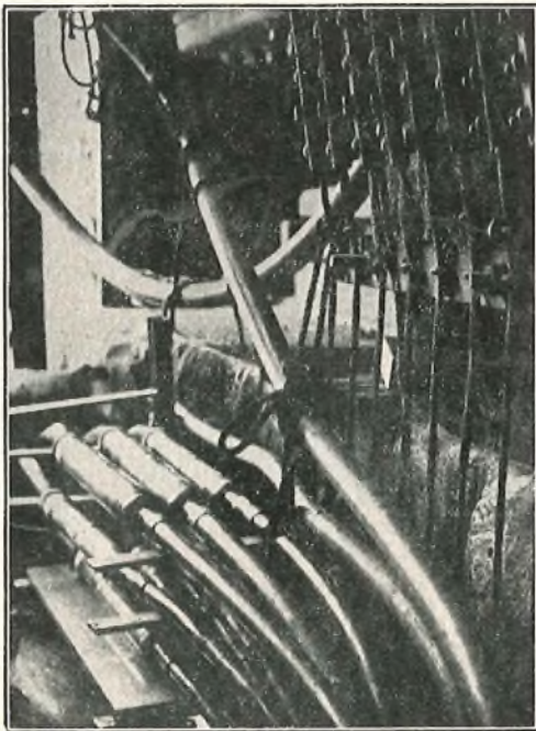
FIG. 16.—JOINTING PLATFORM AND SUSPENSION WIRE TERMINATIONS ON NORTH PIER.
