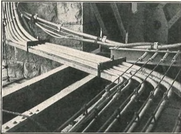
FIG. 8.—CABLES LEAVING SUSPENSION WIRES AT JUBILEE ARCH.
