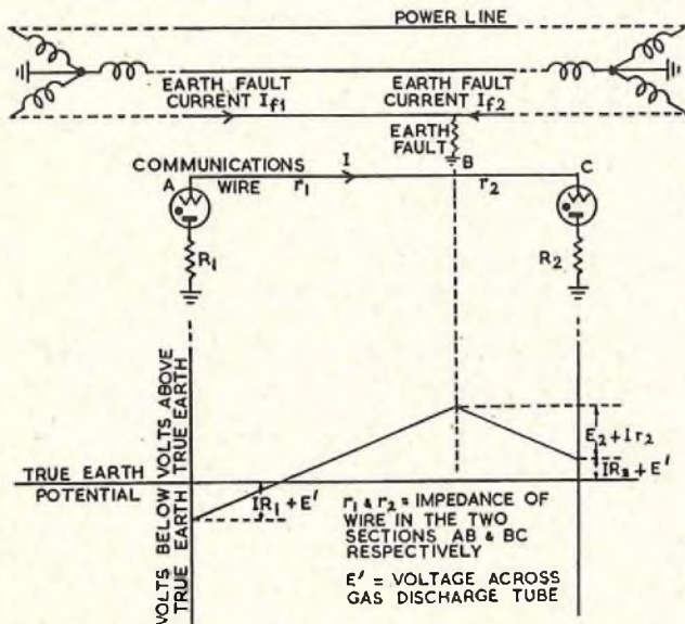
FIG. 2.—VOLTAGE DISTRIBUTION ALONG COMMUNICATIONS WIRE WITH A POWER LINE EARTH FAULT AT AN INTERMEDIATE POINT IN THE EXPOSURE.
