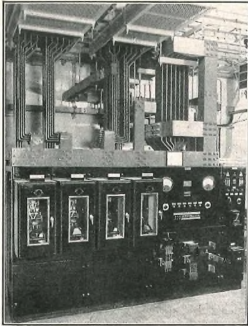
FIG. 8.—POWER-DISTRIBUTION BOARD.
