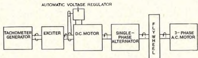
FIG. 1.—BLOCK SCHEMATIC DIAGRAM OF NEW TELEGRAPH POWER PLANT.
