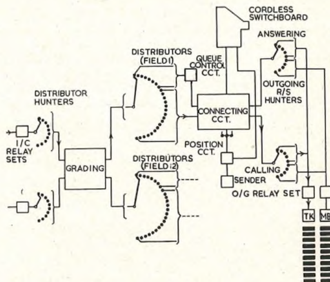
Fig. 2.—TRUNKING PRINCIPLES OF CORDLESS SWITCHBOARD.
