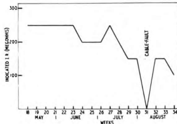
FIG. 9.—INDICATOR READINGS (WEEKLY) AT COLWYN BAY R.S. ON COLWYN BAY-HOLYHEAD CABLE (88 WIRE-MILES).
