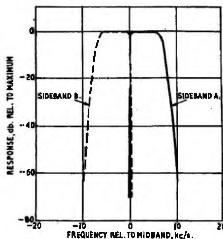
FIG. 7.—OVERALL SELECTIVITY CHARACTERISTIC (UP TO DEMODULATOR INPUT).
