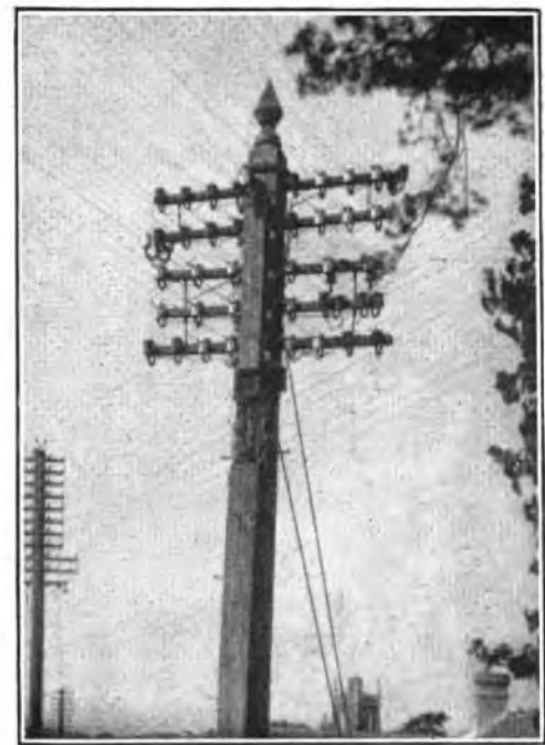
PITCH-PINE SQUARE-SECTION POLE.
