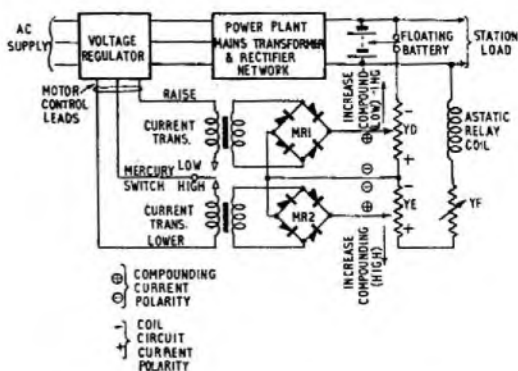
FIG. 3.—CIRCUIT OF D.C. ASTATIC RELAY.
