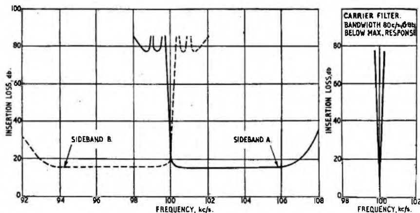
FIG. 8.—CHARACTERISTICS OF SIDEBAND AND CARRIER FILTERS.
