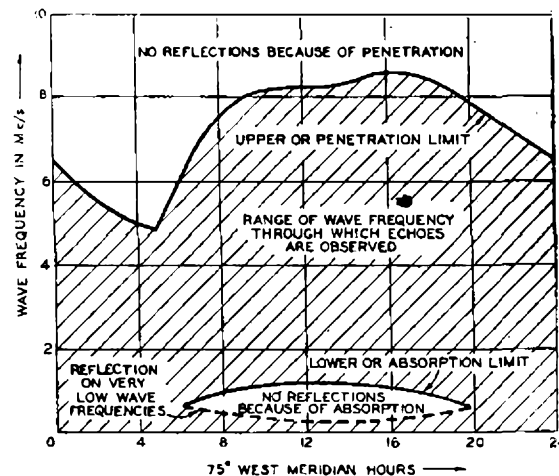
FIG. 1.—WAVE FREQUENCY BOUNDARIES GIVING REFLECTION LIMITATION DURING NORMAL CONDITIONS FOR SIX CONTROL-DAYS NEAR DAY OF FADE-OUT OF 31-7-1937.
