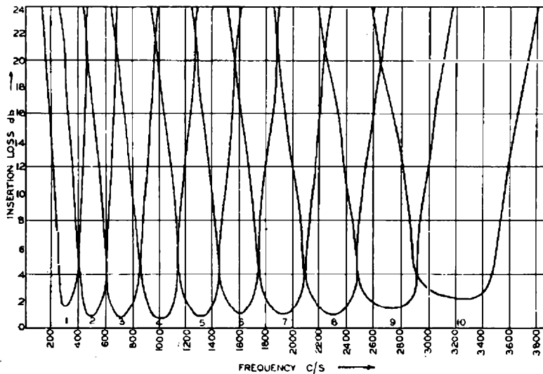
FIG. 5.—INSERTION-LOSS CURVES OF THE SPECTRUM FILTERS.
