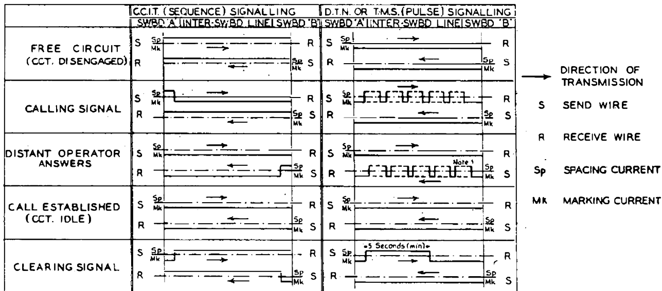
FIG. 1.—BASIC SIGNALLING CONDITIONS—SEQUENCE AND PULSE SIGNALLING SYSTEMS.
