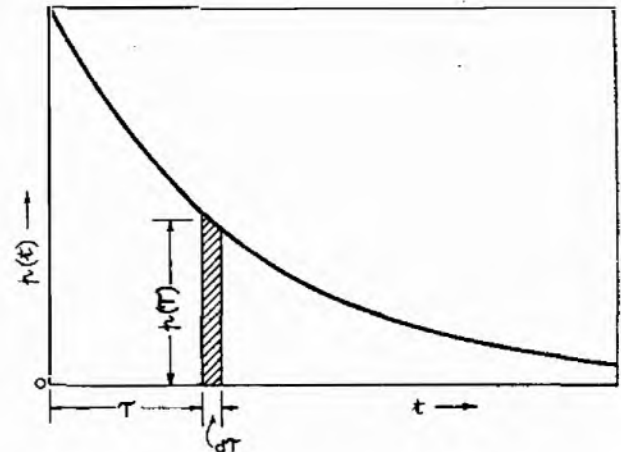
FIG. 2.—EXPONENTIAL DISTRIBUTION.
