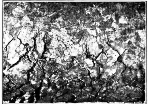
FIG. 2.—FATIGUE CRACKS DUE TO LARGE CRYSTALS (MAG. \times 5 ).
