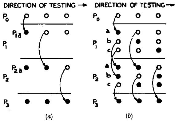
FIG. 2.—ARRIVAL OF CALLS CAUSING THE CONDITION OF A GROUP TO CHANGE.
