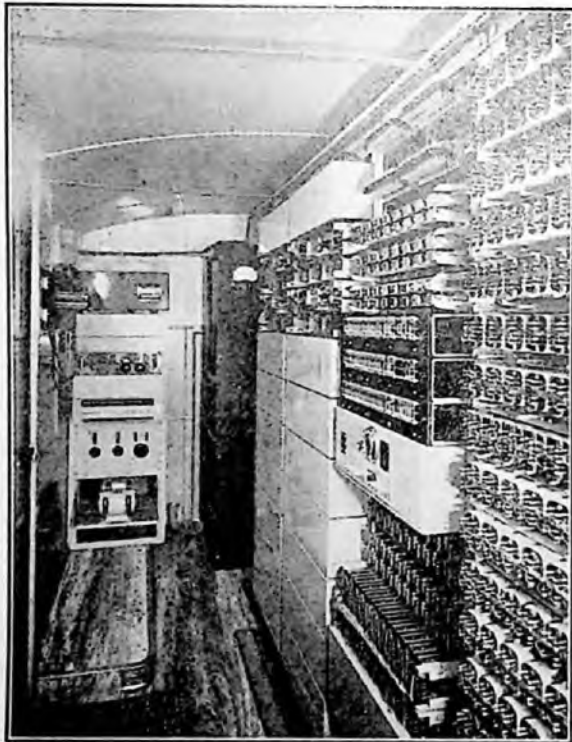
FIG. 2.—EQUIPMENT IN MOBILE REPEATER STATION.
