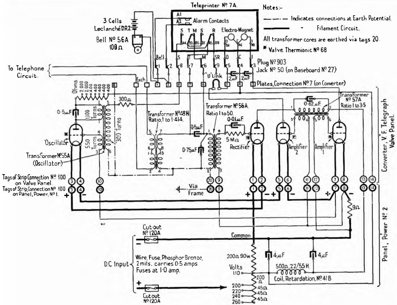
FIG. 5.—CONVERTER WITH D.C. SUPPLY.
