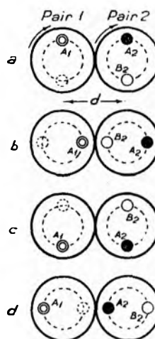
FIG. 2.—THE GEOMETRY OF WIRES IN ADJACENT QUADS HAVING EQUAL PITCHES (PAIRS PARALLEL).
