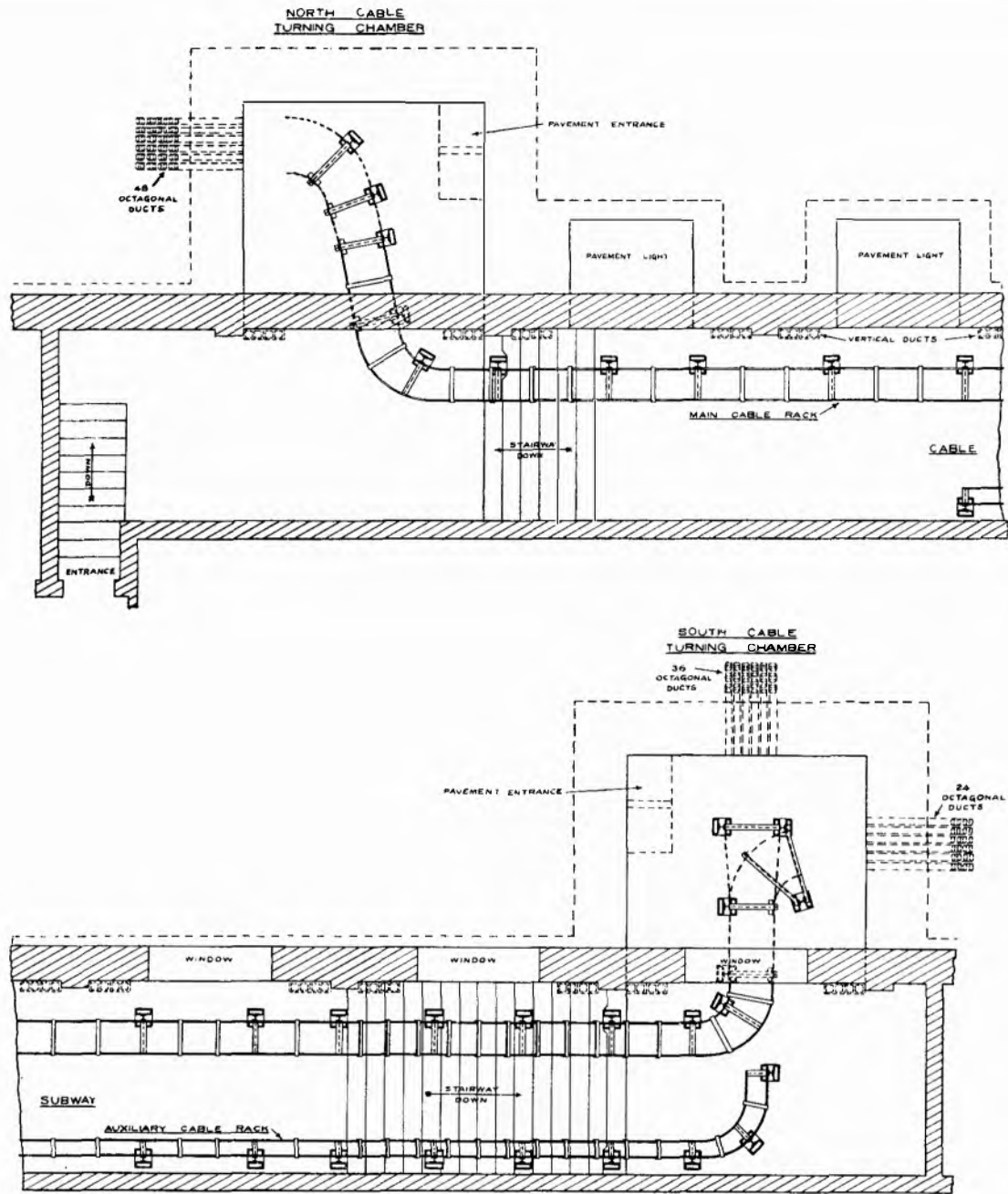
FIG. 9.—PLAN OF NEWCASTLE CENTRAL AUTOMATIC EXCHANGE CABLE SUBWAY, SHOWING CABLE RACK.
