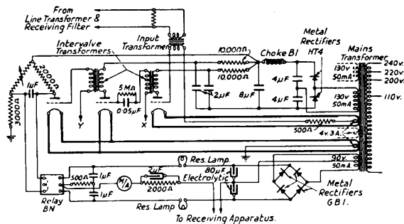
FIG. 5.—RECEIVER AND POWER ARRANGEMENT. (A.C.).
