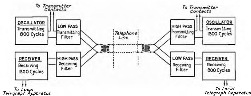
FIG. 1.—SCHEMATIC LAY-OUT.
