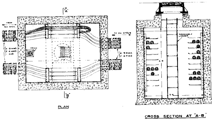
FIG. 1.—SIMPLE MANHOLE ACCOMMODATING 49 DUCTS, WITH ENTRANCE IN CENTRE AND CABLE JOINTS SUPPORTED UPON SIDE WALLS, CORNER OF CARLIOL SQUARE AND WORSWICK STREET, NEWCASTLE-ON-TYNE.
