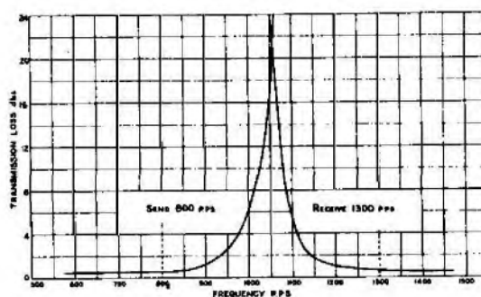
FIG. 6.—FILTER ATTENUATION-FREQUENCY CURVE.
