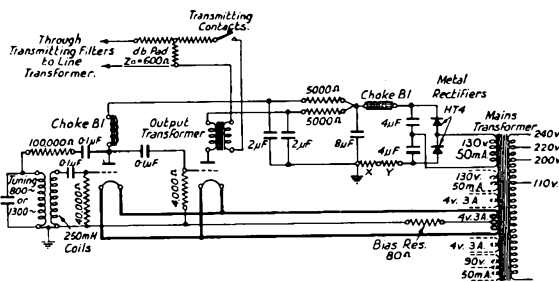
FIG. 4.—OSCILLATOR AND POWER ARRANGEMENT. (A.C.).
