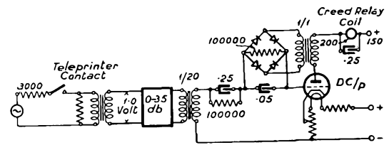
FIG. 3.—SINGLE-VALVE RECEIVER.
