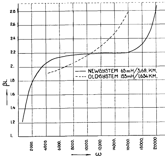
FIG. 2.—ATTENUATION CURVE.
