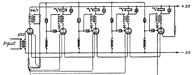
FIG. 4.—FOUR-FREQUENCY VALVE RECEIVING SET FOR KEYSENDING FROM A-POSITIONS.
