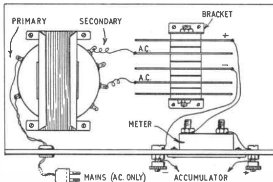
Fig. 2—Complete wiring plan
