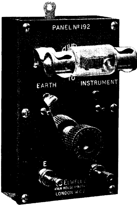
AERIAL-EARTH SWITCH Fig. 1. The lightning arrester is not permanently fixed in the Elwell earth switch, but is held by clips which are also conductors
