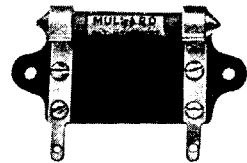
Grid Leak with Fixed Condenser
