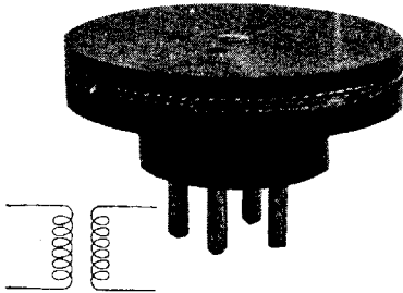
High-frequency transformer
