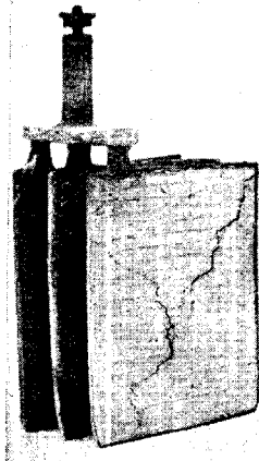
ACCUMULATOR PLATES Assembly of three negative plates suitable for a portable accumulator
