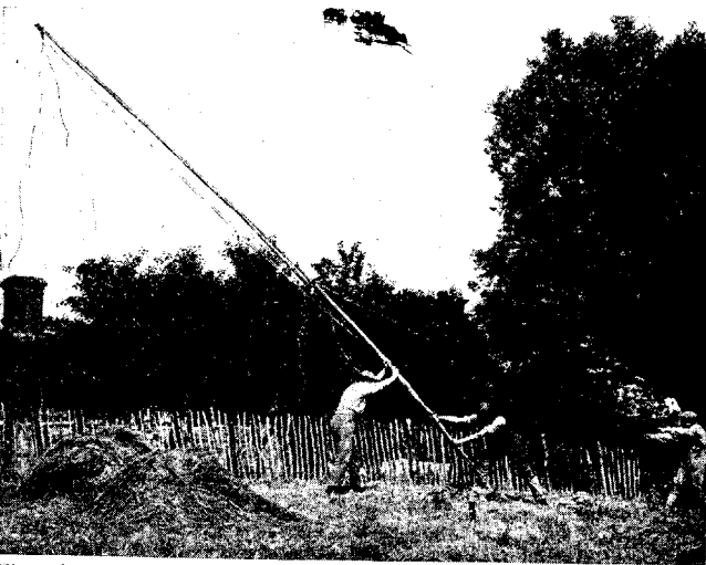
Fig. 28. Guy ropes being used as aids during erection of the two-part aerial mast
