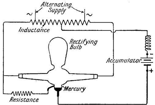
Fig. 15. Showing position of the inductance coil, which furnishes the negative charging terminal and is connected direct across the alternating mains. The mercury vapour bulb acts as a rectifier, and is connected to the positive terminal
