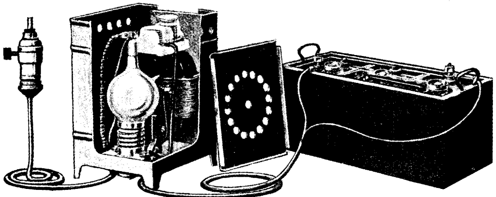
Fig. 16. A bulb filled with argon gas contains a low-voltage tungsten filament and a graphite electrode. A transformer and reactance are also included in the circuit, which operates in a manner similar to the action of the ordinary thermionic detecting valve
