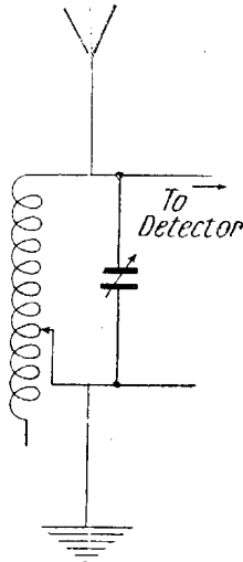
The simplest aerial system
