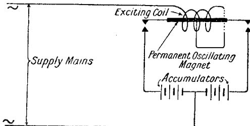
Fig. 13. A mechanical rectifier converts the alternating current to direct current. Resistance control of the charging rate will also be required
