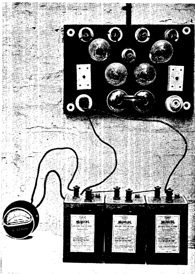
ACCUMULATOR CHARGING BOARD IN USE
