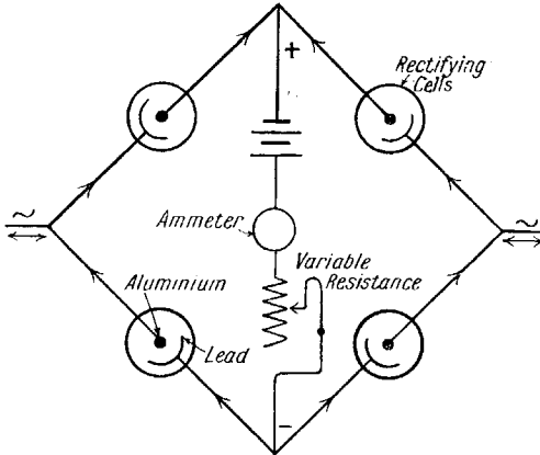
Fig. 14. The Noden valve method, showing the four cells coupled. The arrows indicate the direction of the current, the A.C. supply being seen at the right and left terminals, and rectified D.C. charging current at top and bottom
