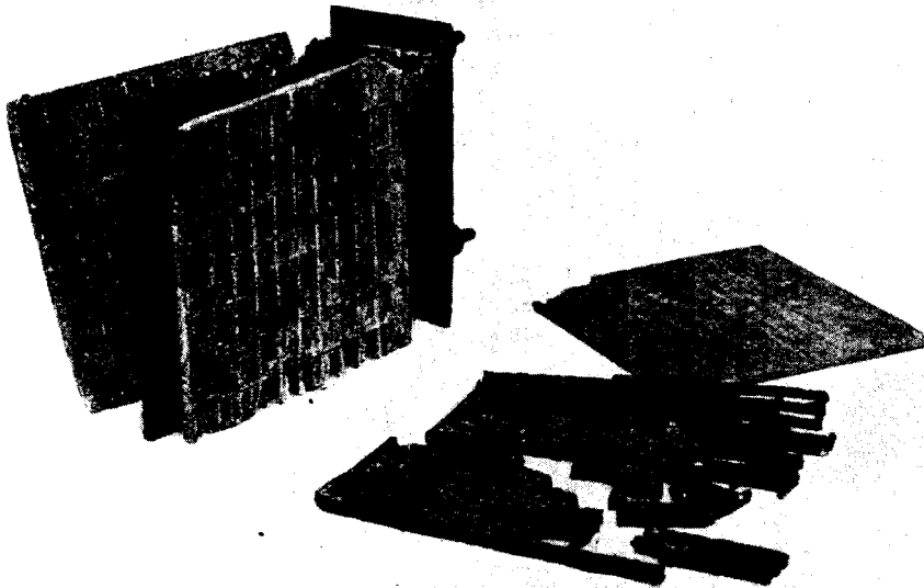
Fig. 23. What happens when an accumulator is allowed to deteriorate by neglect is shown in this example. The terminal has parted from one plate, and the paste filling has fallen away in a number of cases. The plates are beyond practical repair and should be replaced
