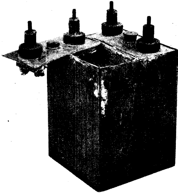
Fig. 19. Top of a cell partly removed during repair of a 4-volt accumulator, showing broken lug
