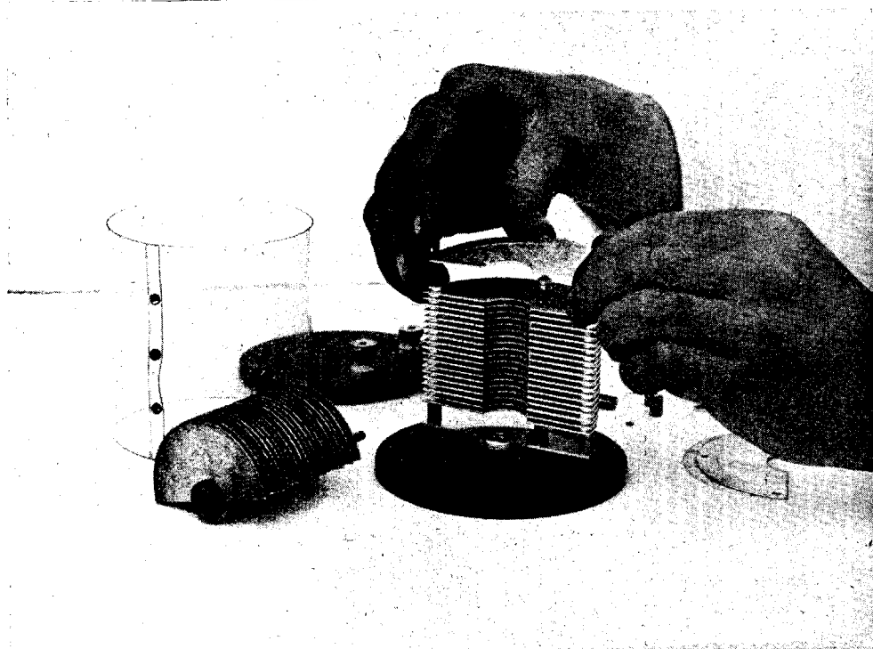
ASSEMBLING THE FIXED PLATES OF A CONDENSER
