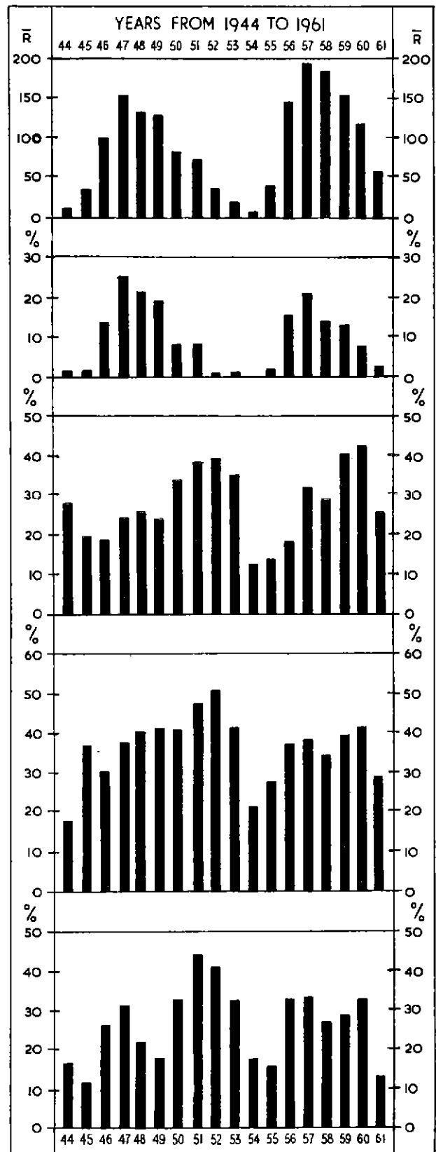
Fig. 5 — Variations of propagational disturbances in southern England with solar activity. Sunspot cycles Nos. 18 and 19 (1944-61).
