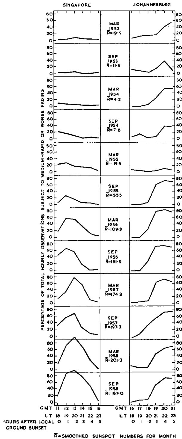
Fig. 3 — Incidence of medium-rapid or worse fading during the period 0 to 5 hours after ground sunset during equinoctial months 1953–8.
