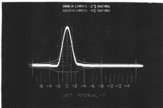
(b 1 ) 2T pulse. Test gear only (2 per cent).
