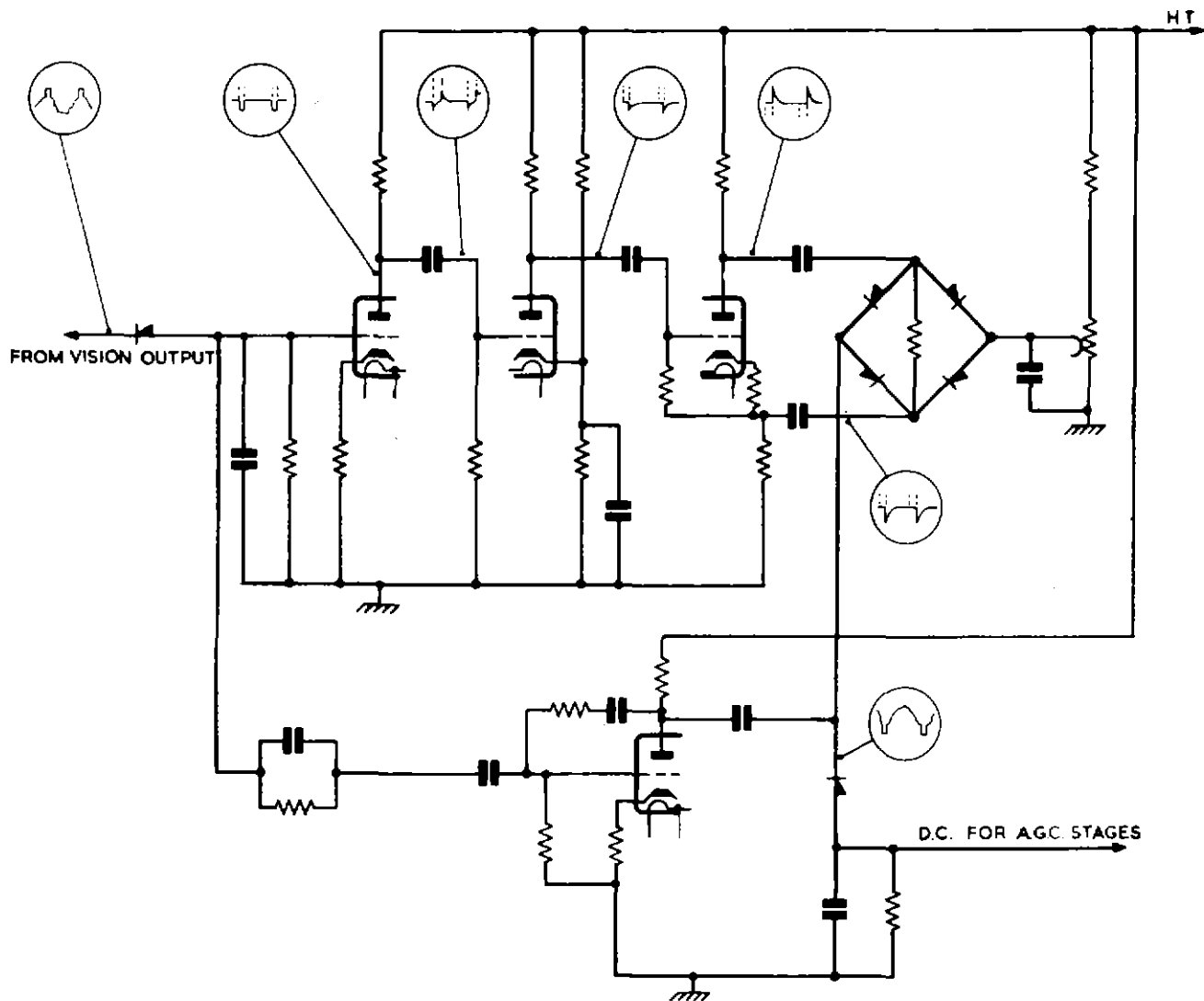
Fig. 7 — Vision A.G.C. circuit.
