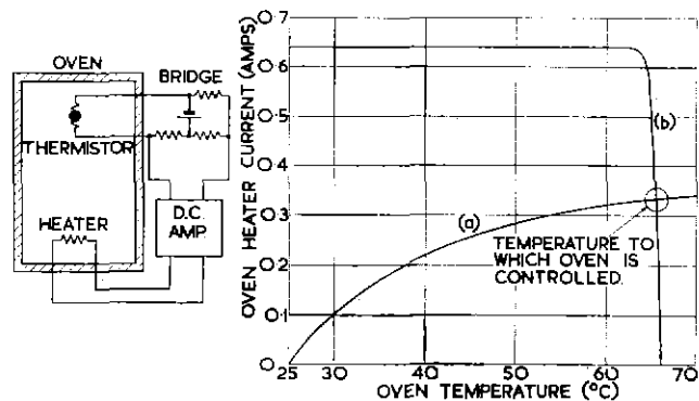
Fig. 6 — Crystal control oven. (a) Current required to maintain oven with an external temperature of 25°C. (b) Heater current output from amplifier and bridge circuit.
