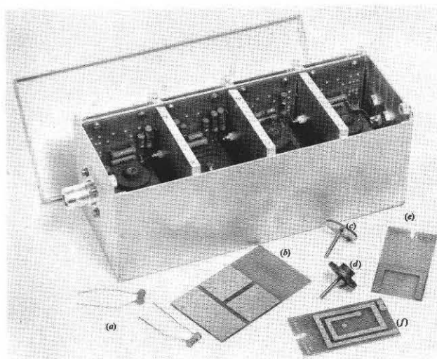
Fig. 5 — Translator R.F. filter and principal components.
