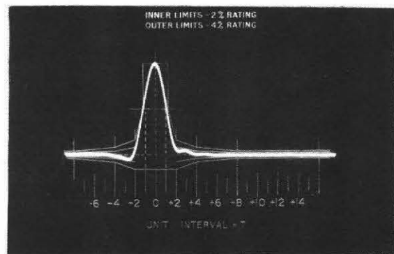
(b 2 ) 2T pulse. Translator and test gear (2 per cent).
