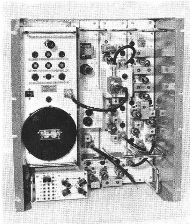
Fig. 14 — Drive equipment for modulating one FM channel from an audio signal. The basic 2·6 Mc/s drive (see Sec. 5.3.1.) is in the oven on the left, and the two small crystal ovens on the other panels form part of a two-stage frequency-changing system.
