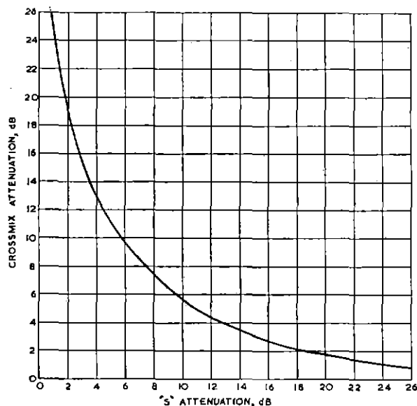
Fig. 4 — Relationship between cross-mix attenuation and 'S' attenuation to give the same scale of width
