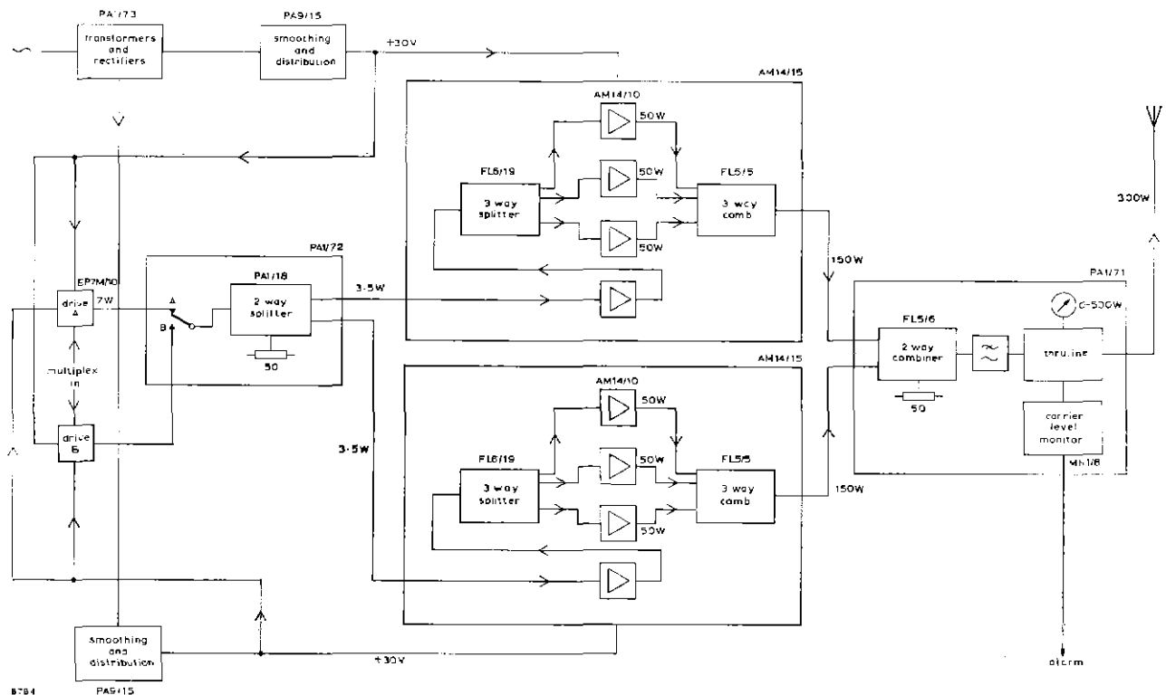
Fig. 4 Block diagram of low-power transmitter
