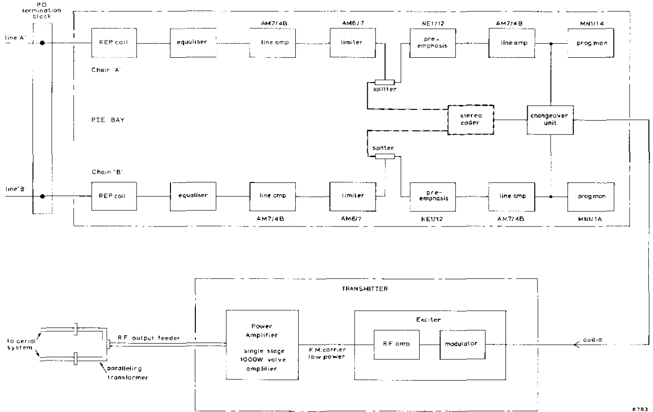
Fig. 3 Block diagram of 1-kW transmitter
