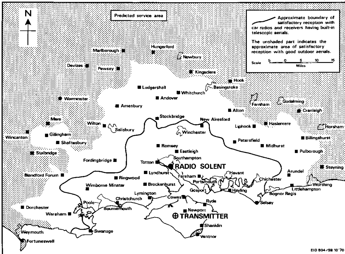
Fig. 16 Radio Solent coverage map. The solid line is the 60 dB ( \mu\text{V}/\text{m} ) contour. The limit of the unshaded area indicates the 48 dB ( \mu\text{V}/\text{m} ) contour
