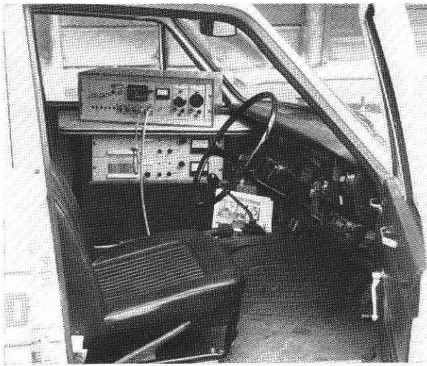
Fig. 11 Equipment in the radio car. The three units on the left of the driver's seat are: Upper: Microphone amplifiers, p.p.m., and input selector Middle: U.H.F. transmitter for programme link Lower: U.H.F. receiver for radio microphone
