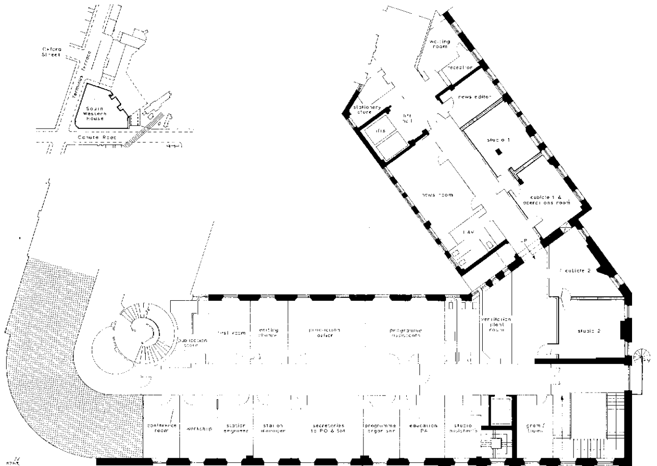
Fig. 17 Radio Solent: floor plan of studio premises
