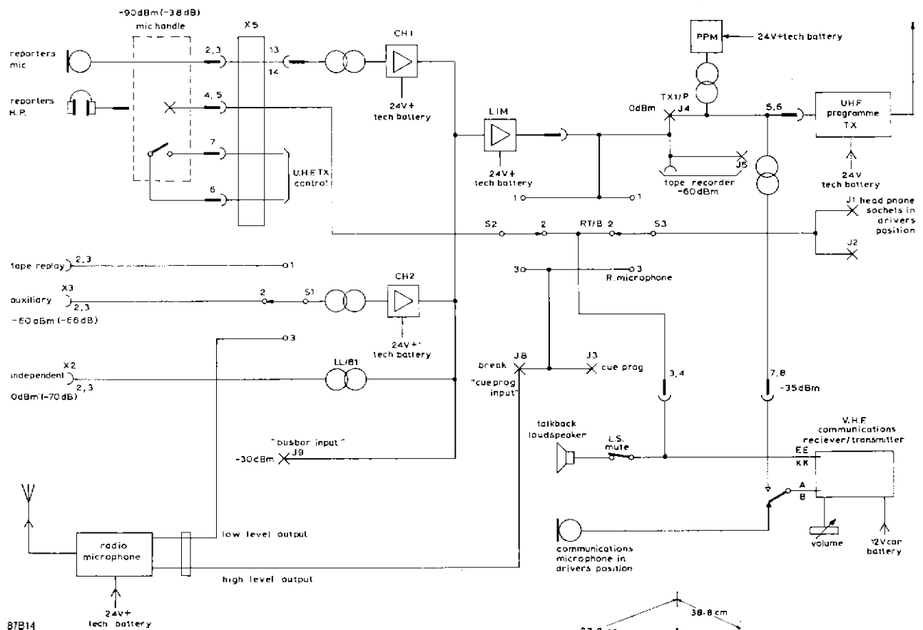
87B14 Fig. 14 Block diagram of radio-car audio circuits
