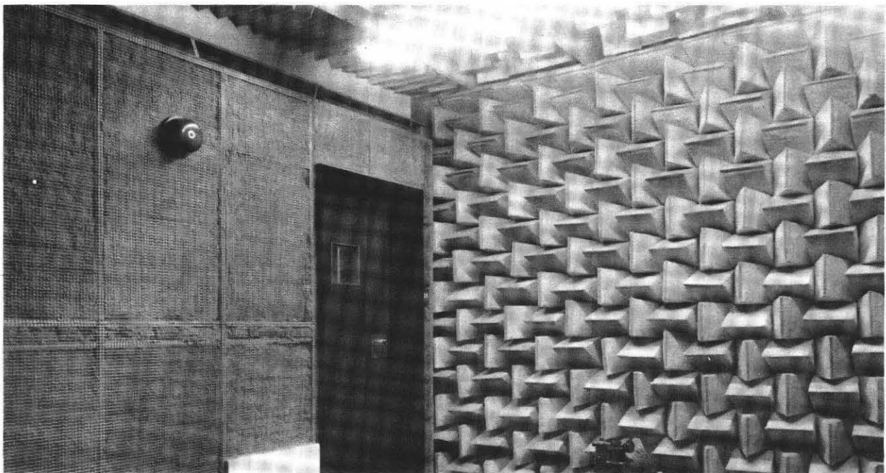
Fig. 6 Acoustic treatment of the dead room adjacent to studio 3
