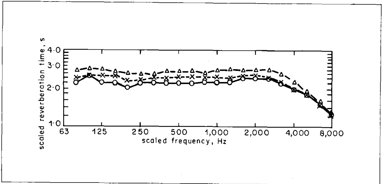
Fig. 11 Reverberation time/frequency curves for proposed Manchester music studio. Height 12 metres.
