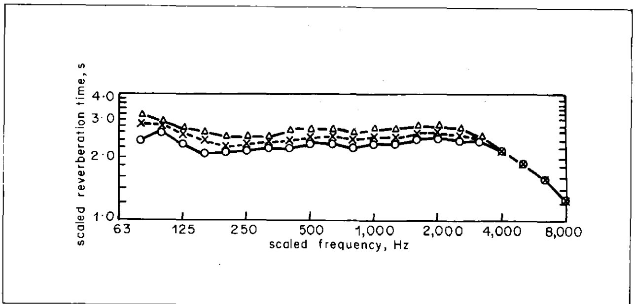
Fig. 12 Reverberation time/frequency curves for proposed Manchester music studio. Height 14 metres.
