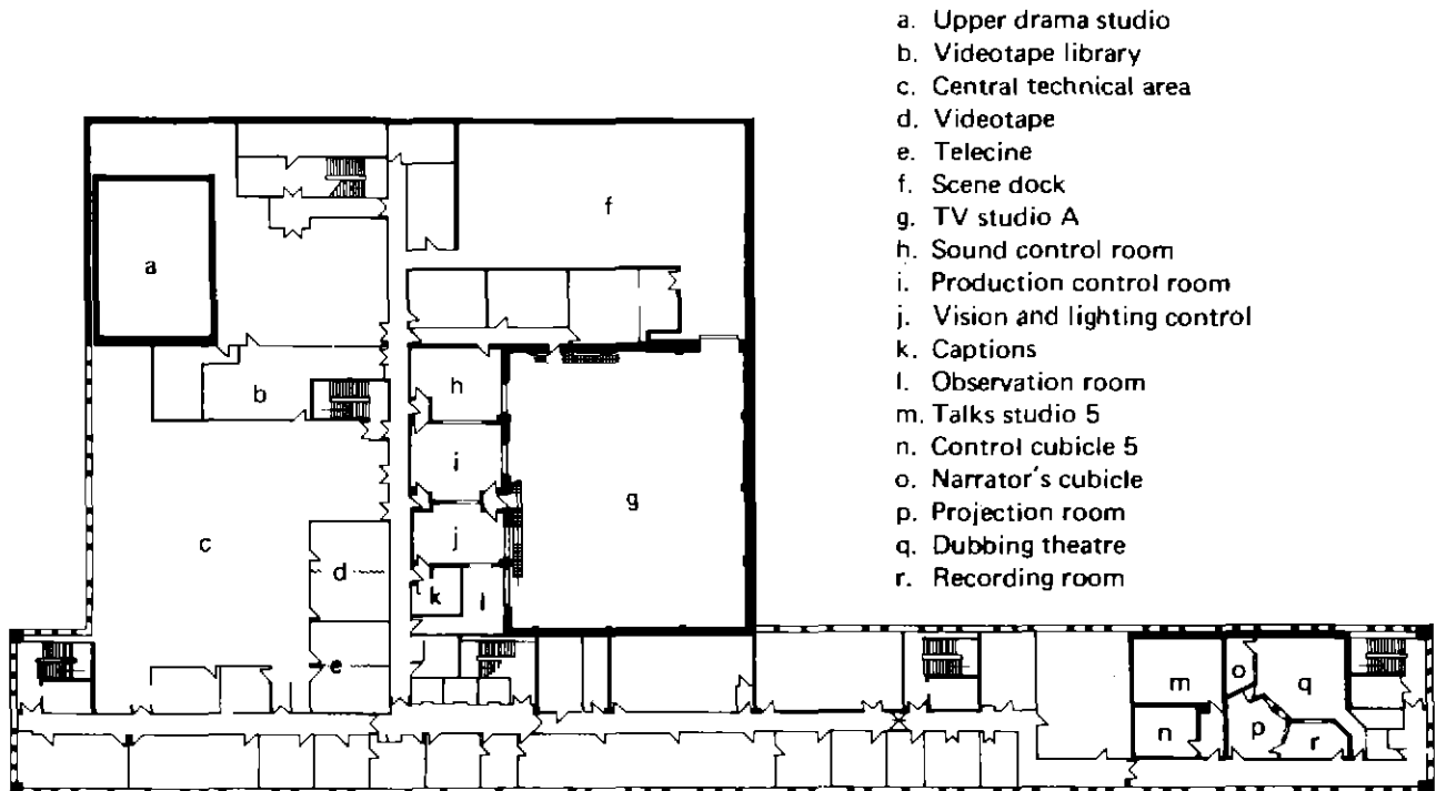
Fig. 3 First-floor plan showing the most significant areas
