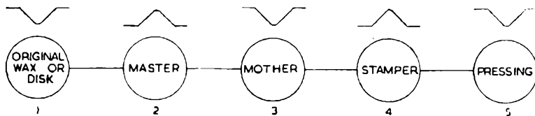
FIG. 99. FULL-PROCESS STAGES
