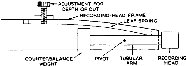
FIG. 41. PORTABLE RECORDING MACHINE TYPE C: RECORDING-HEAD FRAME
