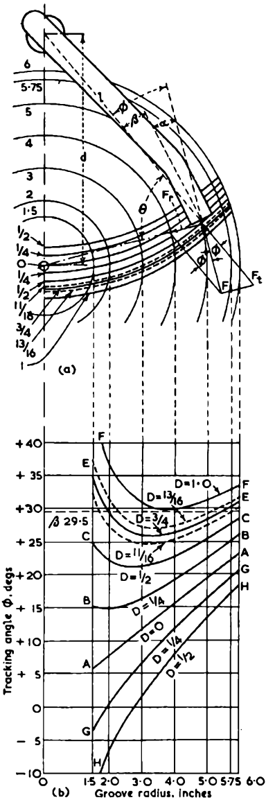
FIG. 11. DIAGRAM SHOWING DIMENSIONS AND ANGLES INVOLVED IN TONE ARM DESIGN, AND CURVES SHOWING HOW TRACKING ANGLE VARIES WITH GROOVE RADIUS FOR DIFFERENT VALUES OF NEEDLE OVERHANG D . ALL LINEAR DIMENSIONS ARE IN INCHES
