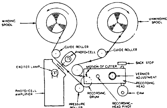
FIG. 124. MECHANICAL ARRANGEMENT OF PHILIPS-MILLER MACHINE
