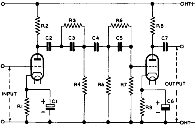
FIG. 30. INTERVALVE COUPLING CIRCUIT FOR GIVING RECORDING CHARACTERISTIC
