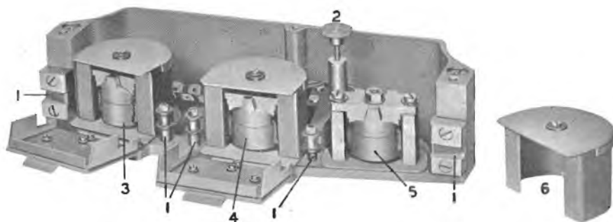
FIG. 113. E.M.I. MAGNETIC RECORDER : HEAD ASSEMBLY
