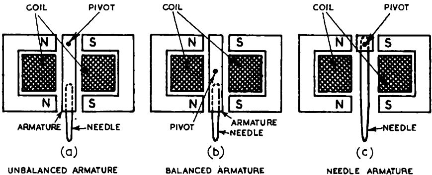
FIG. 75. MOVING-IRON REPRODUCING HEAD : METHODS OF ARMATURE SUSPENSION
