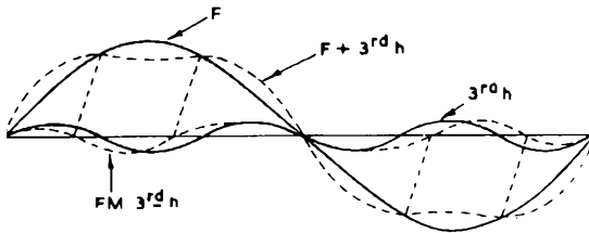
FIG. H3. FREQUENCY MODULATION EFFECT IN PHONOGRAPH PICKUP OUTPUT DUE TO TRACKING ERROR
