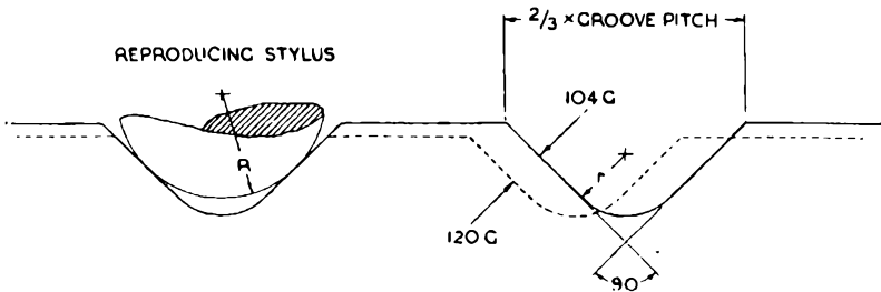
FIG. 20. SECTION OF STANDARD UNMODULATED GROOVE :
