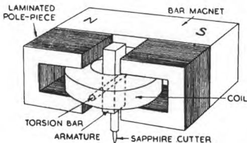
FIG. 28. THEORETICAL DIAGRAM OF MOVING-IRON RECORDING HEAD
