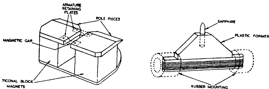
FIG. 80. VOIGT MOVING-COIL REPRODUCING HEAD : CONSTRUCTIONAL DETAILS
