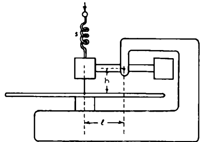
FIG. 32. SHOWING COUNTER-BALANCED HEAD, WITH PIVOTS AT CENTRE OF GRAVITY
