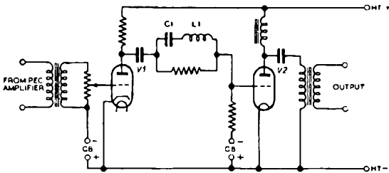
FIG. 131. REPRODUCING AMPLIFIER
