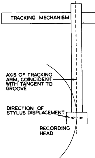
FIG. 87. ILLUSTRATING RADIAL TRACKING WHEN RECORDING
