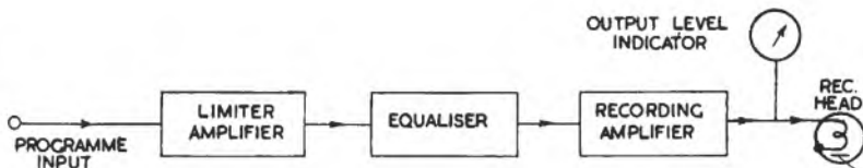
FIG. 46. PRESTO RECORDING CHAIN : BLOCK SCHEMATIC DIAGRAM
