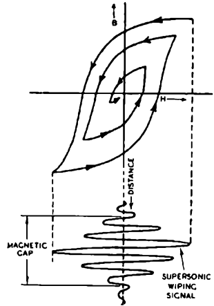
FIG. 108. WIPING PROCESS : MAGNETOPHON
