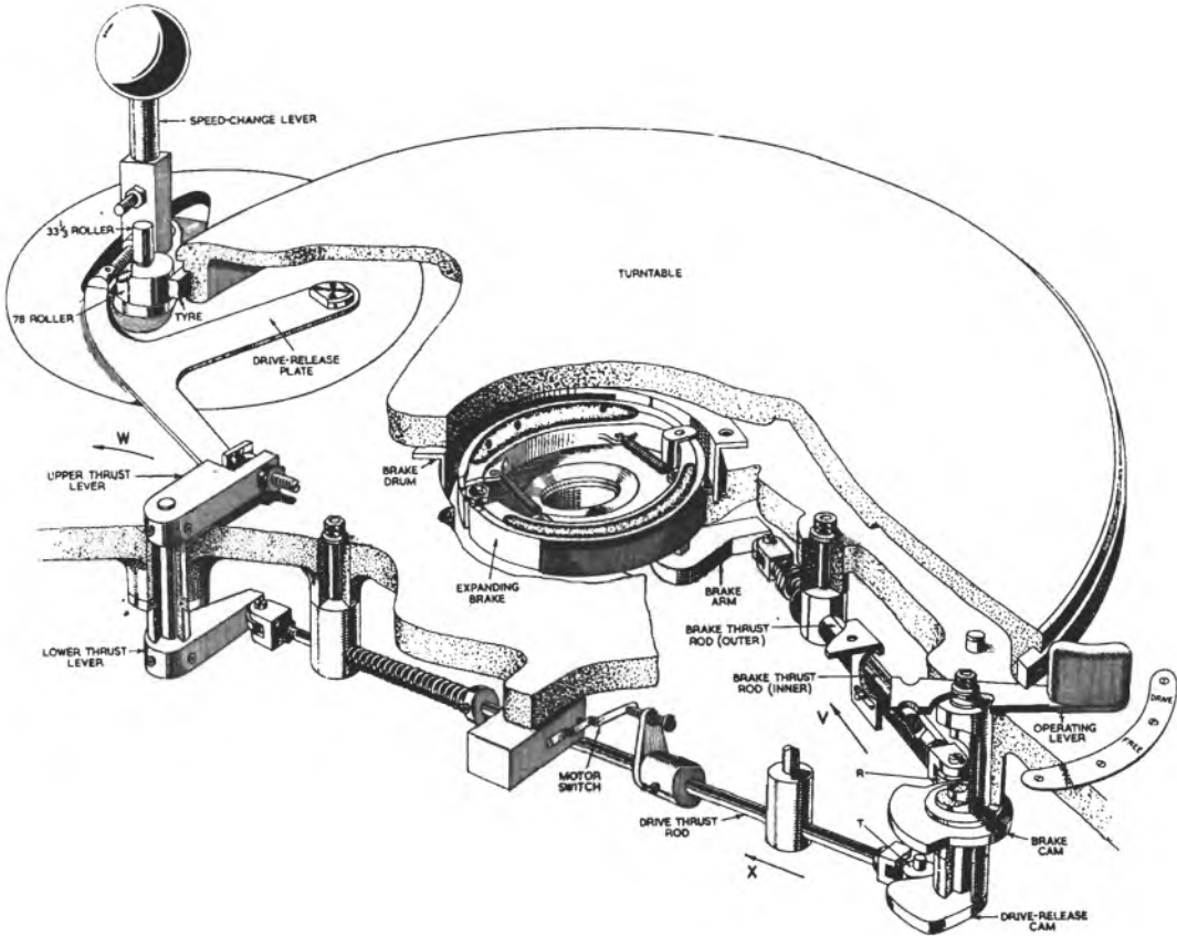
FIG. 92. REPRODUCING DESK DRD/1 ; TURNTABLE CONTROLS
