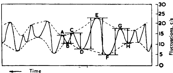
FIG. G9. MEASUREMENT OF WOW ENVELOPE — Trace of Wow Fluctuation - - - Envelope of Wow Fluctuation
