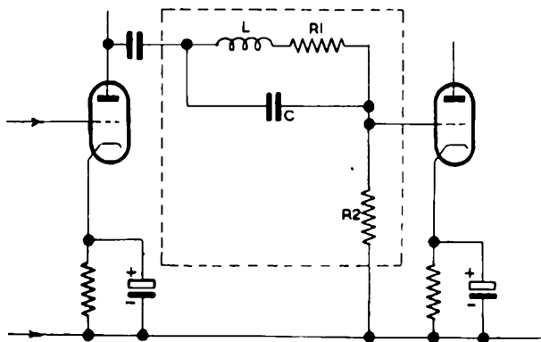
FIG. 38. RECORDING AMPLIFIER EQUALISER CIRCUIT
