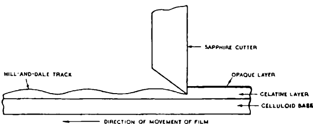
FIG. 122. SECTION THROUGH PHILIPS-MILLER FILM, SHOWING HILL-AND-DALE TRACK
