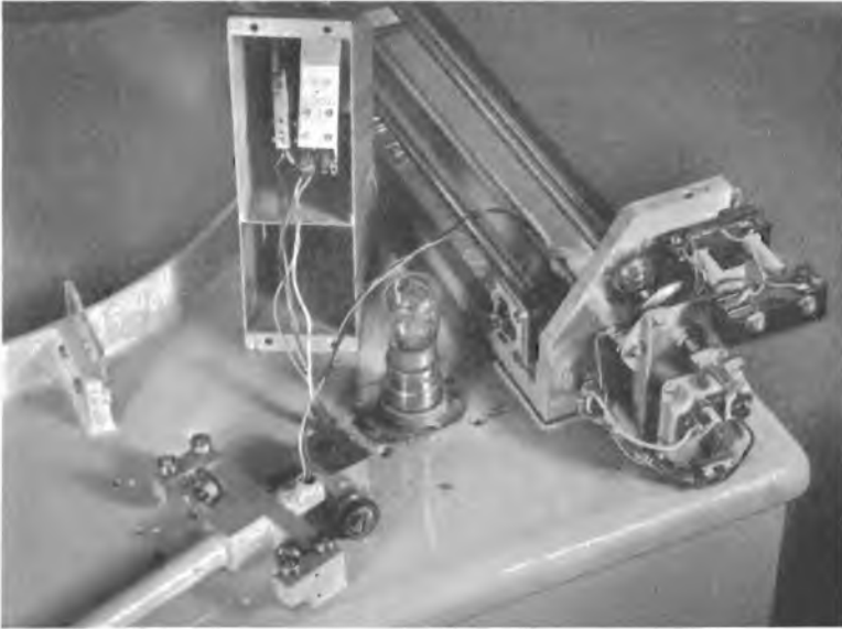
FIG. 93. REPRODUCING DESK DRD/1 ; DETAILS OF GROOVE-LOCATING UNIT GLU/IOA
