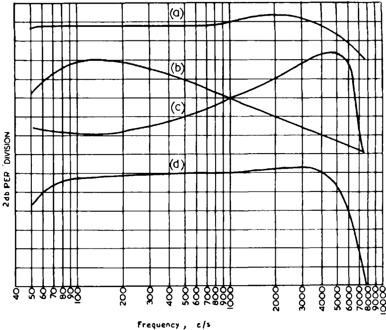
FIG. 105. FREQUENCY RESPONSE CHARACTERISTIC FOR MARCONI-STILLÉ D.P. SYSTEM
