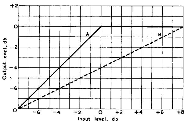
FIG. 12. OPERATING CHARACTERISTICS OF A LIMITING AMPLIFIER
