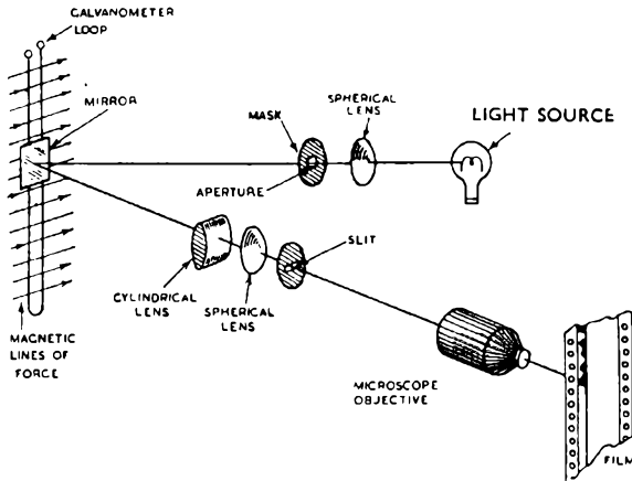
FIG. 117. A METHOD OF VARIABLE-WIDTH RECORDING
