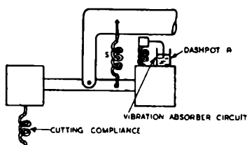
FIG. 34. COUNTERBALANCED HEAD WITH DASH-POT AND ABSORBER CIRCUIT.
