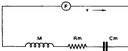
FIG. D4. ELECTRICAL EQUIVALENTS OF MASS, COMPLIANCE AND FRICTION ARE INDUCTANCE, CAPACITANCE AND RESISTANCE
