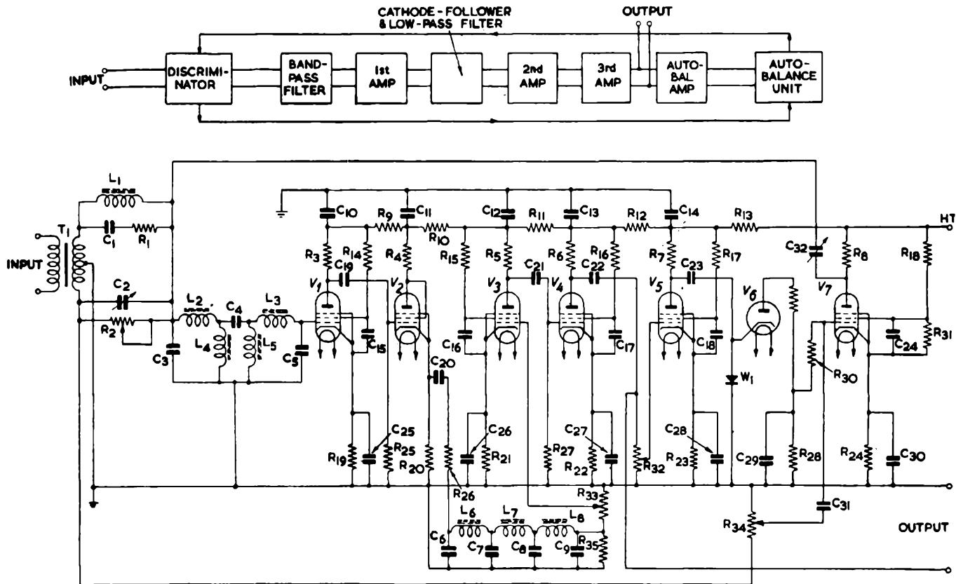
FIG. G14. BLOCK SCHEMATIC AND CIRCUIT DIAGRAMS OF IO-KC/S WOW-MEASURING EQUIPMENT
