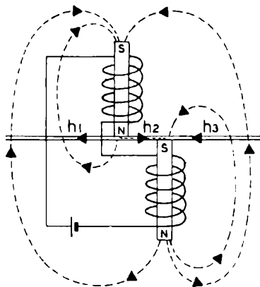
FIG. 103. MARCONI-STILLÉ TWO-POLE-PIECE WIPING SYSTEM
