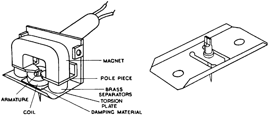
FIG. 79. E.M.I. TYPE-12 HEAD : CONSTRUCTIONAL DETAILS
