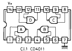
C1.1 CD4011
