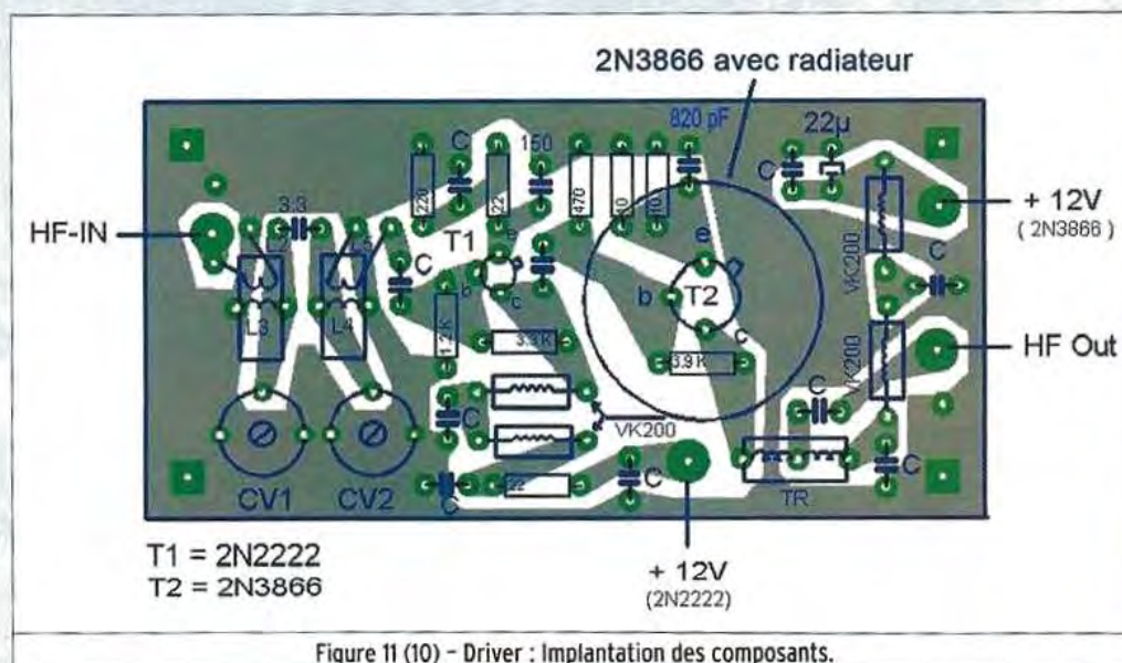
Figure 11 (10) - Driver : Implantation des composants.
