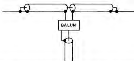
Fig 5—The double bazooka, sometimes called a coaxial dipole. The antenna is self-resonant at 3.75 MHz. The resonator stubs are 43.23-ft lengths of RG-58A coax.
