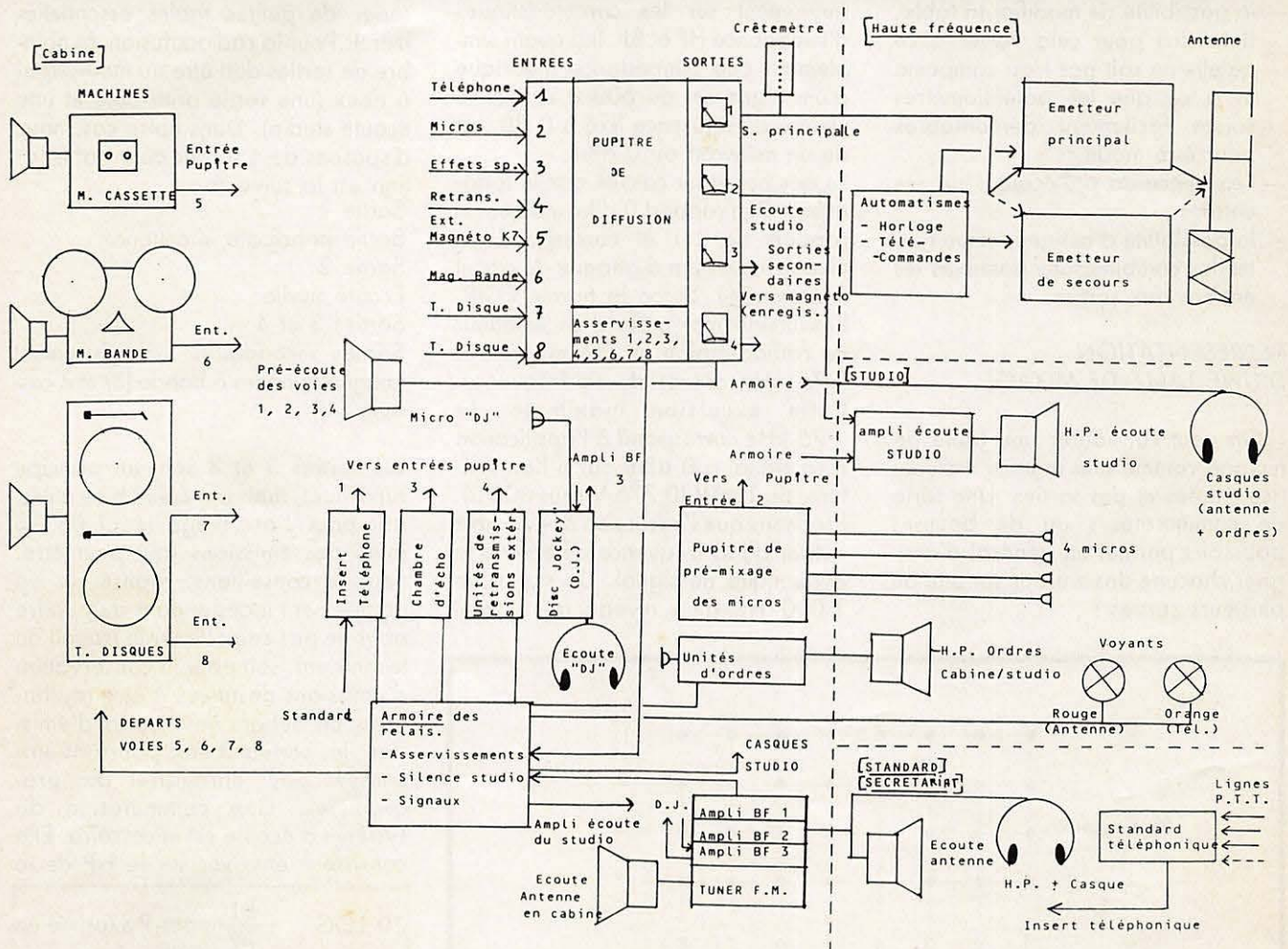
Figure 4 Configuration technique d'une radio locale.
