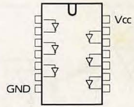
74LS04
