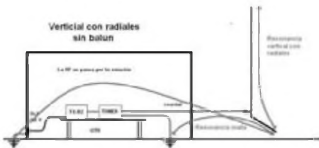
Figura 9: Vertical GP sin balun
