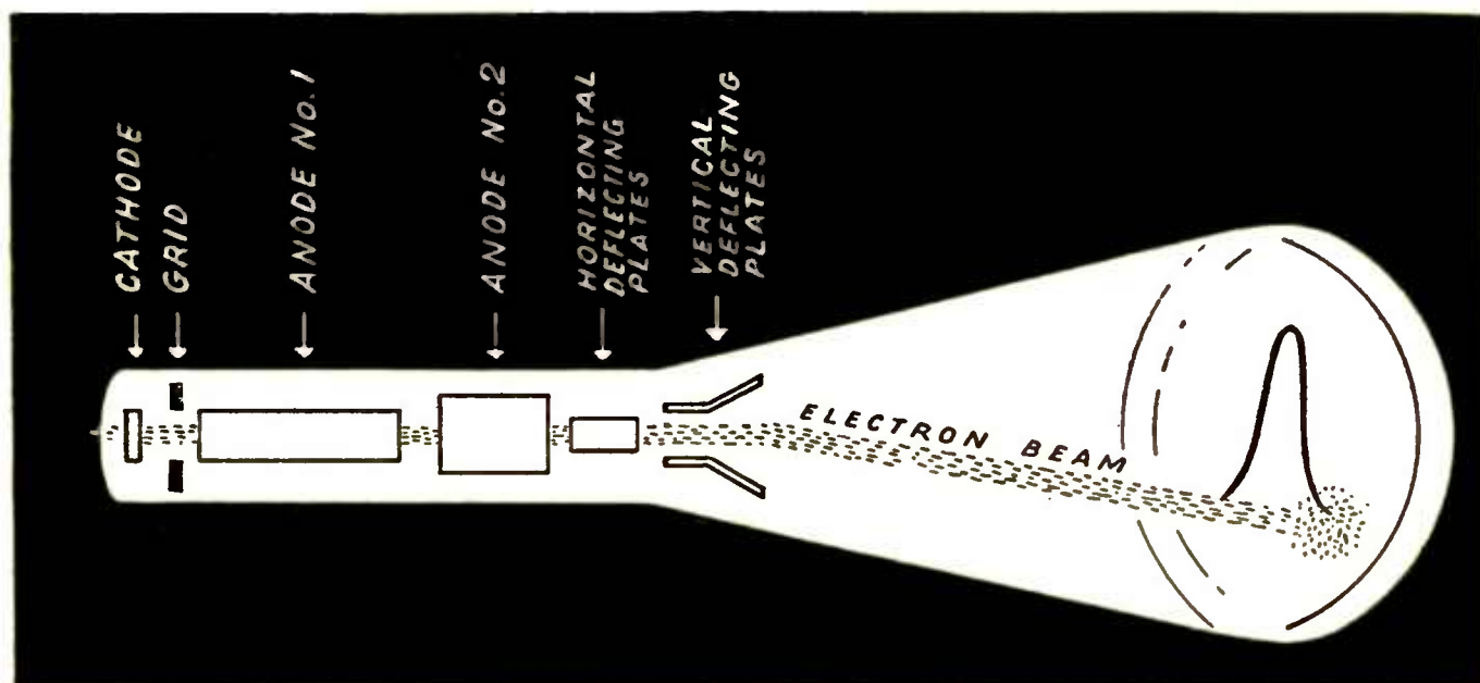
ELEMENTS IN CATHODE-RAY TUBE
