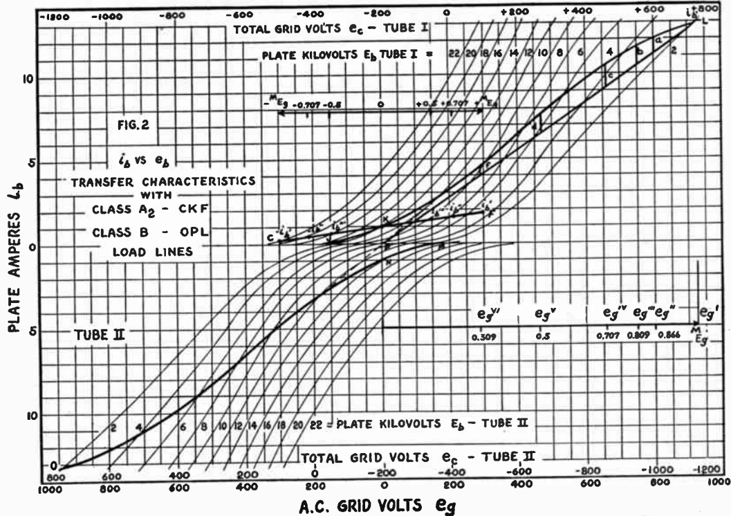
Figure 2— i_b vs e_b Transfer Characteristics with Class A 2 —CKF, Class B—OPL Load Lines.
