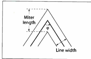
FIGURE 8.11 Miter length
