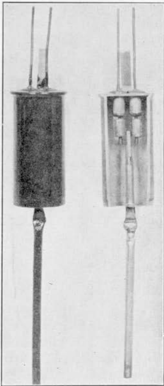
FIG. 83. A single-pole, double-throw vacuum switch.
