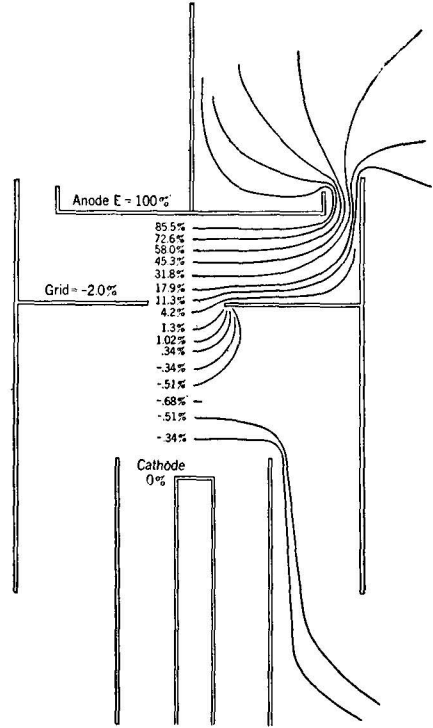
FIG. 58. Potential distribution in a "negative-grid" tube at breakdown.
