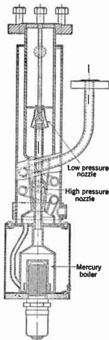
FIG. 5.7.—All-Metal Mercury Condensation Pump (courtesy of General Electric Company).
