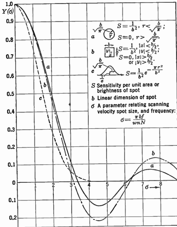
FIG. 6.25.—Aperture Admittance of Various Scanning Spots.
