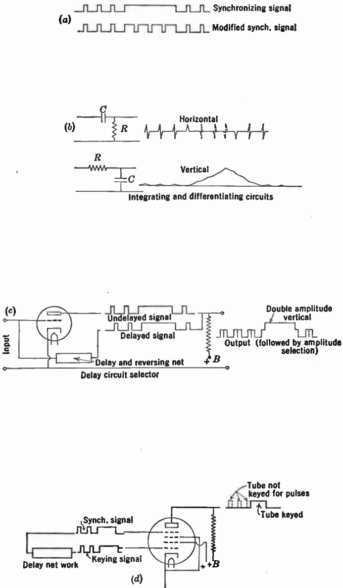
FIG. 15.33.—Duration Selectors.
