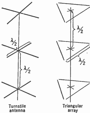
FIG. 16.36.—Turnstile and Triangular Antennas.
