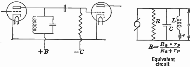
FIG. 17.20.—Simple Intermediate-Frequency Coupling.
