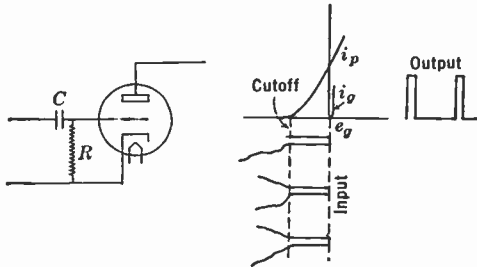
FIG. 15.28.—Grid-Cutoff Separator.
