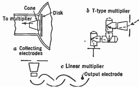
FIG. 11.3.—Secondary-Emission Signal Multipliers Used to Amplify Electron Current from Mosaic.
