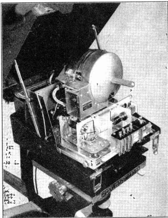
FIG. 18.6.—Interior of Iconoscope Camera (courtesy of NBC).
