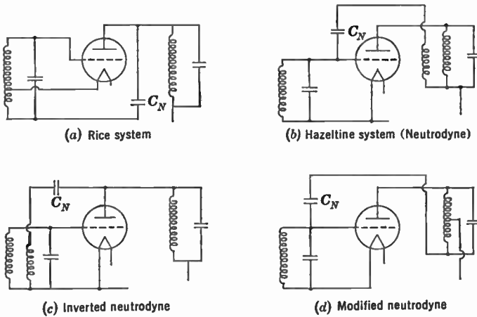
FIG. 16.16.—Systems of Neutralizing Unwanted Capacities.
