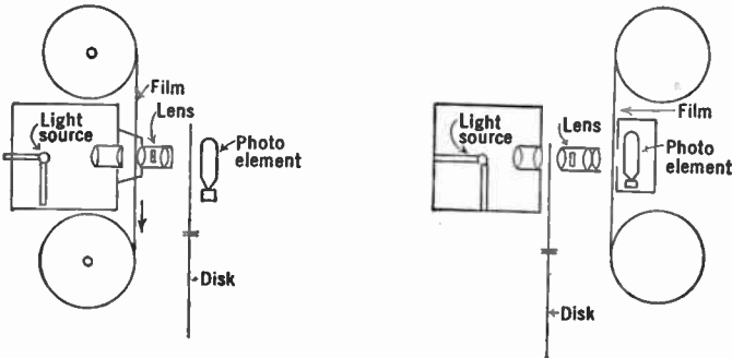
FIG. 8.4.—Two Forms of Simple Disk Film Scanners.
