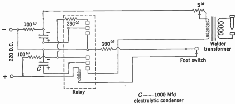
FIG. 5.16.—Circuit Diagram of Impulse Welder.
