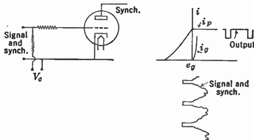
FIG. 15.27.—Positive-Grid Separator.
