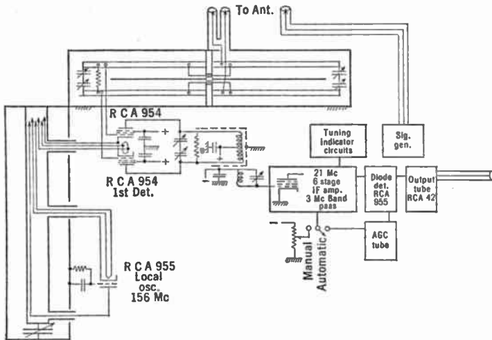
FIG. 19.21.—Schematic Circuit Diagram of Link Receiver.
