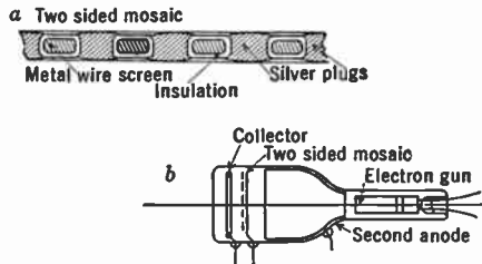
FIG. 11.1.—Iconoscope with Two-Sided Mosaic.
