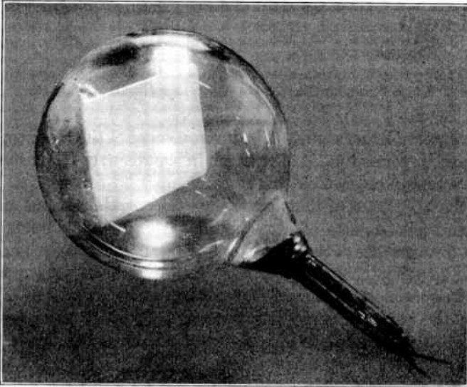
FIG. 12.25.—Front-Surface Kinescope.
