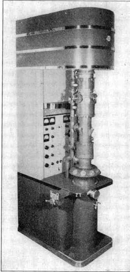
FIG. 4.1.—R.C.A. Electron Microscope.
