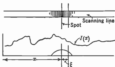
FIG. 6.24.—Scanning with a Finite Aperture.
