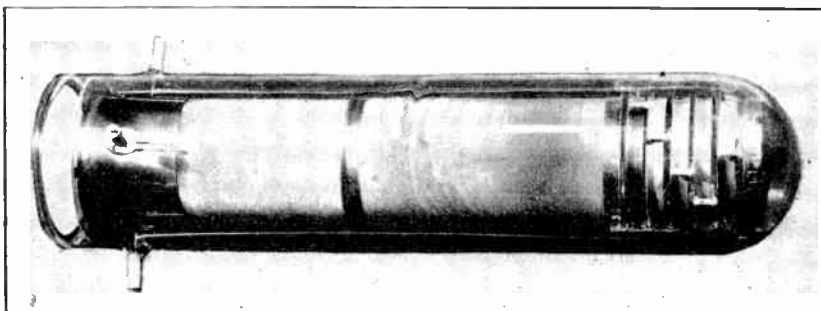
FIG. 4.2.—An Electrostatic Image Tube.
