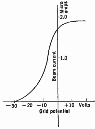
FIG. 10.6.—Current Characteristic of a Typical Iconoscope Gun.
