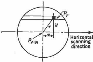
FIG. 13.22.—Determination of Current Distribution in Scanning Line.
