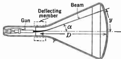
FIG. 15.4.—Deflection of Beam in Kinescope.
