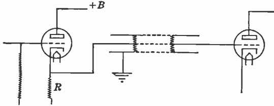
FIG. 14.38.—Cathode-Coupled Driving Circuit for Cable.
