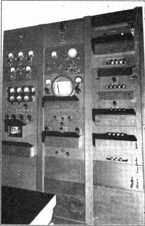
FIG. 10.8.—View of a Typical Iconoscope Test Set.
