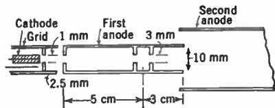
FIG. 13.23.—Elementary Kinescope Gun.
