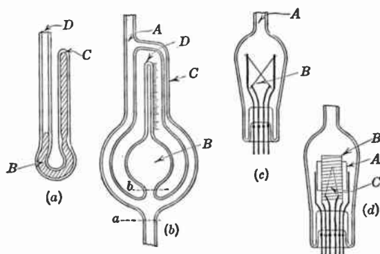
FIG. 5.10.—Vacuum Gauges.
