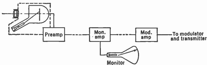
FIG. 14.1.—Video Amplifier Chain at Transmitter.
