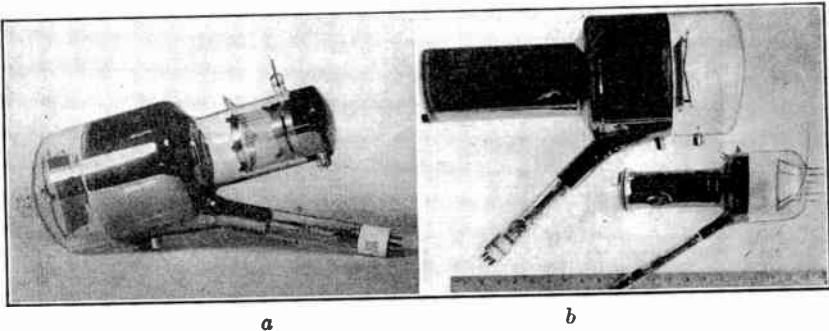
FIG. 11.12.—Electrostatic and Magnetic Image Iconoscopes.
