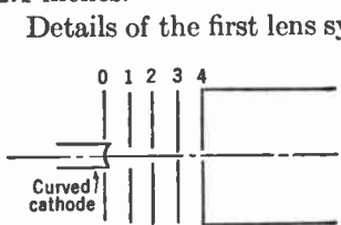
FIG. 13.26.—First Lens of Projection Gun (Law).
