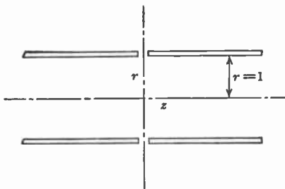
FIG. 4.14.—Coordinates for Electrostatic Cylinder Lens.
