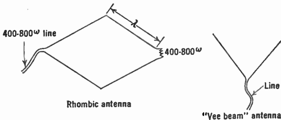
FIG. 17.5.—Some Highly Directive Antennas.
