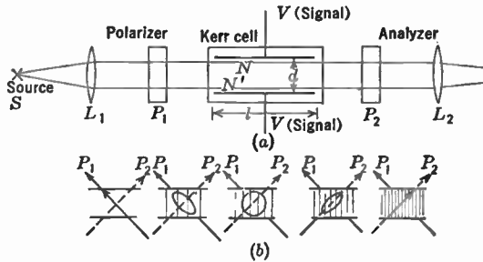
FIG. 9.7.—Principle of the Kerr Cell Light Valve.
