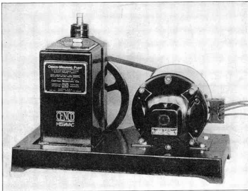
FIG. 5.2.—Cenco Megavac Pump (courtesy of Central Scientific Company).
