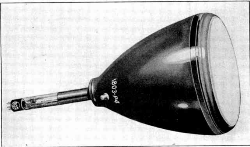
FIG. 12.16.—Twelve-Inch Kinescope RCA 1803-P4.
