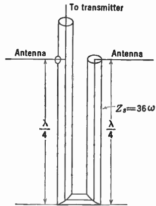
FIG. 16.35.—Coaxial Transformer for Line Division.
