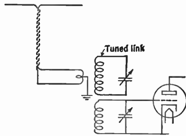
FIG. 17.11.—Input Circuit with Tuned Link Coupling.
