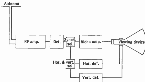
FIG. 7.9.—Television Receiver Employing Radio-Frequency Amplification.
