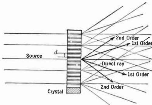
FIG. 9.12.—Diffraction of Light by Supersonic Waves.
