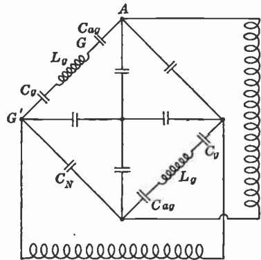
FIG. 16.20.—Compensation for Grid Lead Inductances in Neutralizing Bridge.
