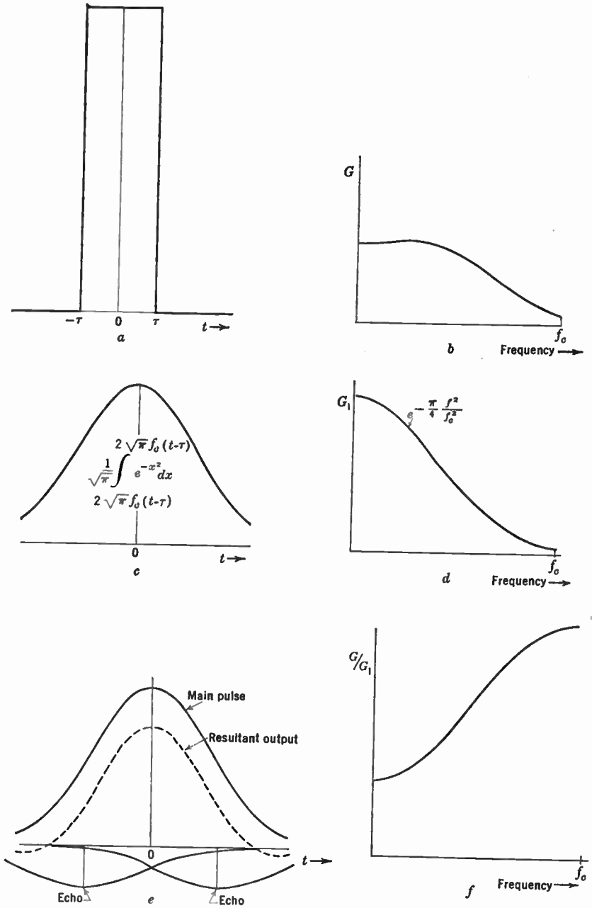
FIG. 14.27.—Determination of Resultant Pulse in the Presence of Amplitude Distortion with the Aid of Positive Paired Echoes.
