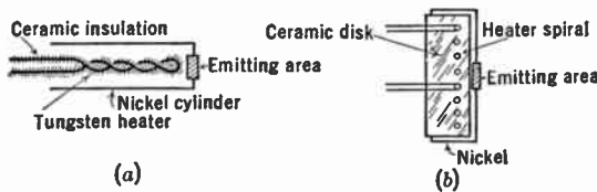
FIG. 13.6.—Typical Indirectly Heated Cathodes.
