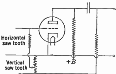
FIG. 15.39.—Simple Keystone Correcting Circuit.
