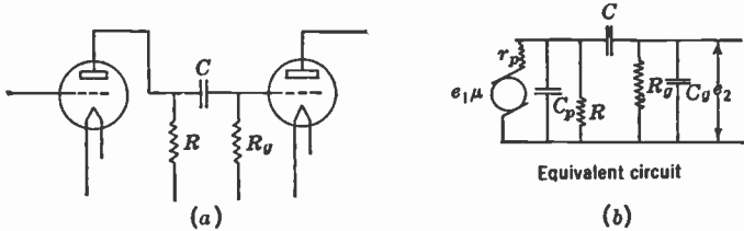
FIG. 14.4.—Simple Resistance-Coupled Stage and Its Equivalent Circuit.
