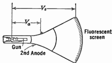
FIG. 2.18.—Schematic Diagram of a Typical Kinescope.
