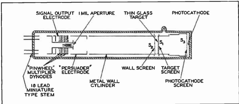
Structure of the MIMO. Ludwell Sibley photo.
