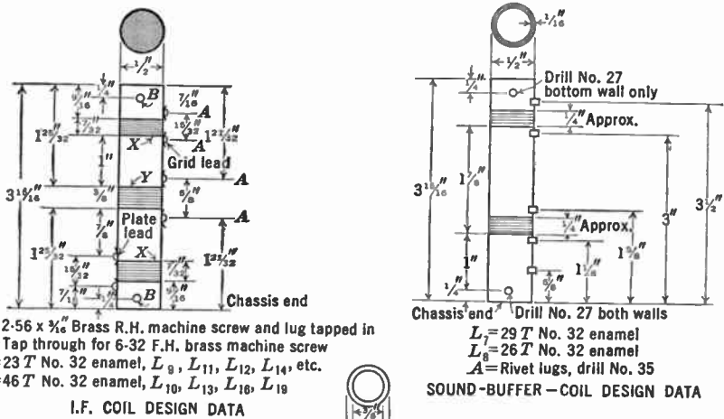
Fig. 17.40.—Coil Design Data I.
