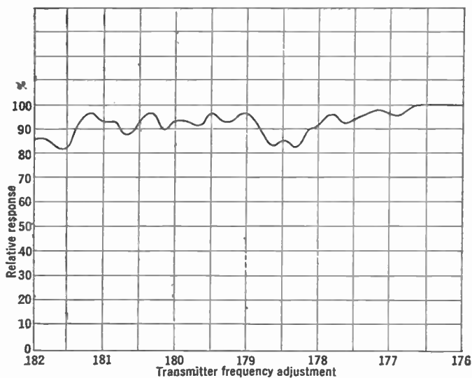
FIG. 19.16.—Variation of Received Signal with Frequency.
