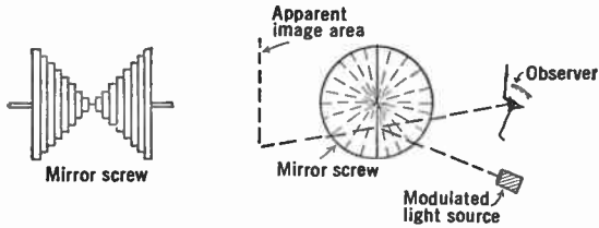
FIG. 9.4.—Mirror Screw.
