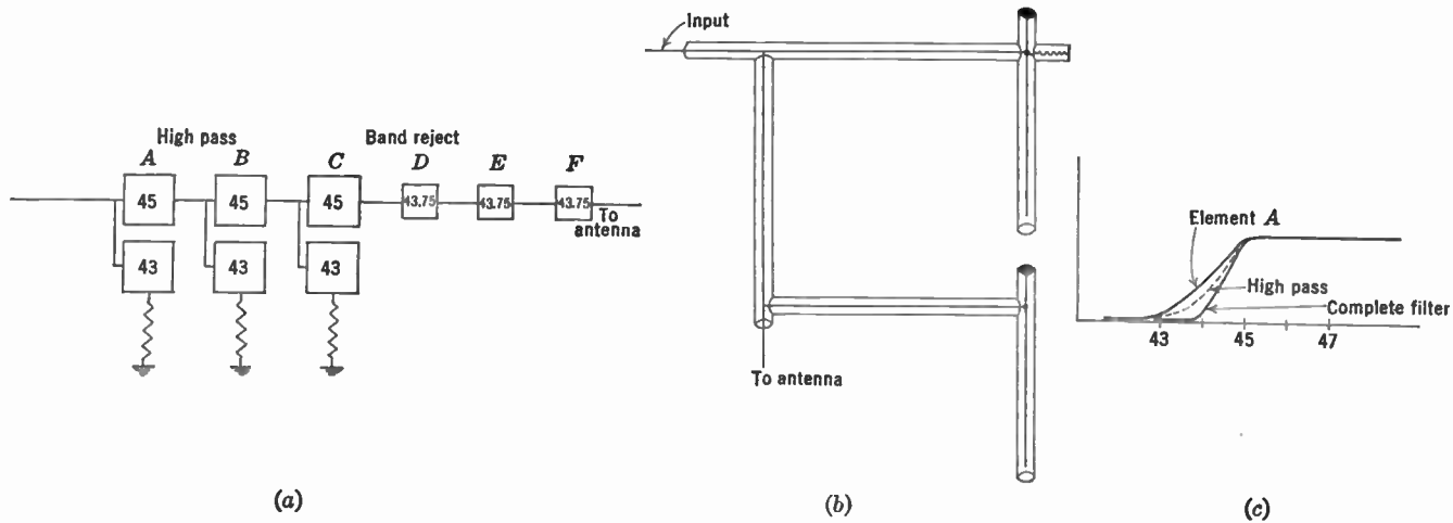
FIG. 19.10.—Coaxial Sideband Elimination Filter.
