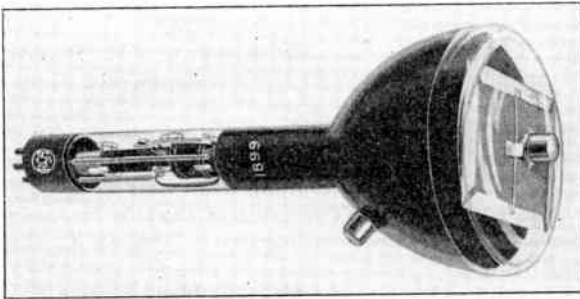
FIG. 11.17.—Monoscope RCA 1899.
