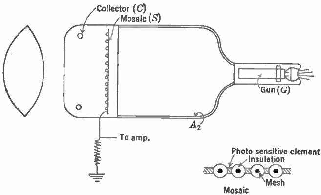
FIG. 8.19.—Diagram of Iconoscope Employing a Two-Sided Mosaic.
