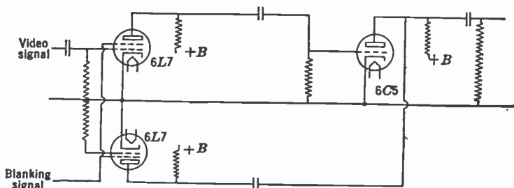
FIG. 14.34.—Balanced Blanking Circuit.
