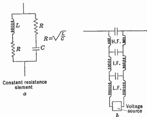
FIG. 19.7.—Constant-Resistance Networks.
