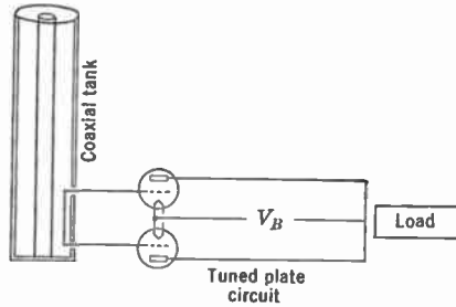
FIG. 16.8.—Push-Pull Concentric Tank Oscillator.
