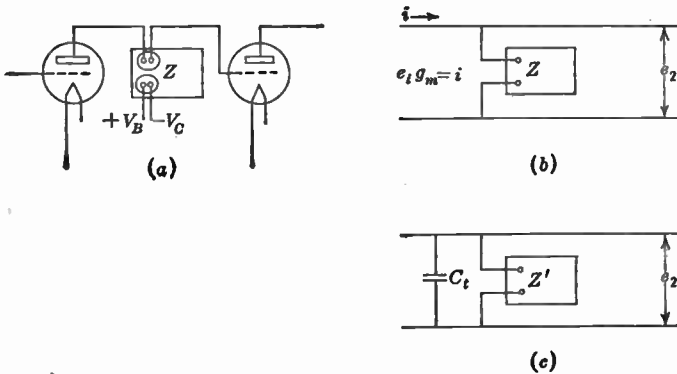
FIG. 14.11.—Two-Terminal Network as Amplifier Coupling.
