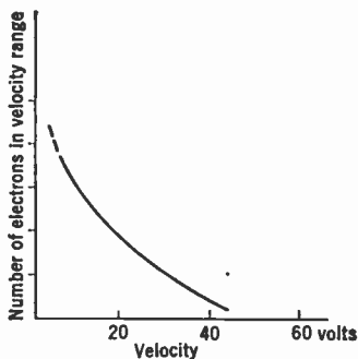
FIG. 1.19.—Velocity Distribution of Secondary Emission from Molybdenum.
