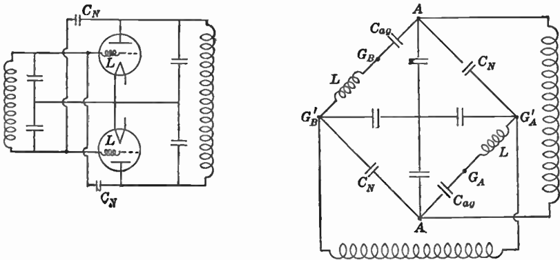
FIG. 16.19.—Effective Grid Lead Inductances in Neutralizing Circuits.
