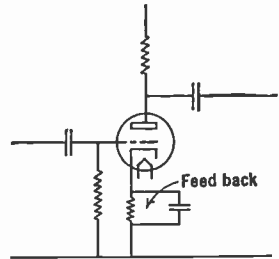
FIG. 14.18.—Simple Feed-back Circuit for Correcting Frequency Response.
