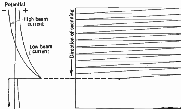
FIG. 10.11.—Distribution of Potential on Mosaic.
