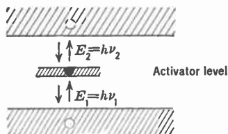
FIG. 2.7.—Electronic Transitions in the Presence of Impurities.
