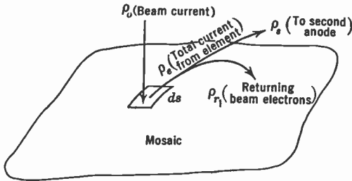
FIG. 10.17.—Current Components for an Element under the Beam.
