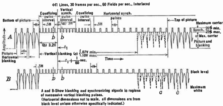
FIG. 7.12.—RMA Standard Television Synchronizing Signal.
