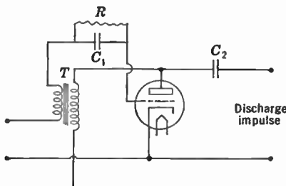
FIG. 15.23.—Blocking Oscillator.
