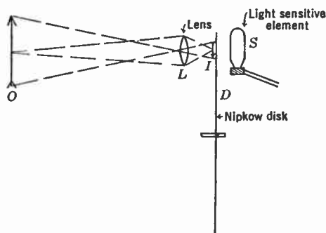
FIG. 8.2.—Direct Pickup Using a Nipkow Disk.
