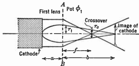
FIG. 13.3.—First Lens of Ideal Gun.
