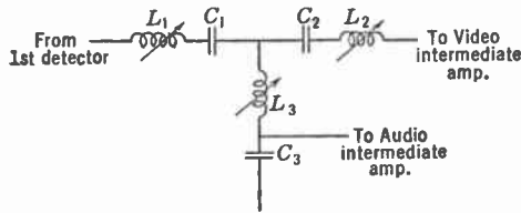
FIG. 17.17.—Selector Separating Video and Audio Intermediate-Frequency Signals.
