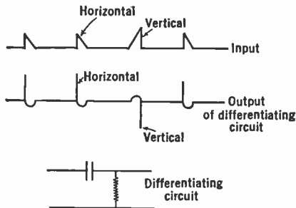
FIG. 15.32.—Differentiation Selector.
