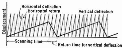
FIG. 15.3.—Sawtooth Displacement Components Required for Scanning.
