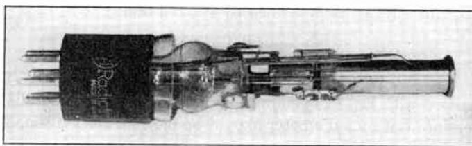
FIG. 13.24.—Photograph of a Typical Kinescope Gun.
