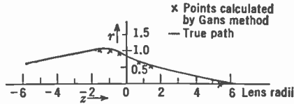
FIG. 4.13.—Electron Trajectory through Cylinder Lens.
