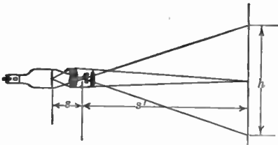
FIG. 12.30.—Optical Arrangement for Projecting Television Pictures.
