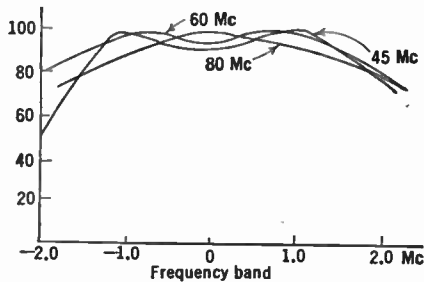
FIG. 17.12.—Response Characteristics of Input Circuit Shown in Fig. 17.11.
