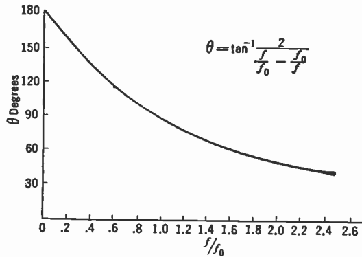
FIG. 14.31.—Phase Response of Network Shown in Fig. 14.30.
