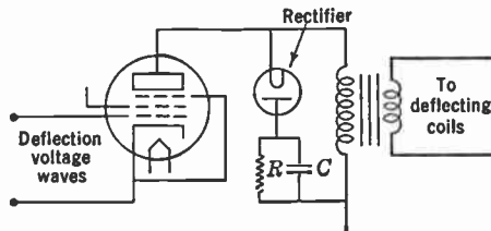
FIG. 15.20.—Diode Used in Special Damping Circuit.
