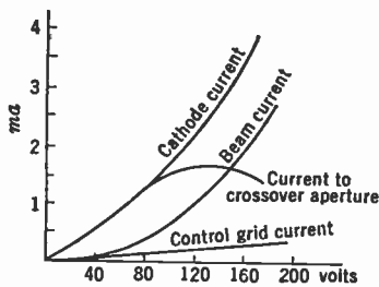
FIG. 13.28.—Current Characteristics of Law's Projection Gun.
