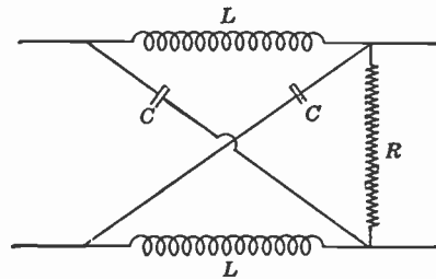
FIG. 14.30.—Phase Correcting Network.
