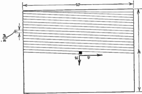
FIG. 6.2.—Scanning Pattern.
