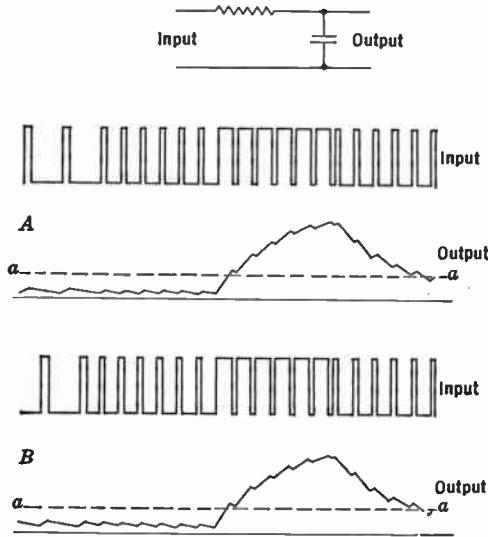
FIG. 17.34.—Selection of Vertical Synchronizing Signal.
