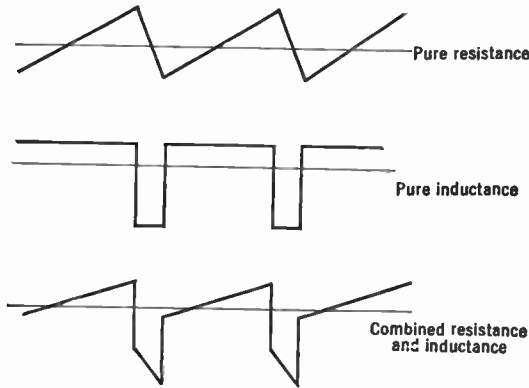
FIG. 15.19.—Voltage Wave Shapes Required for Sawtooth Deflection.
