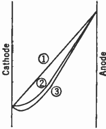
FIG. 1.9.—Effect of Space Charge on Potential Distribution.
