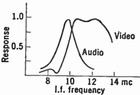
FIG. 17.19.—Response of Circuit Shown in Fig. 17.17 to Audio and Video Intermediate-Frequency Signals.
