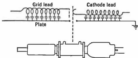
FIG. 16.27.—Approximate Equivalent Network of Electrodes of High-Power Ultra-High-Frequency Transmitting Tube.
