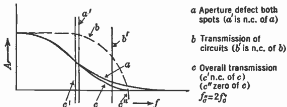
FIG. 6.30—Channel Characteristic as Resultant of Aperture Defect and Circuit Response.
