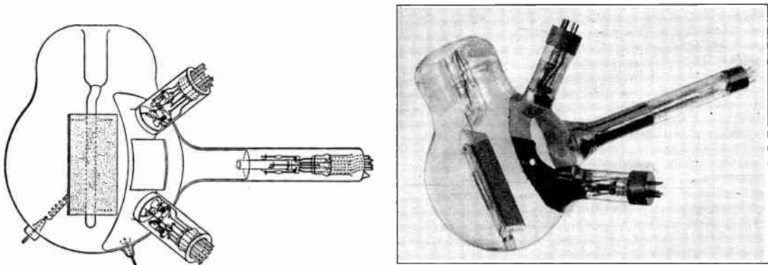
FIG. 11.4.—Signal-Multiplier Iconoscope.
