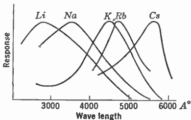
FIG. 1.11.—Spectral Selective Effect of the Alkali Metals (after Hughes and DuBridge).
