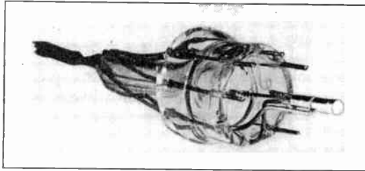
FIG. 13.7.—Photograph of Cathode Assembly.
