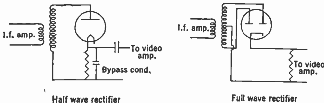
FIG. 17.29.—Typical Second Detector Circuits.
