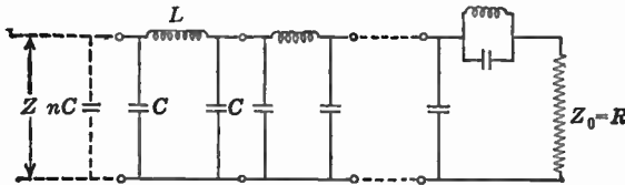
FIG. 14.15.—Constant-k Network.
