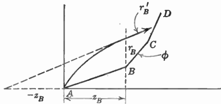
FIG. 4.20.—Determination of Electron Trajectory Near Cathode in Gans Method of Ray Tracing.
