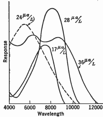
FIG. 11.6.—Spectral Response of Various Semi-Transparent Photocathodes.
