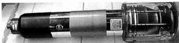
4.5 inch image orthicon. Dave Johnson photo.
