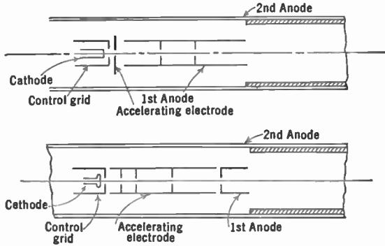
FIG. 13.14.—Lens Systems Employing Additional Electrodes.
