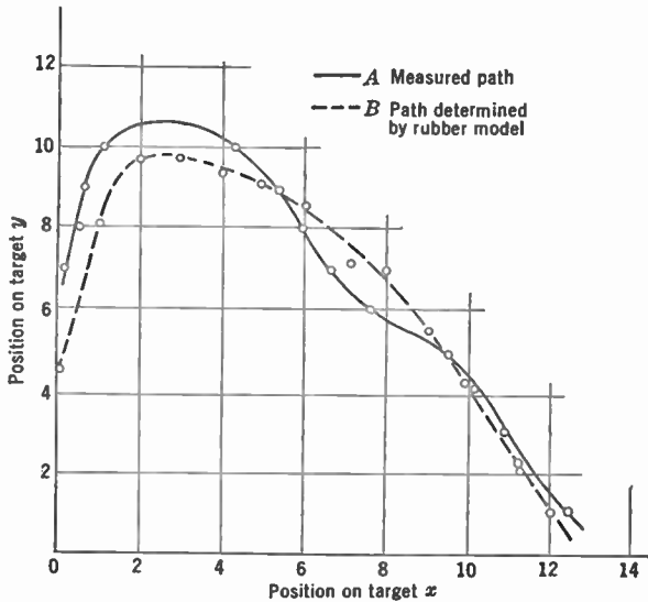
FIG. 3.11.—Curves Showing Termini of Electron Trajectories in the Multiplier as Determined by Direct Measurement and from a Rubber Model.
