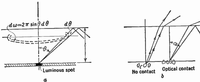
FIG. 12.12.—Reflection and Refraction in the Tube Face.
