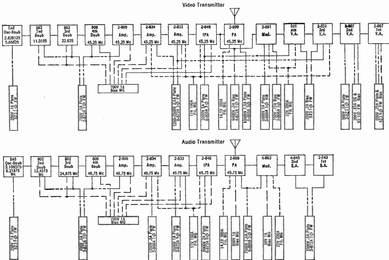
FIG. 19.3.—Block Diagram of Empire State Transmitter (courtesy of NBC).
