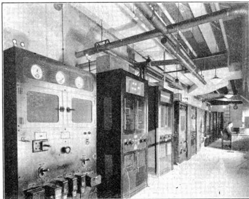
FIG. 19.8.—View of Complete Television Transmitter (courtesy of NBC).
