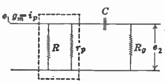
FIG. 14.7. — Low-Frequency Equivalent Circuit of a Resistance-Coupled Stage.
