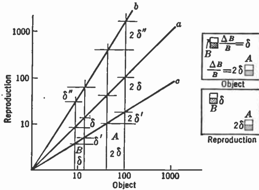
FIG. 6.17.—Relative Contrasts in Object and Reproduction.
