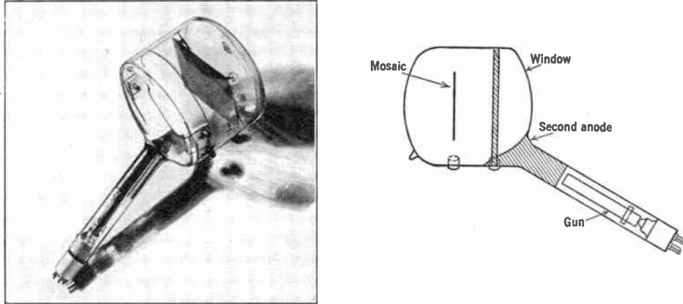
FIG. 10.1.—Photograph and Diagram of an Iconoscope.
