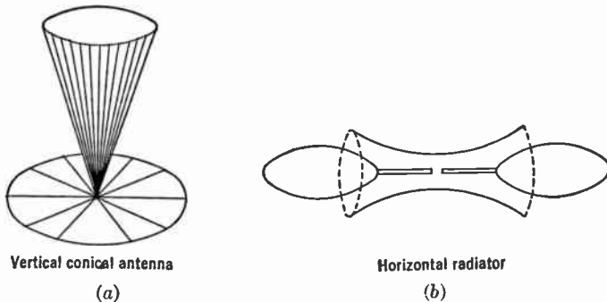
FIG. 16.37.—Special Wide-Band Television Antennas.
