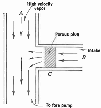
FIG. 5.5.—Principle of Diffusion Pump.
