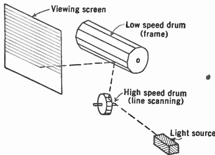
FIG. 9.5.—Television Reproducer Using High- and Low-Speed Mirror Drums.
