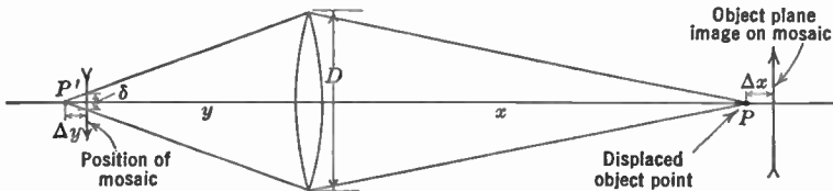
FIG. 10.21.—Determination of Depth of Focus.
