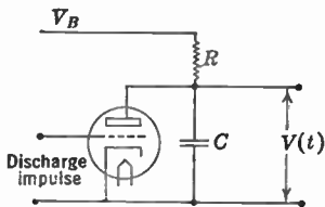
FIG. 15.16.—Grid-Glow Tube Sawtooth Generator.
