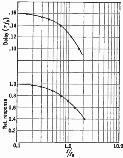
FIG. 14.6.—Response of the Coupling Shown in Fig. 14.5.
