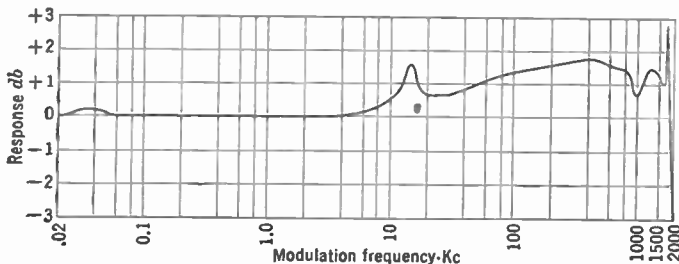
FIG. 19.22.—Overall Response Characteristic of Television Relay Link.
