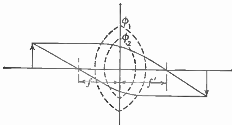
FIG. 4.8.—Double-Layer Lens.
