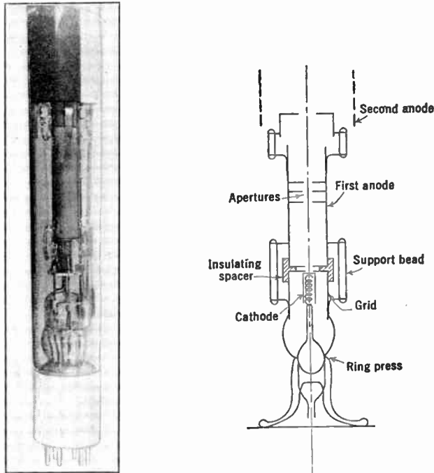
Fig. 10.2.—Iconoscope Gun.
