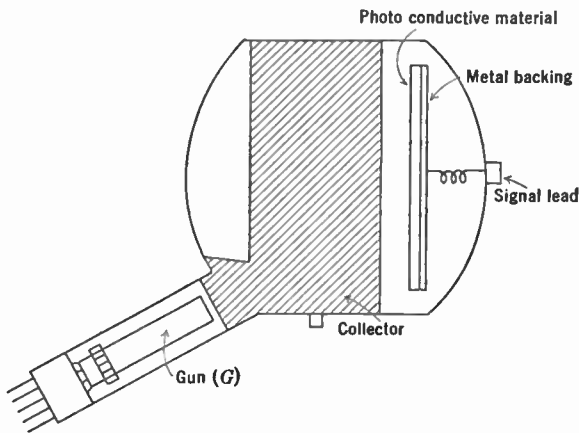
FIG. 8.21.—Photoconductive Pickup Tube.
