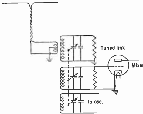
FIG. 17.14.—Complete Input Circuit.
