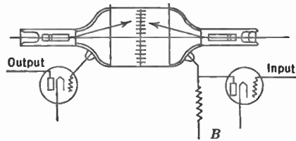
FIG. 11.16.—Storage Tube.
