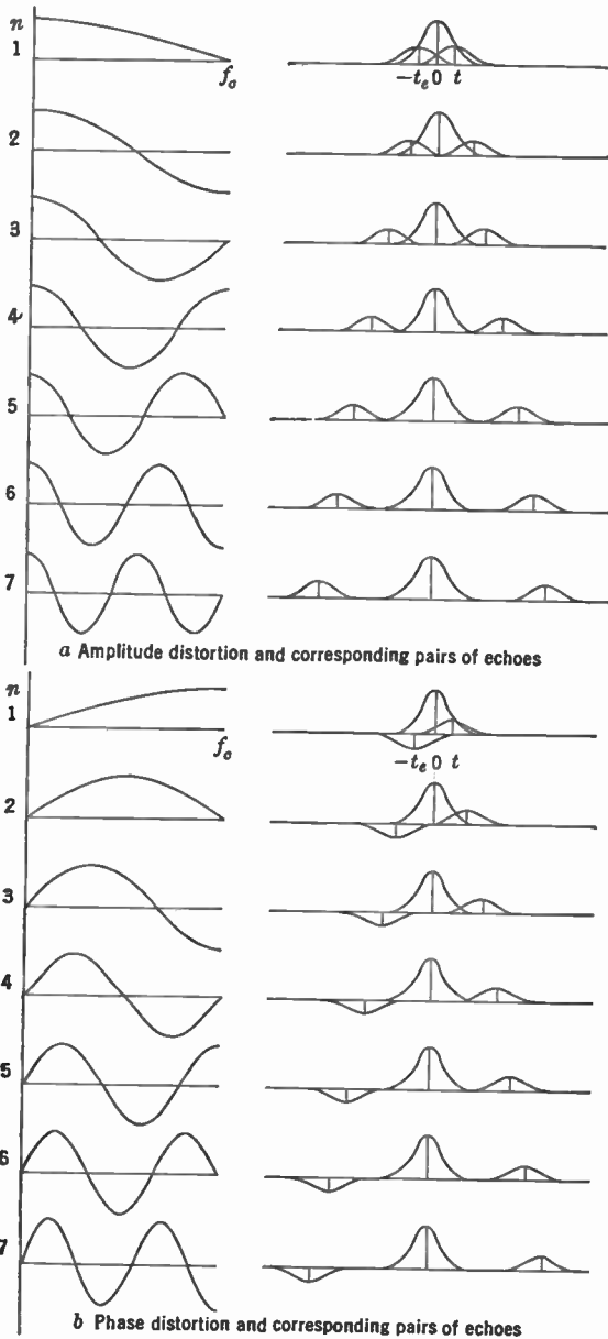
FIG. 14.29.—Echo Pairs for Various Distortion Characteristics.
