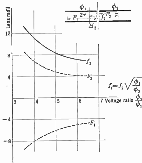
FIG. 4.15.—Focal Length and Position of Focal Points of Cylinder Lens as Function of Voltage Ratio (After Epstein).
