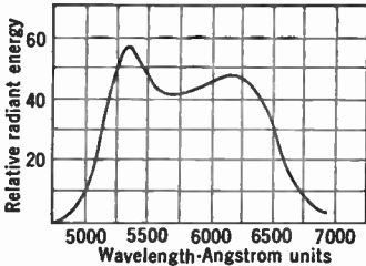
FIG. 12.23.—Spectral Characteristics of White Phosphor No. 4.
