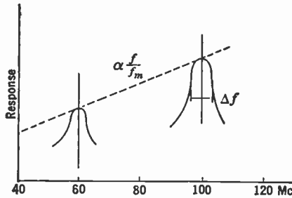
FIG. 17.8.—Response of Simple Input Circuit.
