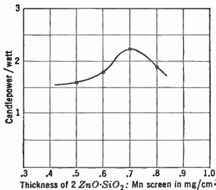
FIG. 12.6.—Light Output as Function of Screen Thickness.
