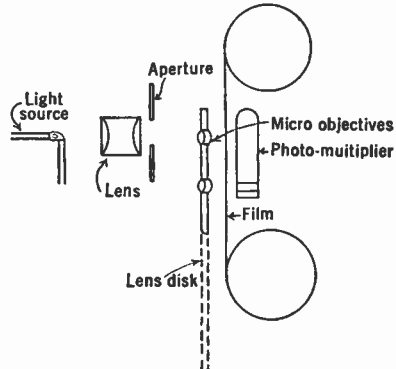
FIG. 8.6.—Film Scanner with Lens Disk.
