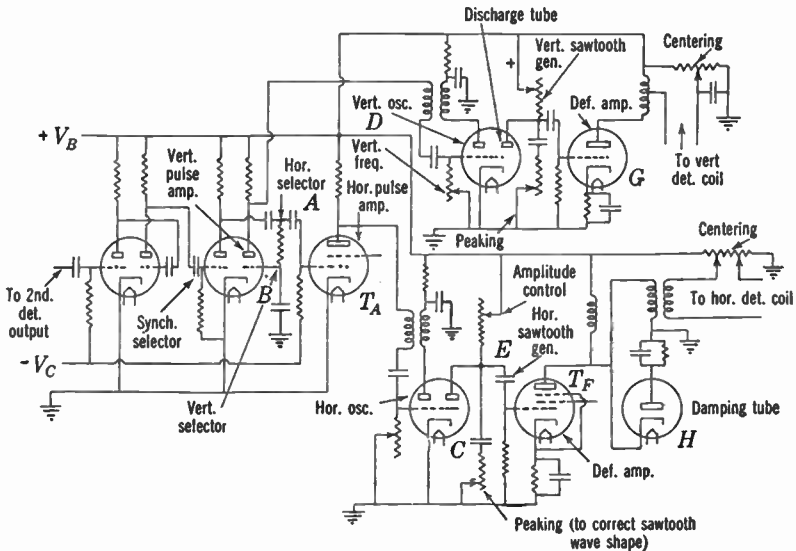
FIG. 17.35.—Typical Synchronizing and Deflecting Circuits.
