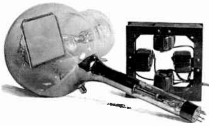
Zworykin's improved (1931) Iconoscope with deflection coil yoke.
