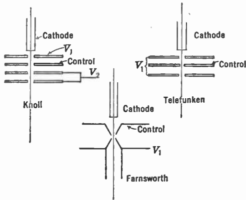
FIG. 13.15.—First-Lens Systems with Crossover Apertures.
