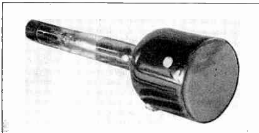
FIG. 12.32.—High-Voltage Projection Kinescope.
