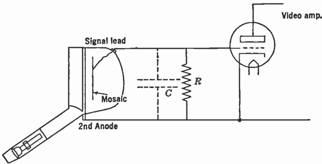
FIG. 10.20.—Simple Iconoscope Coupling Circuit.
