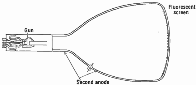
FIG. 12.1.—Diagram of Kinescope.
