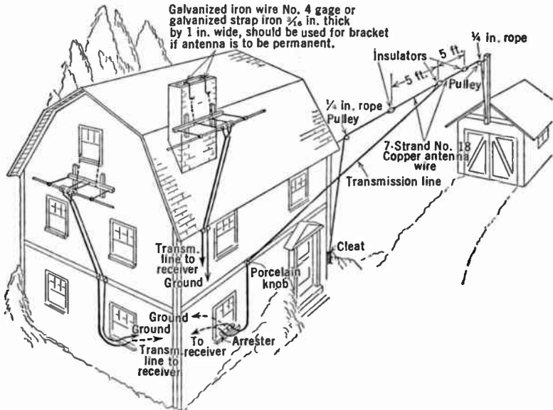
FIG. 17.6.—Practical Television Receiving Antenna Installations.
