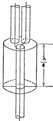
FIG. 16.35.—Coaxial Transformer for Line Division.
