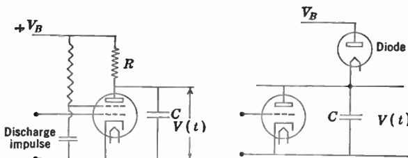
FIG. 15.17.—Sawtooth Generators Employing Hard Vacuum Tubes.
