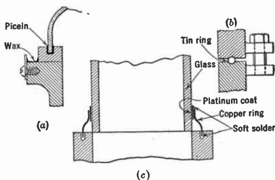
FIG. 5.18.—Vacuum Seals for Demountable Systems.
