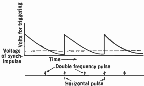
FIG. 15.25.—Sensitivity of Control Oscillator as a Function of Time.
