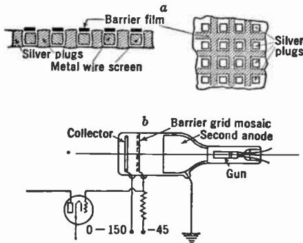
FIG. 11.2.—Barrier-Grid Iconoscope.
