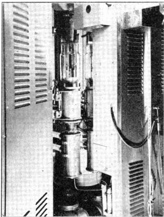
FIG. 19.6.—RCA 899 Output Stage of Empire State Transmitter (courtesy of NBC).
