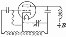
FIG. 17.13.—Local Oscillator of First Detector.
