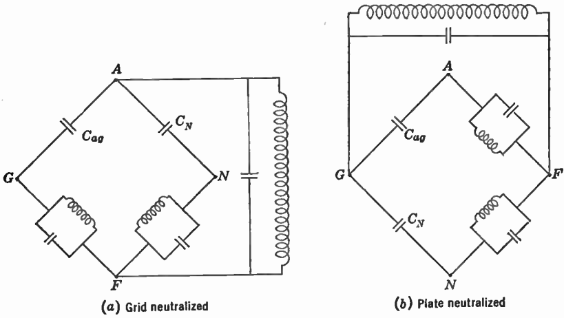
FIG. 16.17.—Unsymmetrical Neutralizing Bridges.
