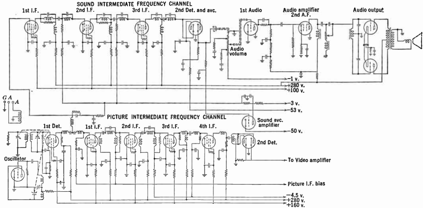
FIG. 17.28.—Radio- and Intermediate-Frequency Circuits of an RCA Experimental Television Receiver.
