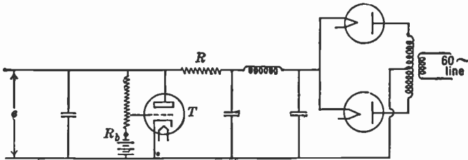
FIG. 14.20.—Regulated Voltage Supply.
