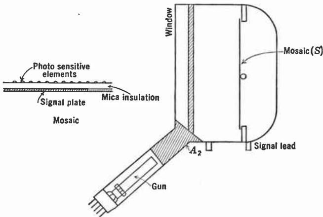
FIG. 8.20.—Normal Iconoscope with a Single-Sided Mosaic.
