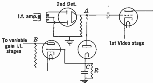
FIG. 17.30.—Automatic Gain Control Circuit.
