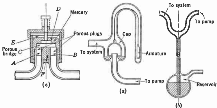
FIG. 5.9.—Typical Vacuum Cutoffs.
