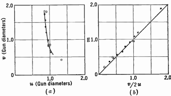
FIG. 11.9.—Focusing Properties of Electrostatic Image Tube.
