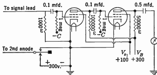
FIG. 10.5.—Vacuum-Tube Meter for Sensitivity Test.
