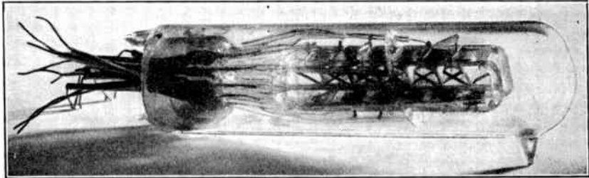
FIG. 3.9.—An Experimental Electrostatic Secondary-Emission Multiplier.
