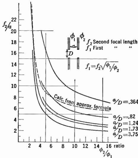
FIG. 4.16.—Focal Length of Double-Aperture Lenses (After Polotovsky).
