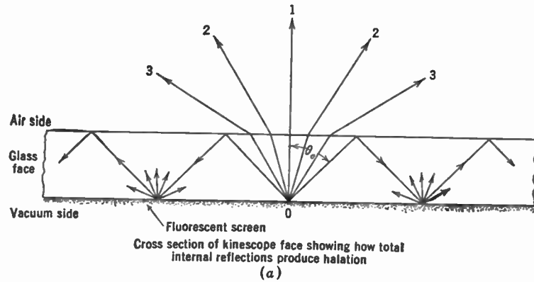
FIG. 12.11.—Internal Total Reflection.
