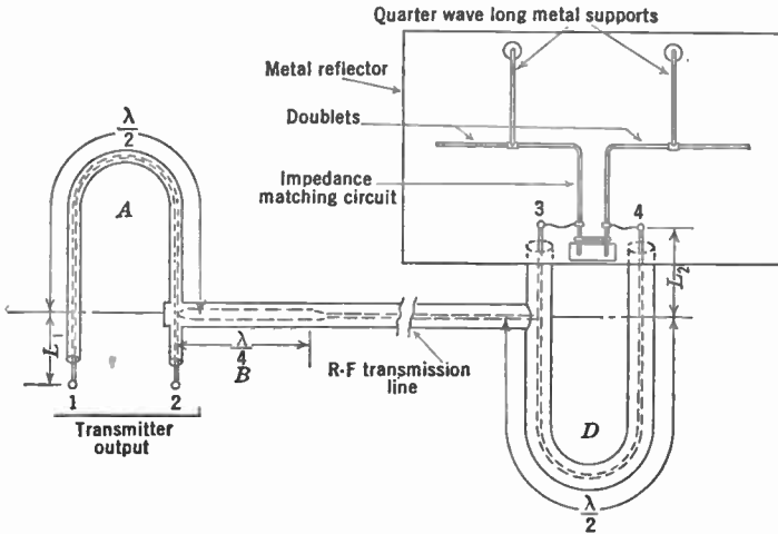
Fig. 19.20.—Antenna Coupling Circuit for Link Transmitter.
