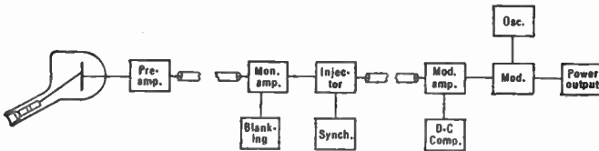
FIG. 14.40.—Block Diagram of Complete Amplifier Including Injector and Blanking Units.
