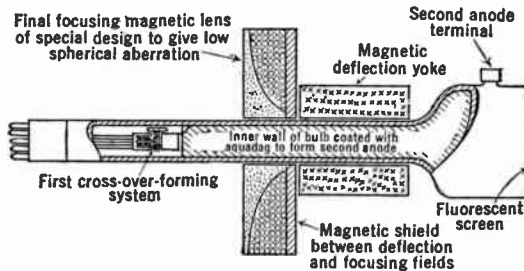
FIG. 13.27.—Diagram of Assembly of Law's Projection Gun.
