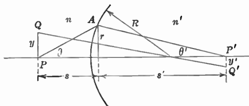
FIG. 4.3.—Refraction at a Curved Surface.
