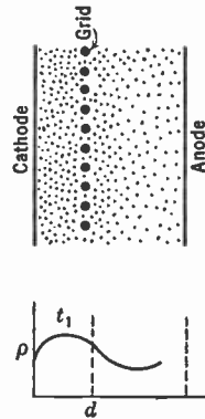
FIG. 17.16.— Electron Distribution in Triode.
