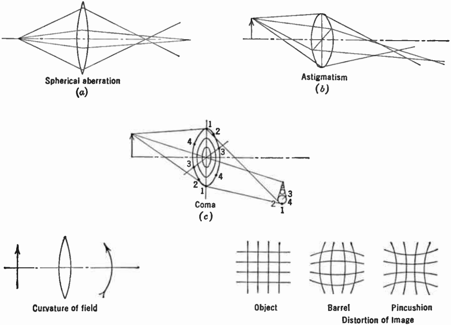
FIG. 4.23.—Nature of the Five Third-Order Aberrations.
