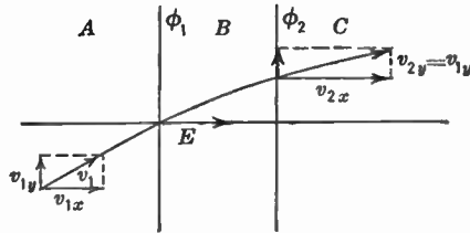
FIG. 4.7.—Refraction by Potential Double Layer.
