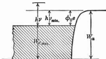
FIG. 1.10.—Electron Energies Associated with Photoelectric Emission.
