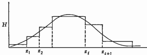
FIG. 4.22.—Approximate Representation of Axial Magnetic Field.
