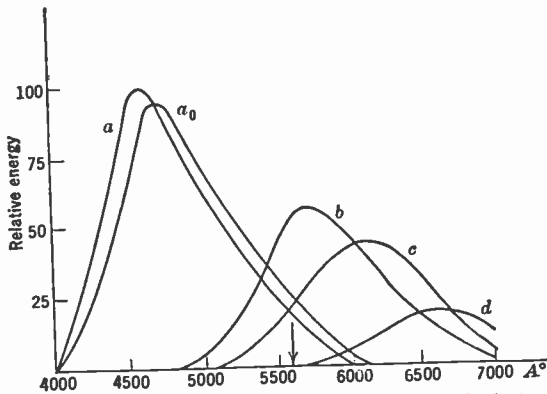
FIG. 2.3.—The Variation of Spectral Characteristics of Zinc Cadmium Sulphide with Zn : Cd Ratio.
