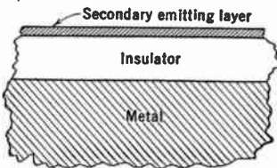
FIG. 1.21.—Thin Film Field Emitter.
