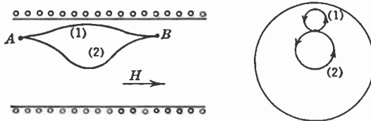
FIG. 4.21.—Electron Paths in a Uniform Magnetic Field.
