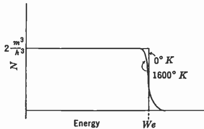
FIG. 1.4.—Distribution of Electron Energies by Fermi-Dirac Statistics.
