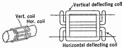
FIG. 15.13.—Simple Form of Air-Core Deflecting Coils.
