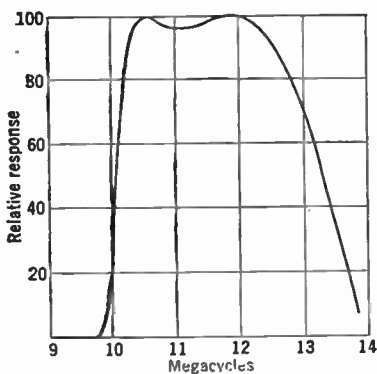
FIG. 17.26.—Overall Response of Intermediate-Frequency Amplifier of an RCA Experimental Television Receiver.
