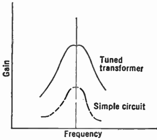
FIG. 17.10.—Comparative Response of Simple and Tuned Transformer Input Circuits.
