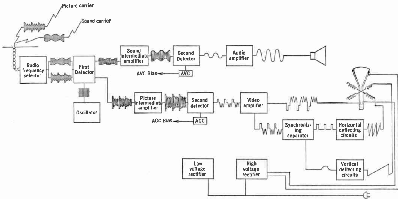
FIG. 17.1.—Block Diagram of Superheterodyne Receiver Showing Wave Forms at Various Points.
