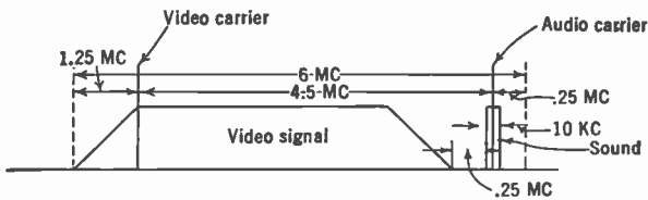
FIG. 7.5.—Utilization of the 6-Megacycle Channel.
