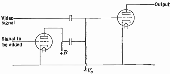
FIG. 14.36.—Simple Injector Circuit.
