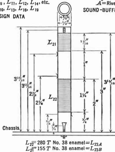
Fig. 17.41.—Coil Design Data II.
