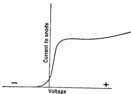
FIG. 1.8.—Idealized Current Characteristics of a Diode.
