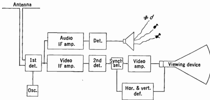
FIG. 7.10.—Block Diagram of a Superheterodyne Television Receiver.
