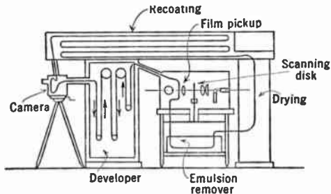
FIG. 8.12.—Continuous Intermediate Film Scanner.
