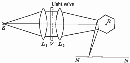
FIG. 9.16.—Large Area Light Valve.
