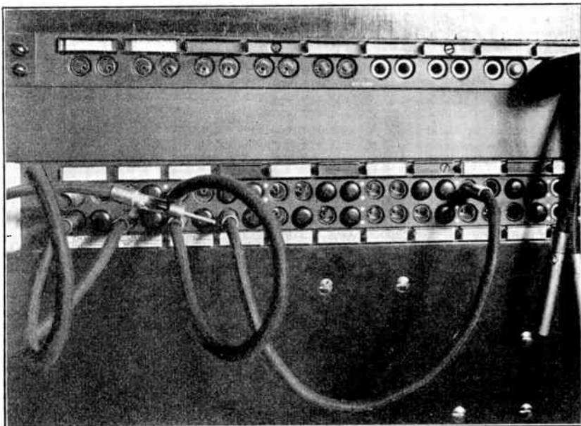
FIG. 18.16.—Coaxial Cable Jack Panel and Patch Cords (courtesy of NBC).
