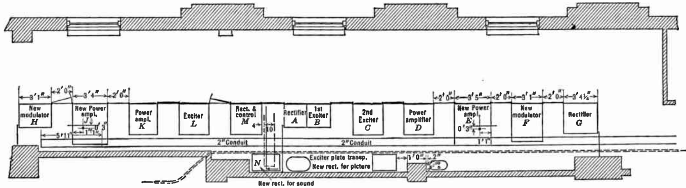
FIG. 19.2.—Layout of Empire State Television Transmitter (courtesy of NBC).
