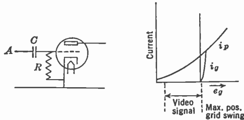
FIG. 17.31.—Restoration of D-C Component of Video Signal.
