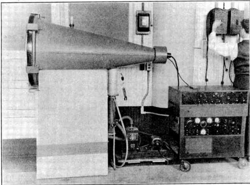
FIG. 12.27.—Thirty-One-Inch Demountable Kinescope.
