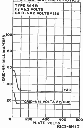
AVERAGE CHARACTERISTICS
