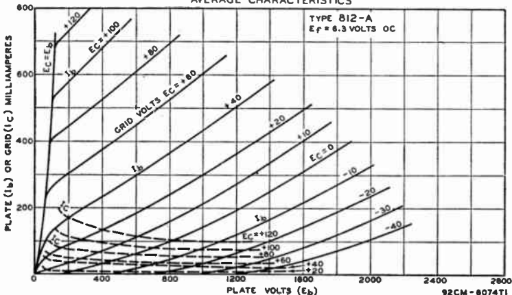
AVERAGE CHARACTERISTICS
