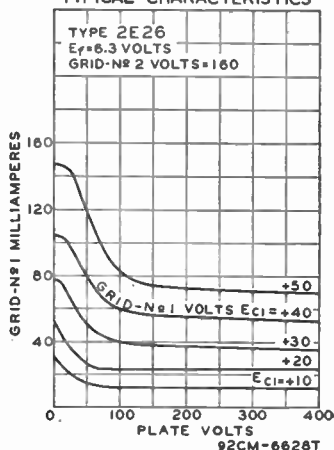
TYPICAL CHARACTERISTICS
