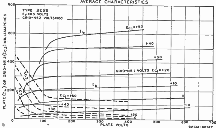
AVERAGE CHARACTERISTICS
