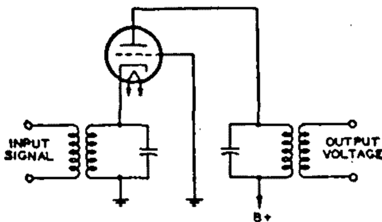
Fig. 47—Cathode-drive circuit.
