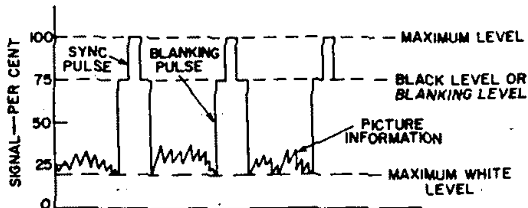
Fig. 79—Detected video signal.
