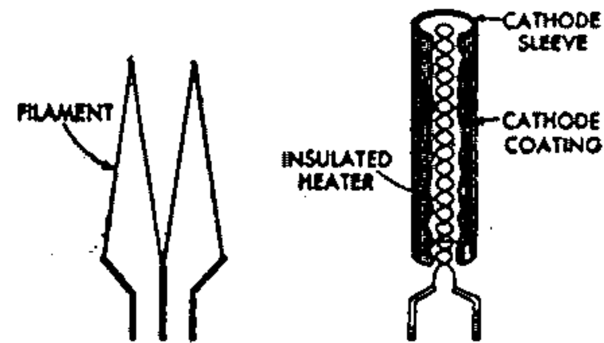
Fig. 1—Filament or directly heated cathode.
