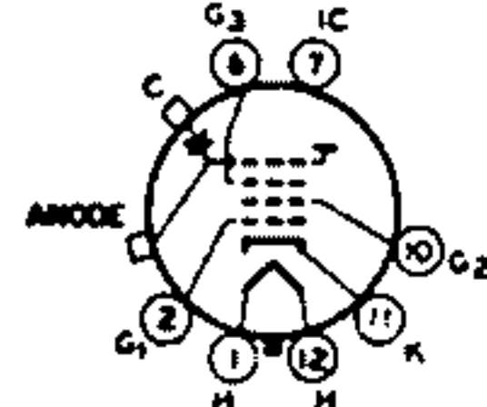
12C ANODE = G 4 + C FOCUSING ELECTRODE - G 3
