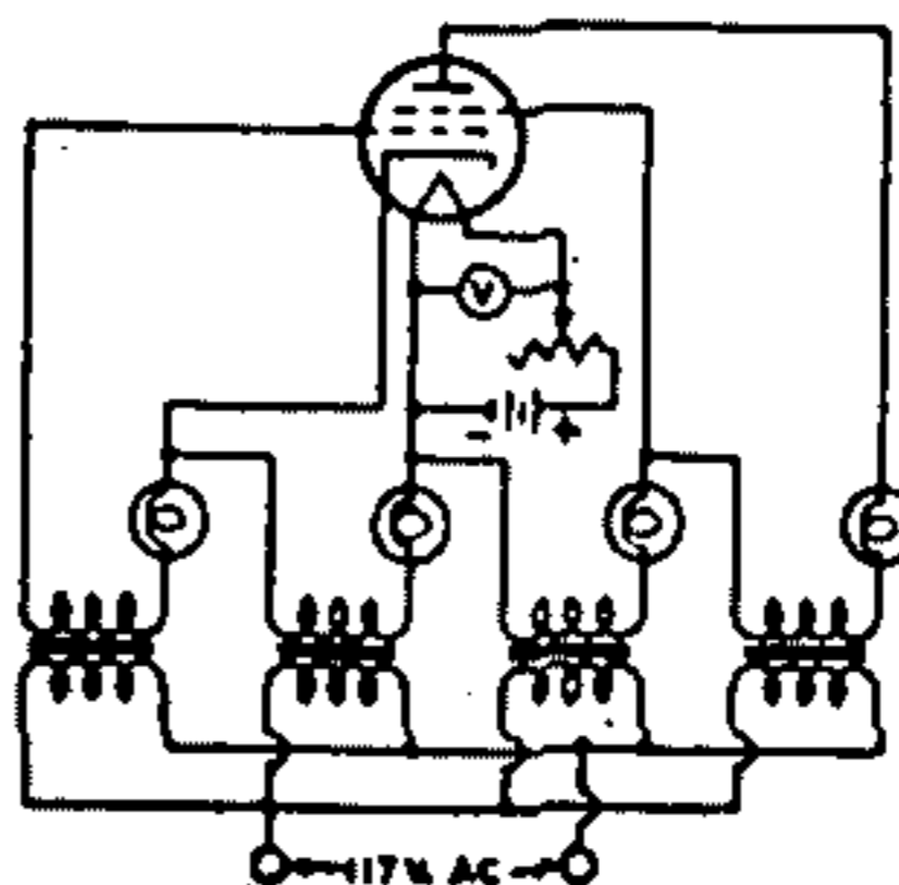
Fig. 129—Fundamental circuit of a short-circuit tester.
