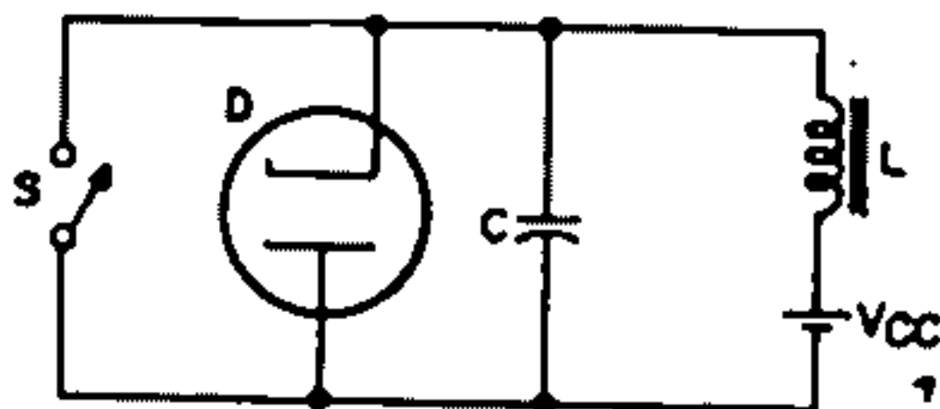
Fig. 88—Incorporation of damper diode.
