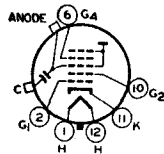
12L ANODE = G 3 + G 2 + C1 FOCUSING ELECTRODE = G 4
