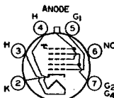
7FG ANODE = G 3 + G 5 + CL AUTOMATIC FOCUSING
