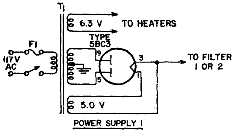
POWER SUPPLY 1
