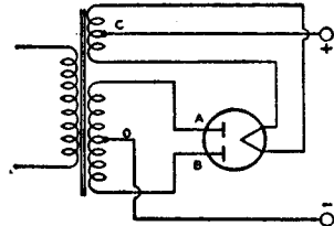
Fig. 104—Schematic diagram of full-wave rectifier tube and circuit connections.
