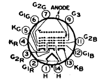
14AH ANODE = G 4 + G 5 + C1 + R FOCUSING ELECTRODE = G 3
