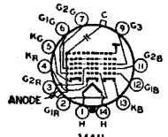
14AU ULTOR = G 4 + G 5 + C1 FOCUSING ELECTRODE = G 3
