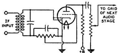
Fig. 54—Diode-biased detector circuit.
