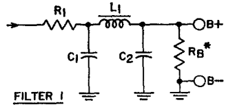
FILTER 1
