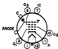
12C ANODE = G_4 + CL FOCUSING ELECTRODE = G_2
