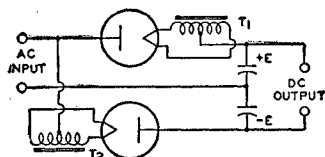
T_1, T_2 = SEPARATE FILAMENT TRANSFORMER WINDINGS
