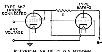
R: TYPICAL VALUE IS 0.5 MEGOHM Fig. 66
