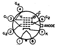
8JK ANODE = G_3 + G_2 + CL FOCUSING ELECTRODE = G_4
