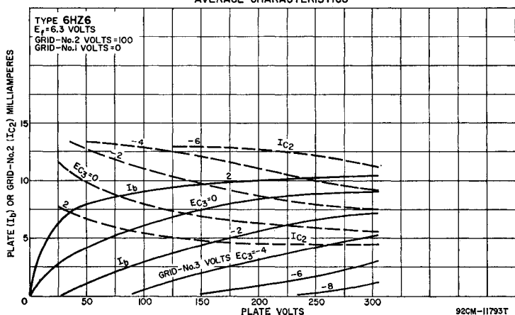
AVERAGE CHARACTERISTICS
