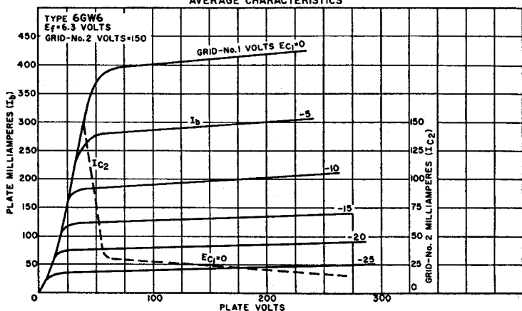
AVERAGE CHARACTERISTICS
