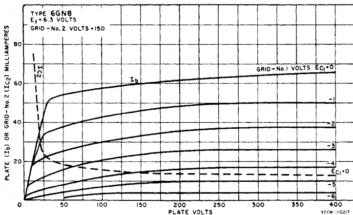
AVERAGE CHARACTERISTICS
