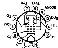
14R ANODE = G_2 + G_4 + CL FOCUSING ELECTRODE = G_3
