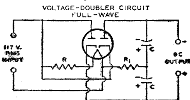
R = HEATERS OF OTHER TUBES IN SERIES WITH VOLTAGE-DROPPING RESISTOR
