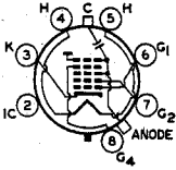
8KP ANODE = G_3 + G_2 + CL FOCUSING ELECTRODE = G_4
