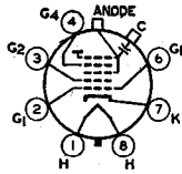
8HR ANODE = G_3 + G_2 + CL FOCUSING ELECTRODE = G_4
