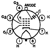
8JR ANODE = G_4 + CL FOCUSING ELECTRODE = G_2
