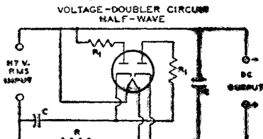
R_1 = PROTECTIVE RESISTOR
