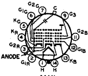
14AU ANODE = G_4 + G_2 + CL FOCUSING ELECTRODE = G_3
