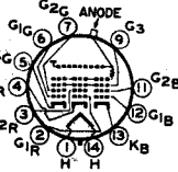
14AH ANODE = G_4 + G_2 + CL + R FOCUSING ELECTRODE = G_3
