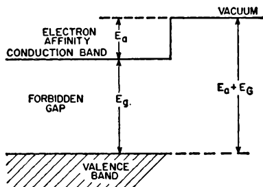
Fig. 5. Energy model of a semiconductor photoemitter.
