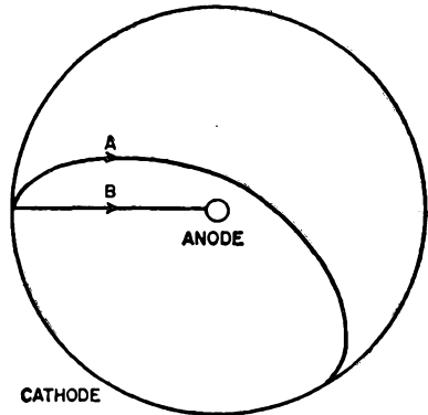
Fig. 15. Paths of electrons in a tube having cylindrical geometry. Directions of emission velocities are (a) tangential and (b) radial.
