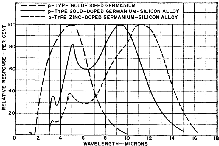
Fig. 87. Spectral response of infrared-sensitive detectors.
