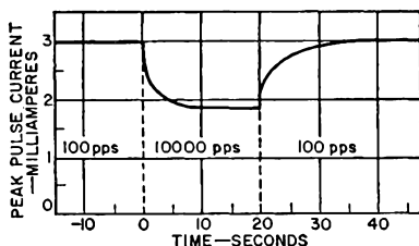
Fig. 70. Variation of output pulse height as the rate of pulsing is changed in a poorly designed experimental tube. Light pulses were provided from a cathode-ray tube. At the left of the graph, which shows the pulse-amplitude envelope with time for the output of the multiplier phototube, the pulses are at 100 per second. The pulse rate is increased suddenly to 10,000 per second and again reduced as indicated. Changes in amplitude are probably the result of insulator charging.
