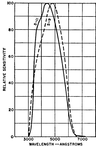
Fig. 37. Comparison of the S-9 and S-11 spectral response characteristics. Both curves are for transmission-type cesium-antimony photocathodes. The S-11 response was evolved to provide maximum blue response for scintillation counting.
