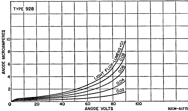
TYPICAL ANODE CHARACTERISTICS
