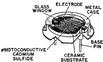
Fig. 71. Typical RCA cadmium-sulfide photocell.
