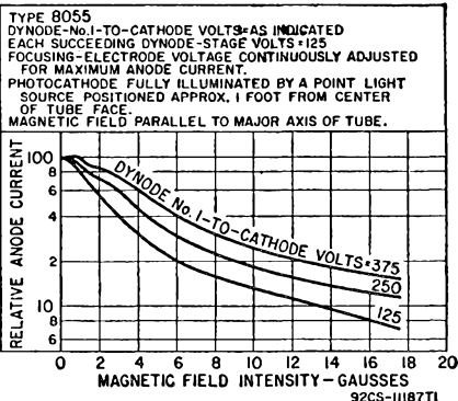
TYPICAL ANODE-CURRENT CHARACTERISTICS
