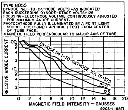
TYPICAL ANODE-CURRENT CHARACTERISTICS
