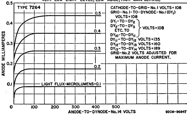
TYPICAL ANODE CHARACTERISTICS VERY-LOW-LIGHT-LEVEL, LOW-NOISE, HIGH-GAIN SERVICE
