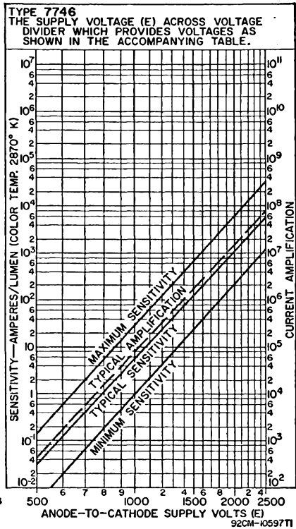
SENSITIVITY AND CURRENT AMPLIFICATION CHARACTERISTICS
