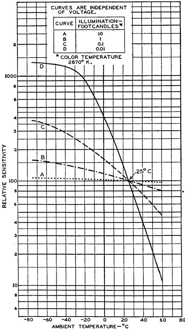
Fig. 79. Sensitivity as a function of temperature for a cadmium-sulfide cell.
