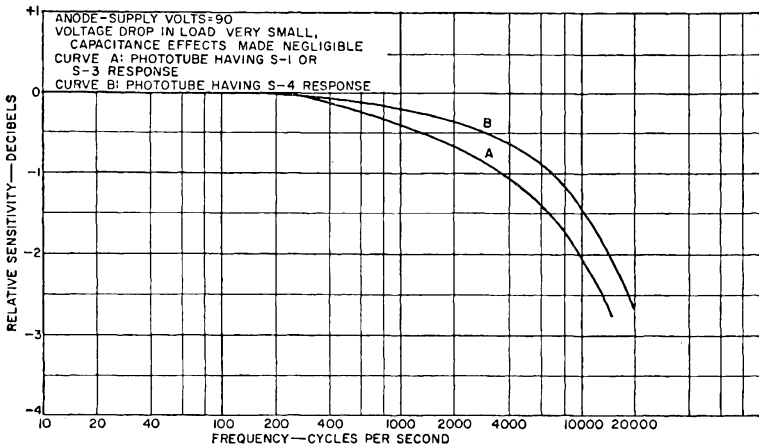
Fig. 28. Frequency response of gas-filled phototubes: (a) Response of a tube having S-1 spectral response (Ag-O-Cs photocathode) (b) Response of a tube having S-4 spectral response (Cs-Sb).
