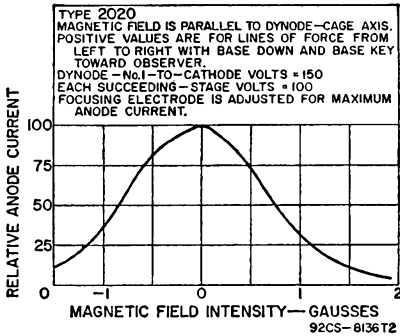
EFFECT OF MAGNETIC FIELD ON ANODE CURRENT
