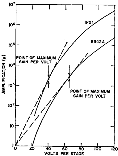
Fig. 36. Log of gain as a function of volts per stage for a tube (IP21) with Cs-Sb dynodes and for a tube (6342A) with Cu-Be dynodes.
