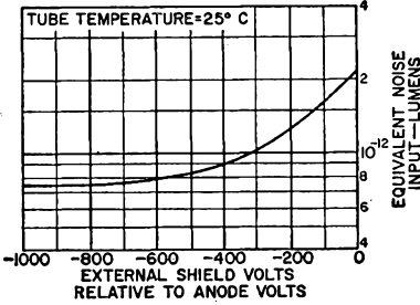
Fig. 47. Effect of external-shield potential on the noise of a 1P21 multiplier phototube. Note the desirability of maintaining a negative bulb potential.
