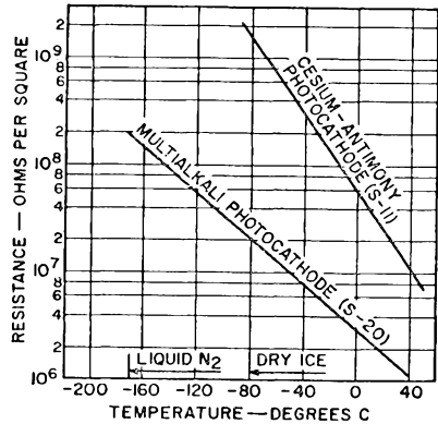
Fig. 63. Resistance per square as a function of temperature for the Cs-Sb and the multialkali semitransparent photocathodes. These data were obtained with special tubes having connections to parallel conducting lines on the photocathode.
