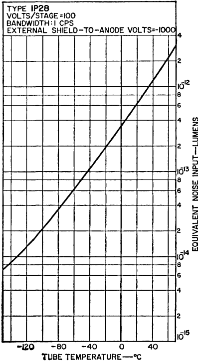
EQUIVALENT-NOISE-INPUT CHARACTERISTICS
