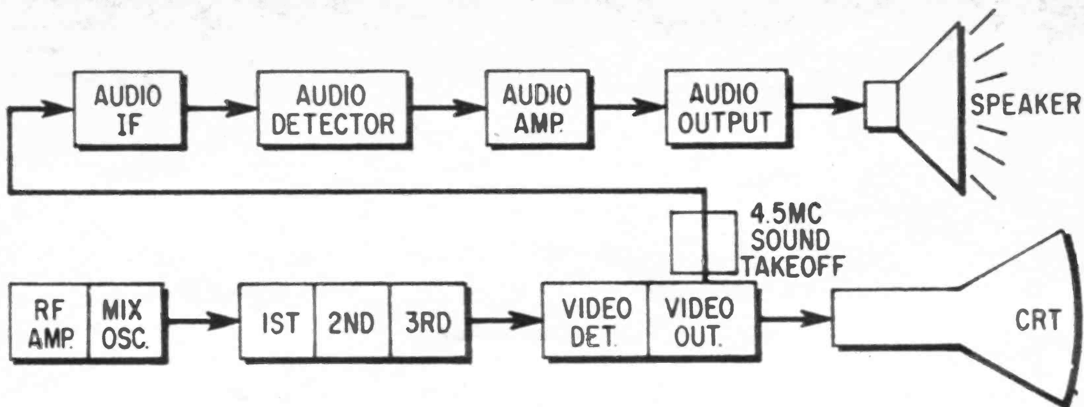
The audio in a black-and-white TV is usually taken off in the video output with a 4.5 MC sound can. The audio in a color TV has its own separate sound detector that works alongside the video detector.
