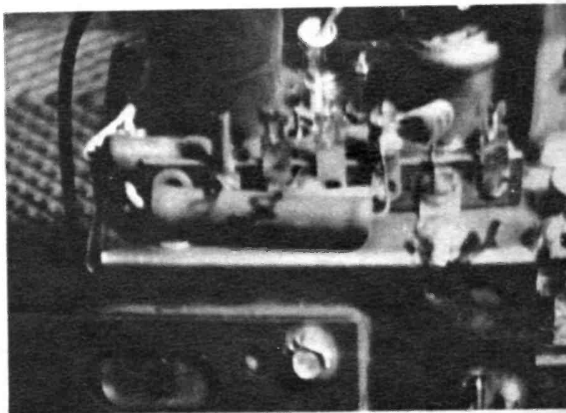
Look for broken charred resistors going into tuner. When these open they kill B plus, cause snow.
