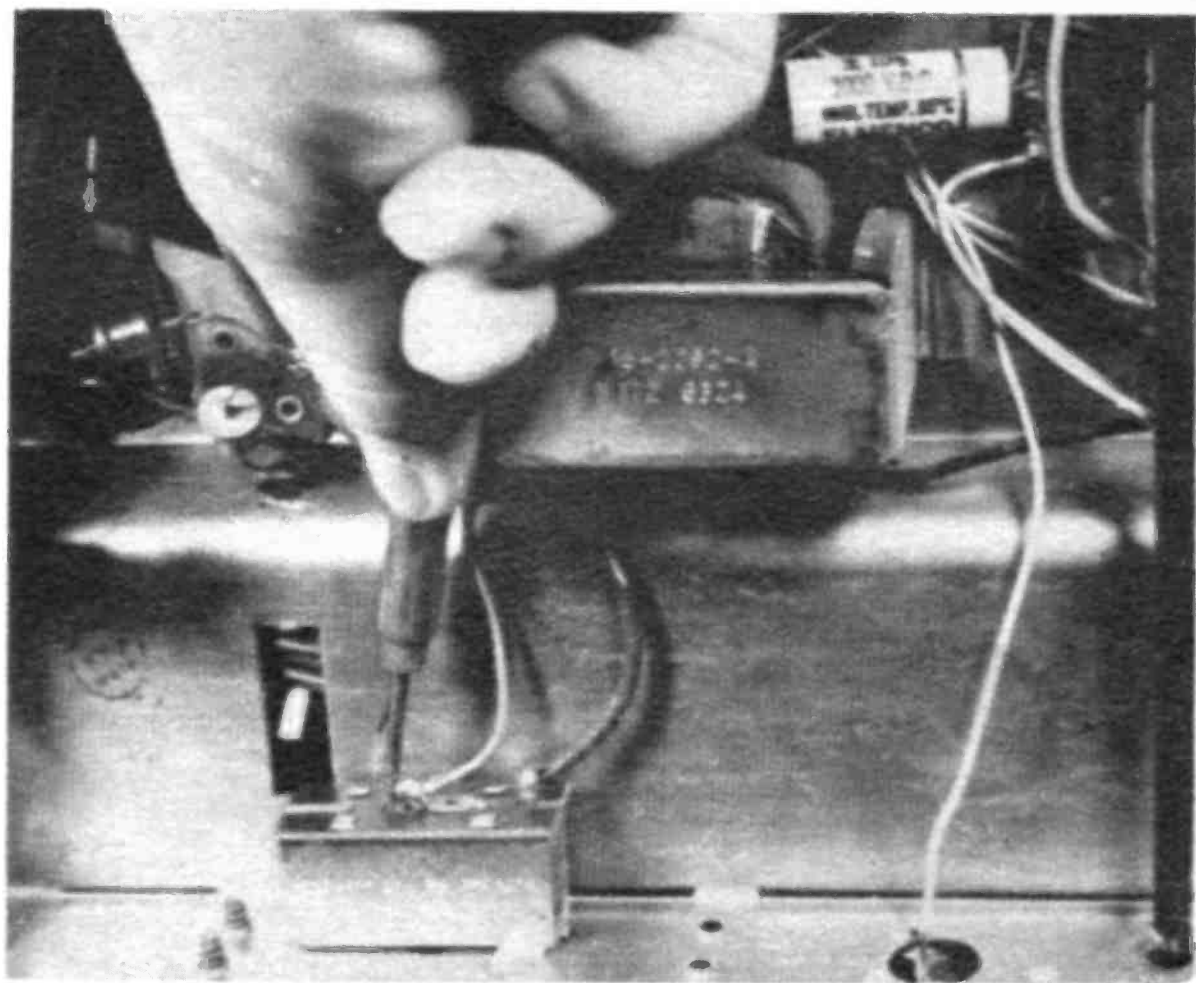
Some circuit breakers have a screw-type adjustment. By turning it in, its amperage is increased.
