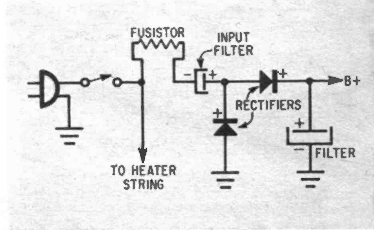
Other part of the power supply, the B plus line, contains a fusistor, rectifiers and input filter.
