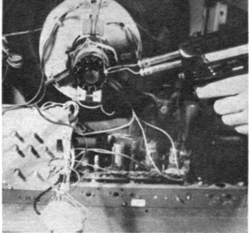
If you can heat pins with a solder gun and add solder in addition to crimping, repair is sure.
