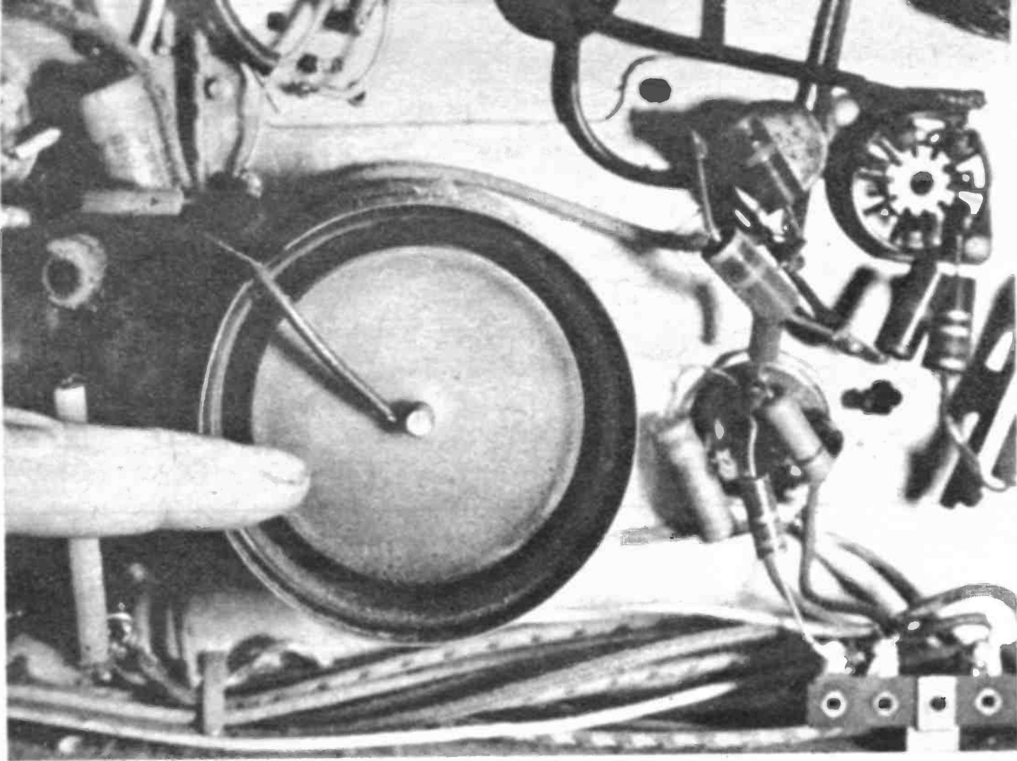
Thick plastic covers are placed on rectifier bottoms to insulate it from chassis. Breaks can cause corona.
