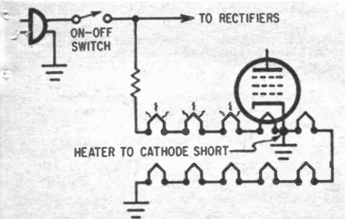
In series wired TV should the tubes light overly bright, a lit tube is shorted, causing trouble.
