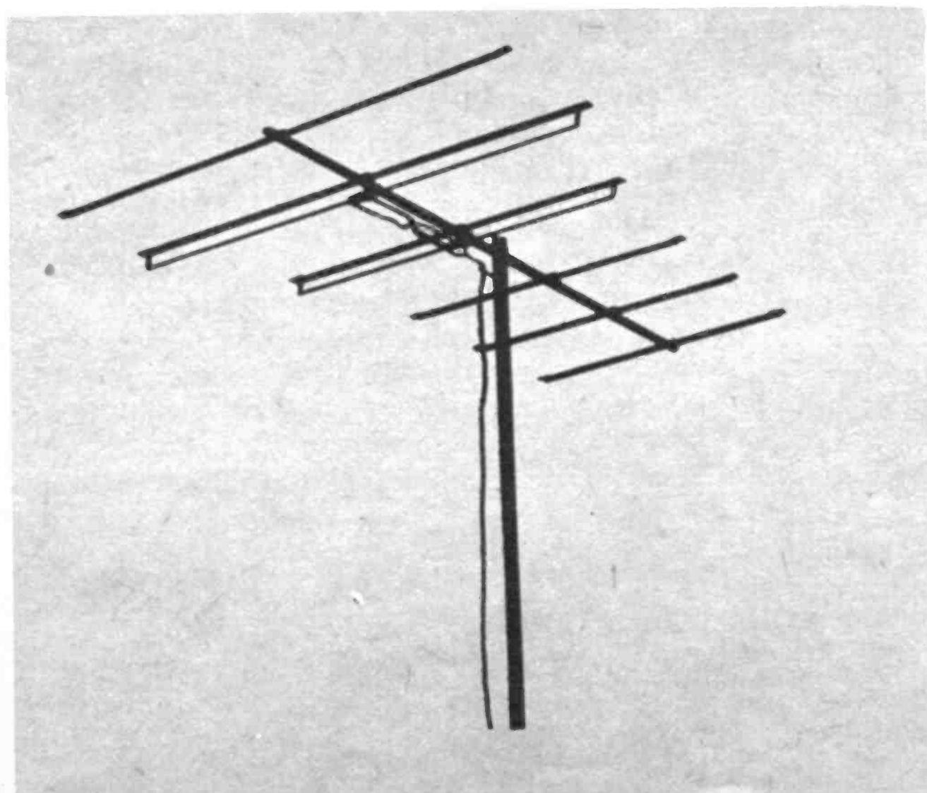
This is a yagi type that pulls channels seven through thirteen. There are all types available. Low band picks up channels 2-6.
