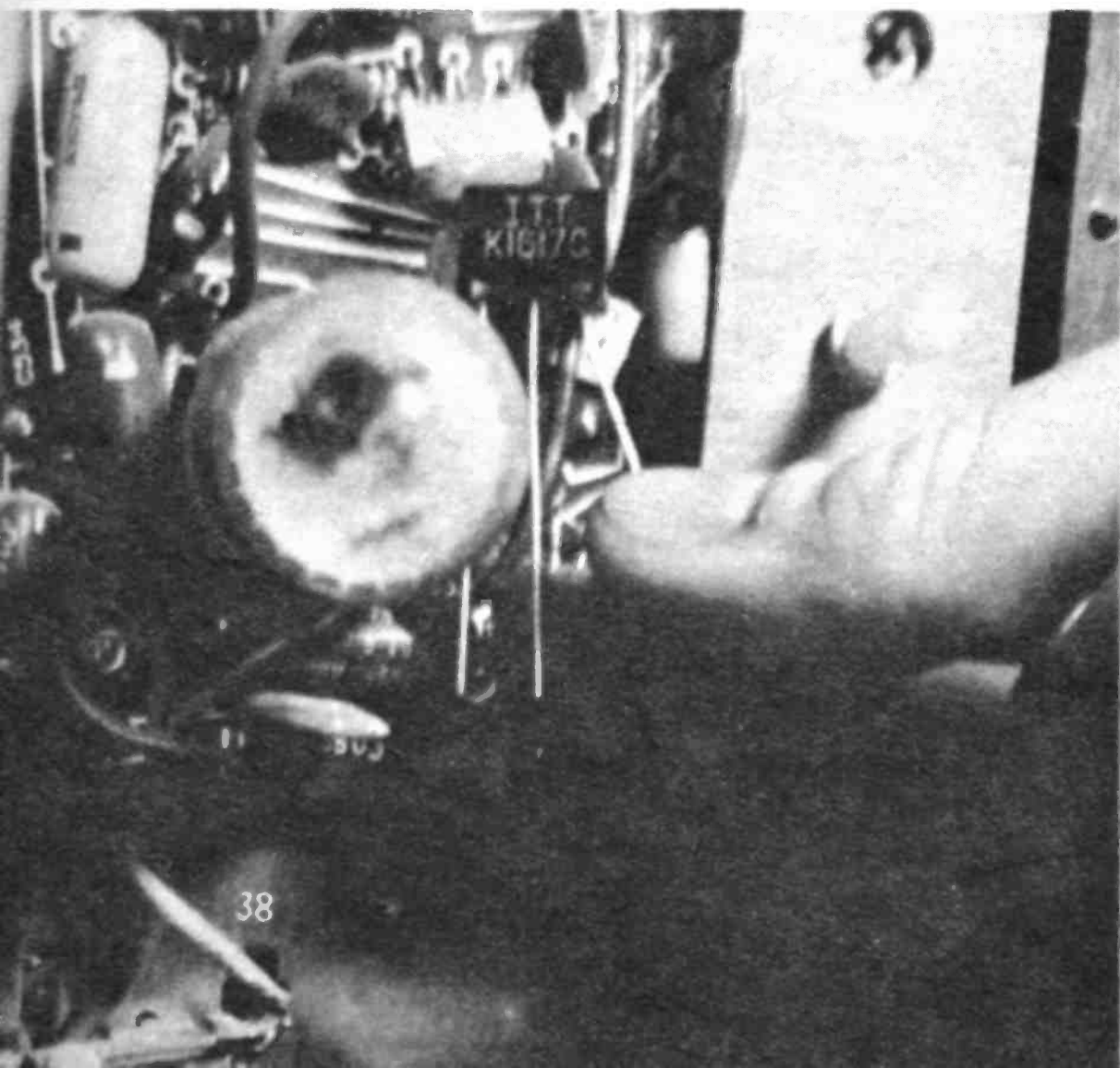
These diodes replace the horizontal phase detector tube. Some plug in but most require soldering.
