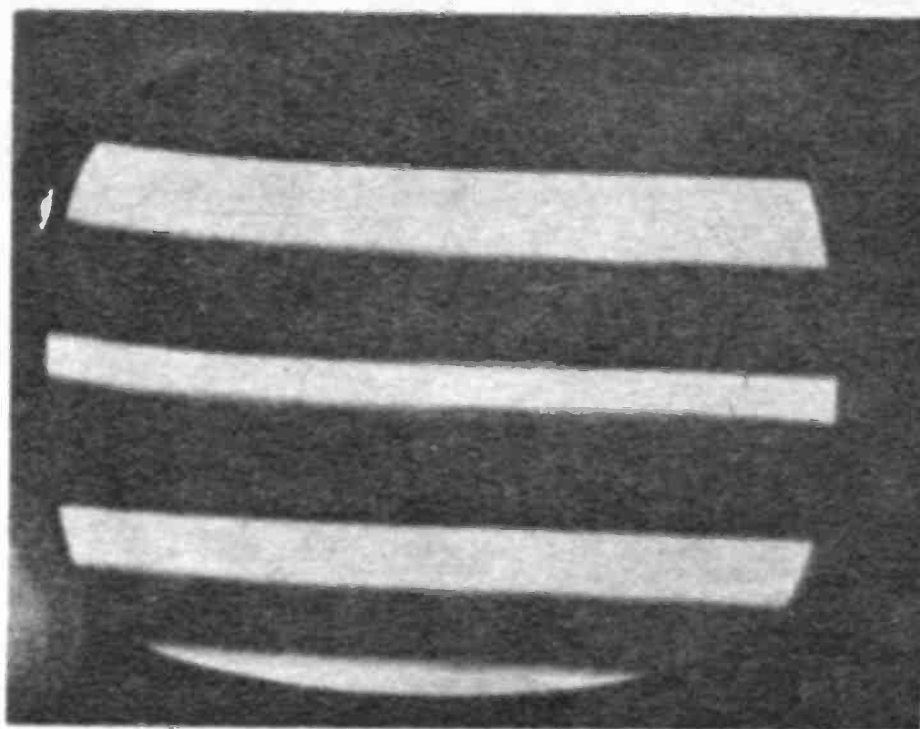
If many hum bars appear along with a motorboat noise, change the mixer-oscillator or IF tubes.
