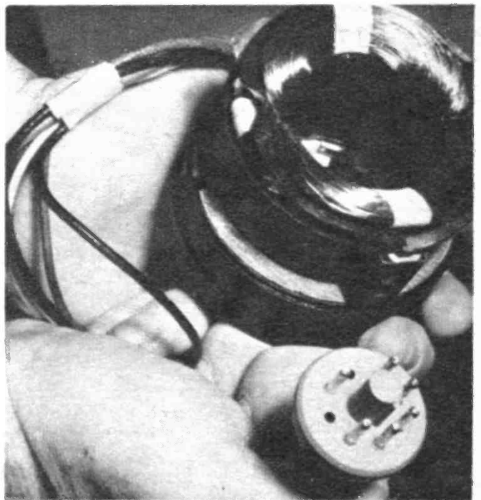
Yoke is mounted around neck of picture tube. It sweeps cathode ray, helps in making high voltage.
