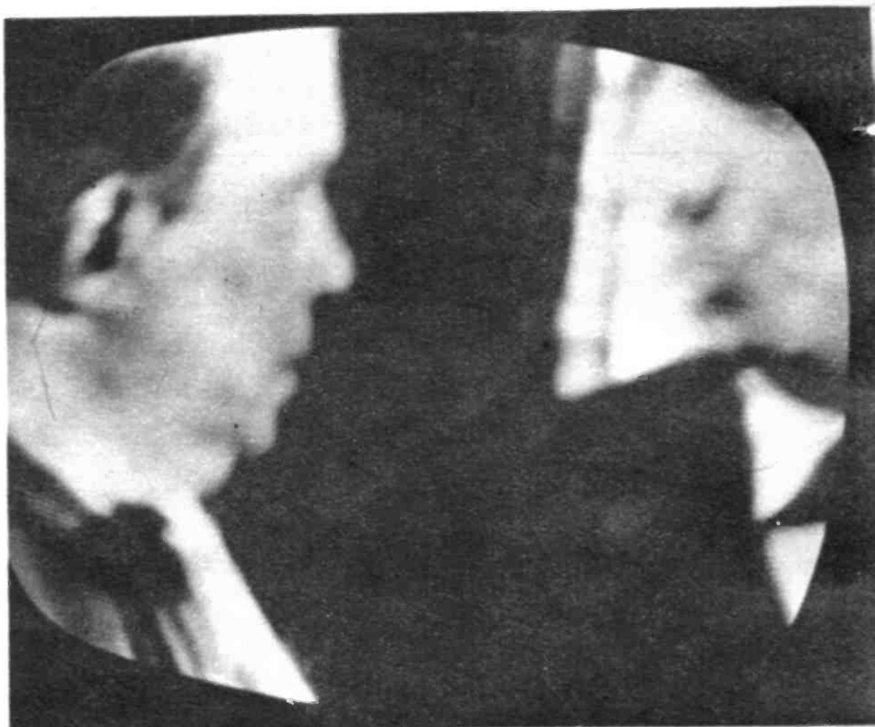
Blooming occurs from low high voltage. Adjusting the brightness control reveals this condition.
