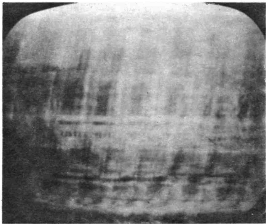
The further away from 15,750 the horizontal oscillator gets the more lines appear on your screen.
