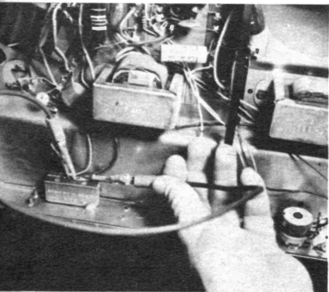
A quick check of the circuit breaker is to short it out. If the TV comes back on, breaker is bad.
