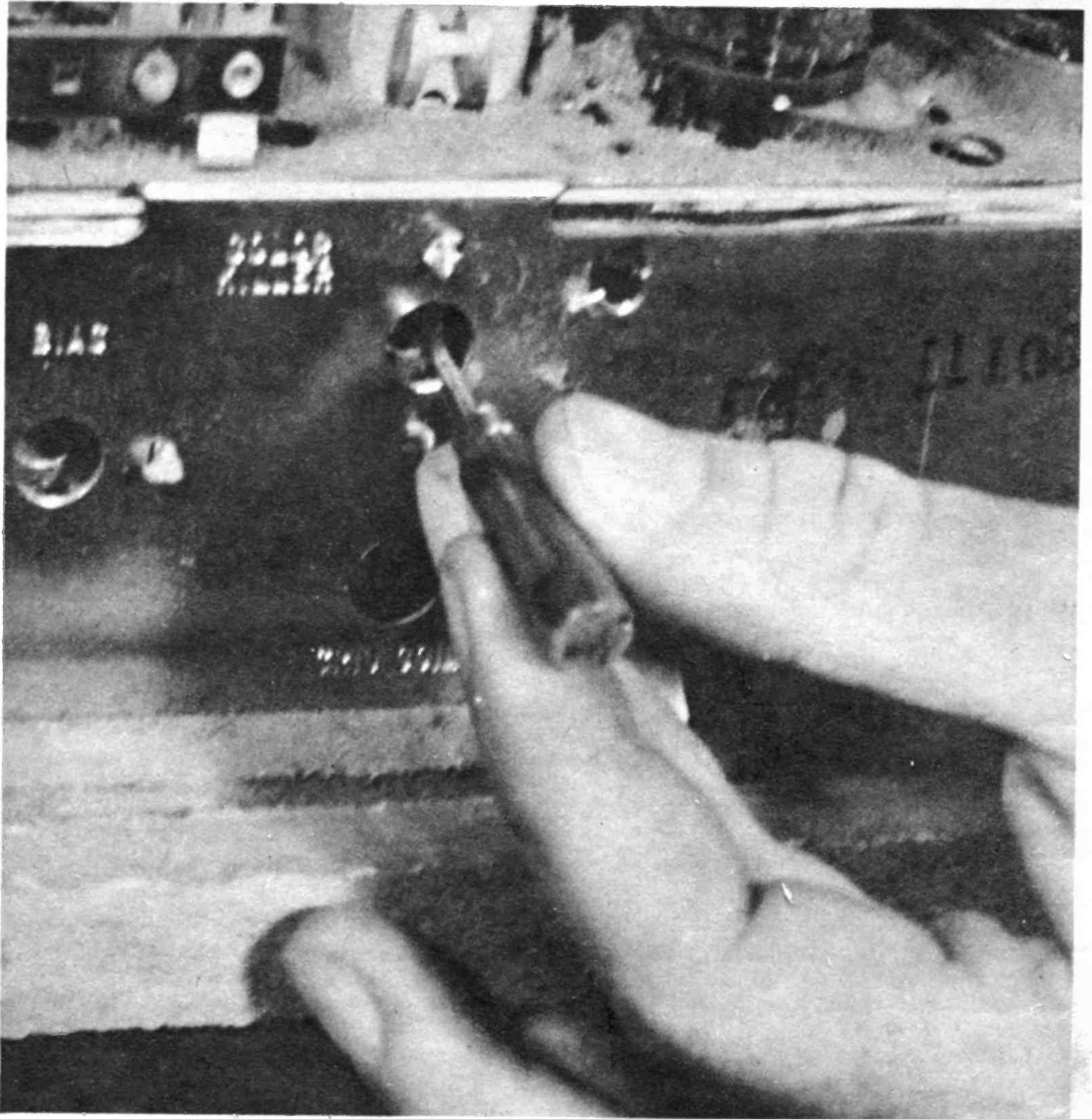
The only color control on the rear panel is the color killer. It sets threshold for color signal input.
