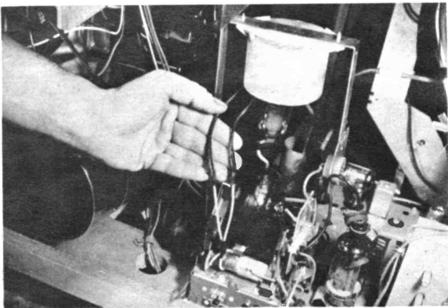
Common cause of high voltage leaking is this rectifier heater winding. Its one turn is easily replaced.
