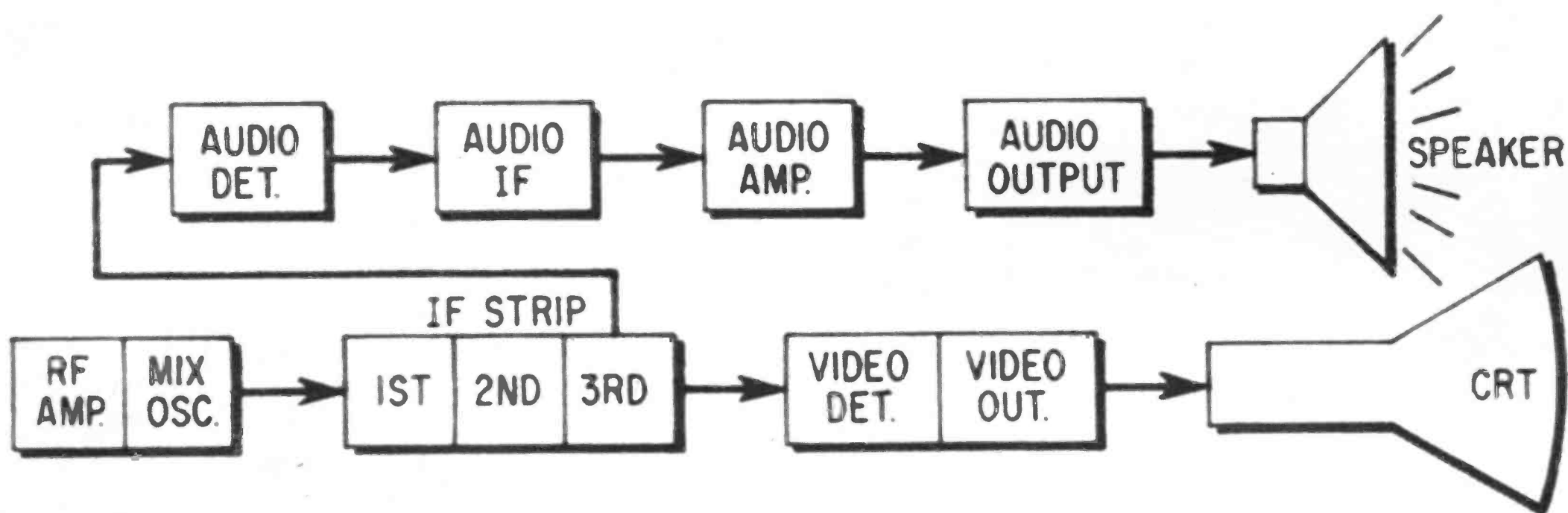
The audio in a black-and-white TV is usually taken off in the video output with a 4.5 MC sound can. The audio in a color TV has its own separate sound detector that works alongside the video detector.
