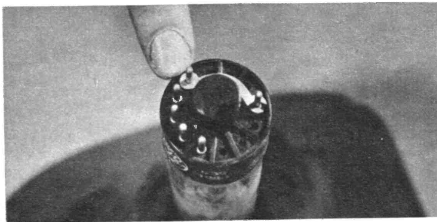
Sometimes a picture tube needs a strap between the heater and the focus anode mounted in electron gun.
