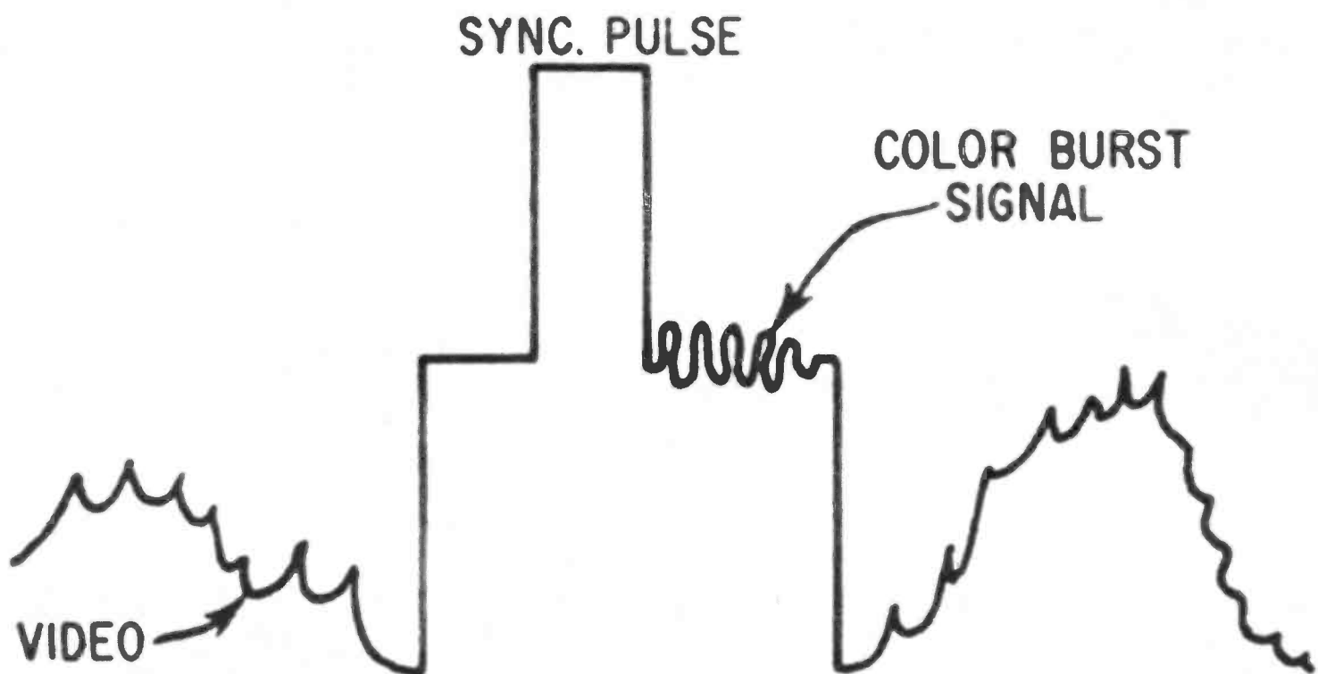
Color burst is found on the back porch of composite color signal near horizontal and vertical.
