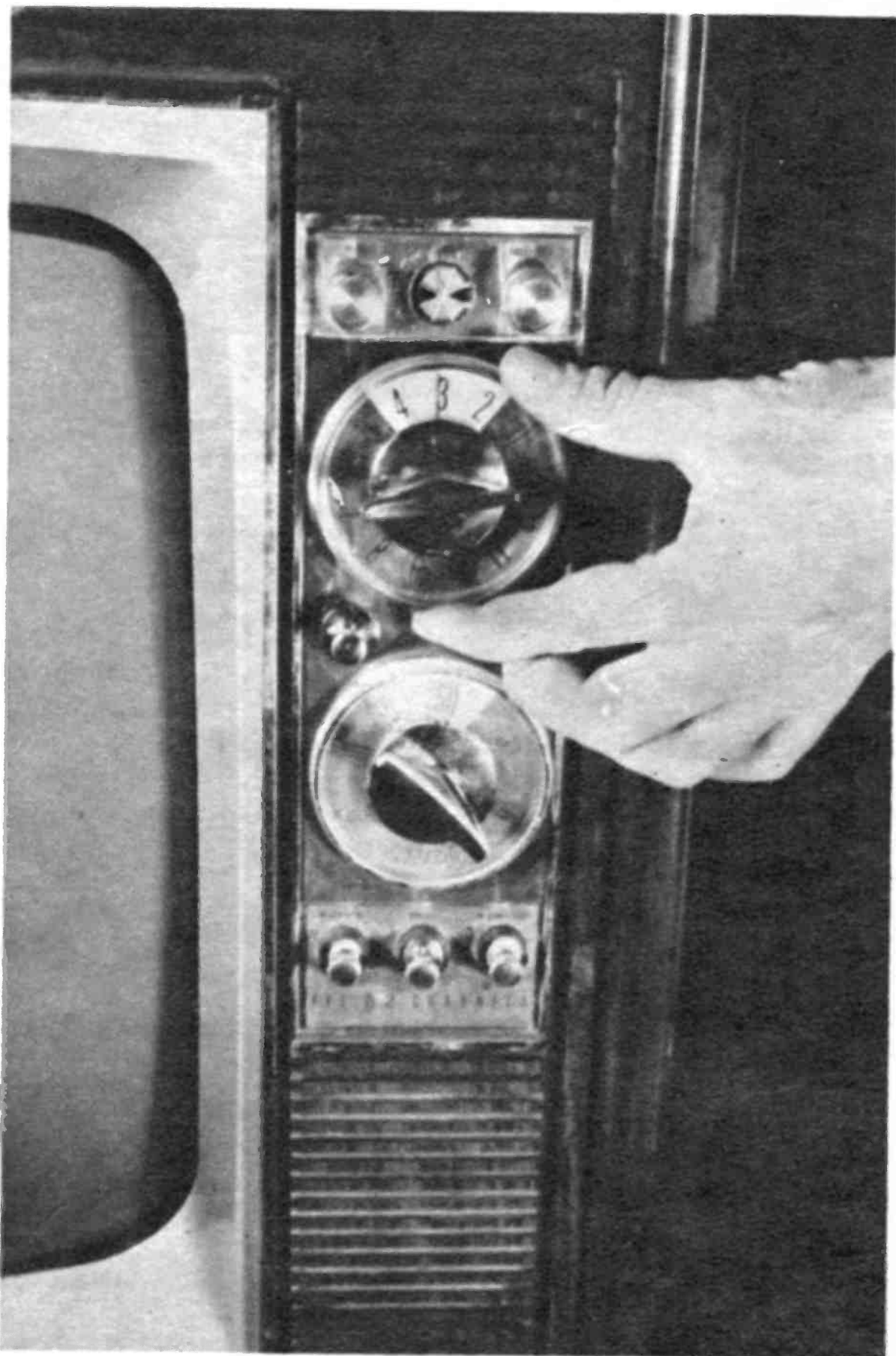
The fine tuner serves an important function for color. With a wrong setting you can lose color.
