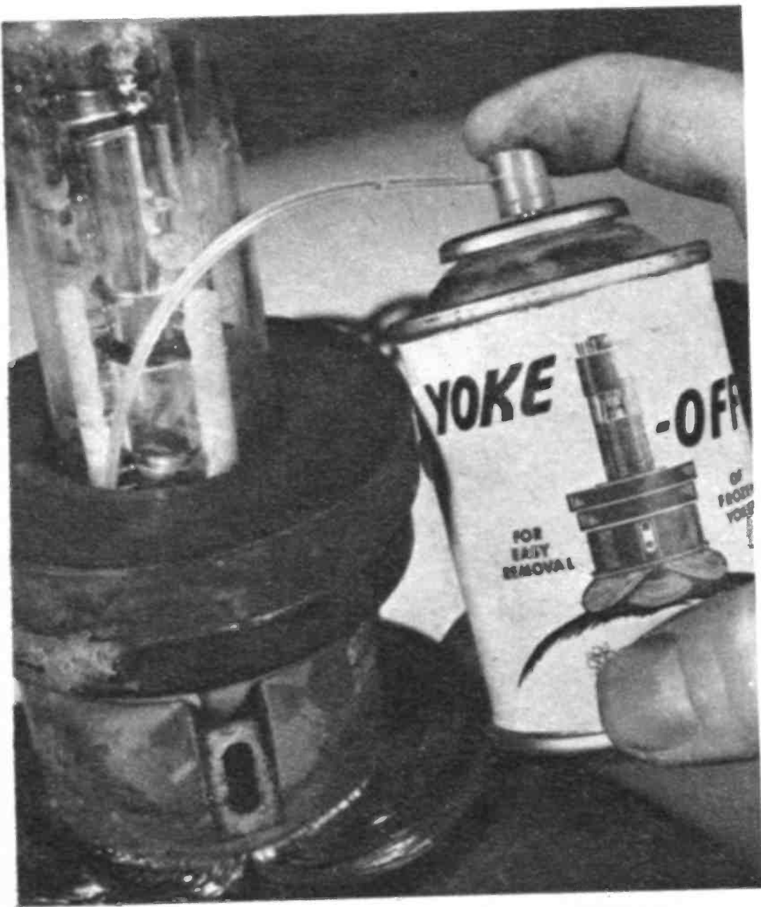
When a yoke freezes to the glass neck, it can be loosened easily with this special yoke loosener.
