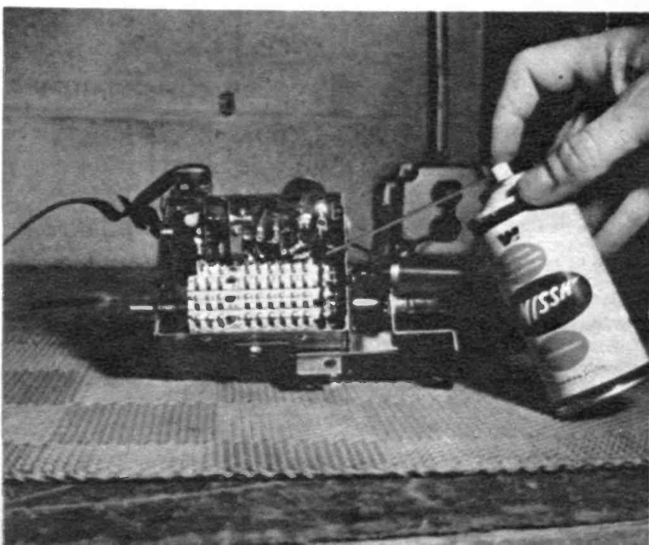
A quick clean job for minor erratic action is to spray tuner lube into tuner, rotate slowly.
