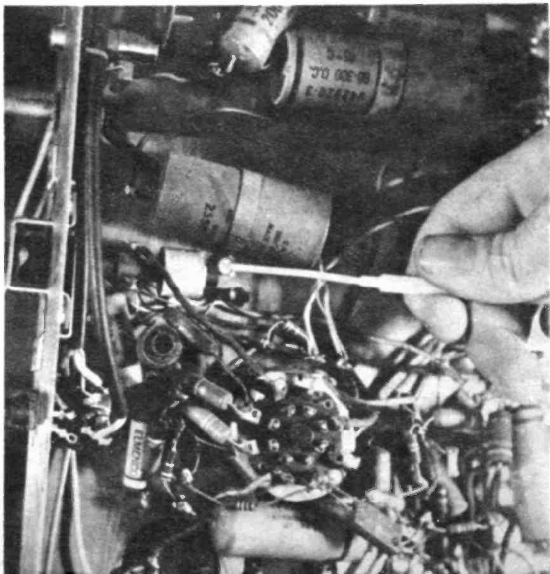
Never use metal screwdriver in horizontal phase coil. It has electrical effects, can crumble coil.
