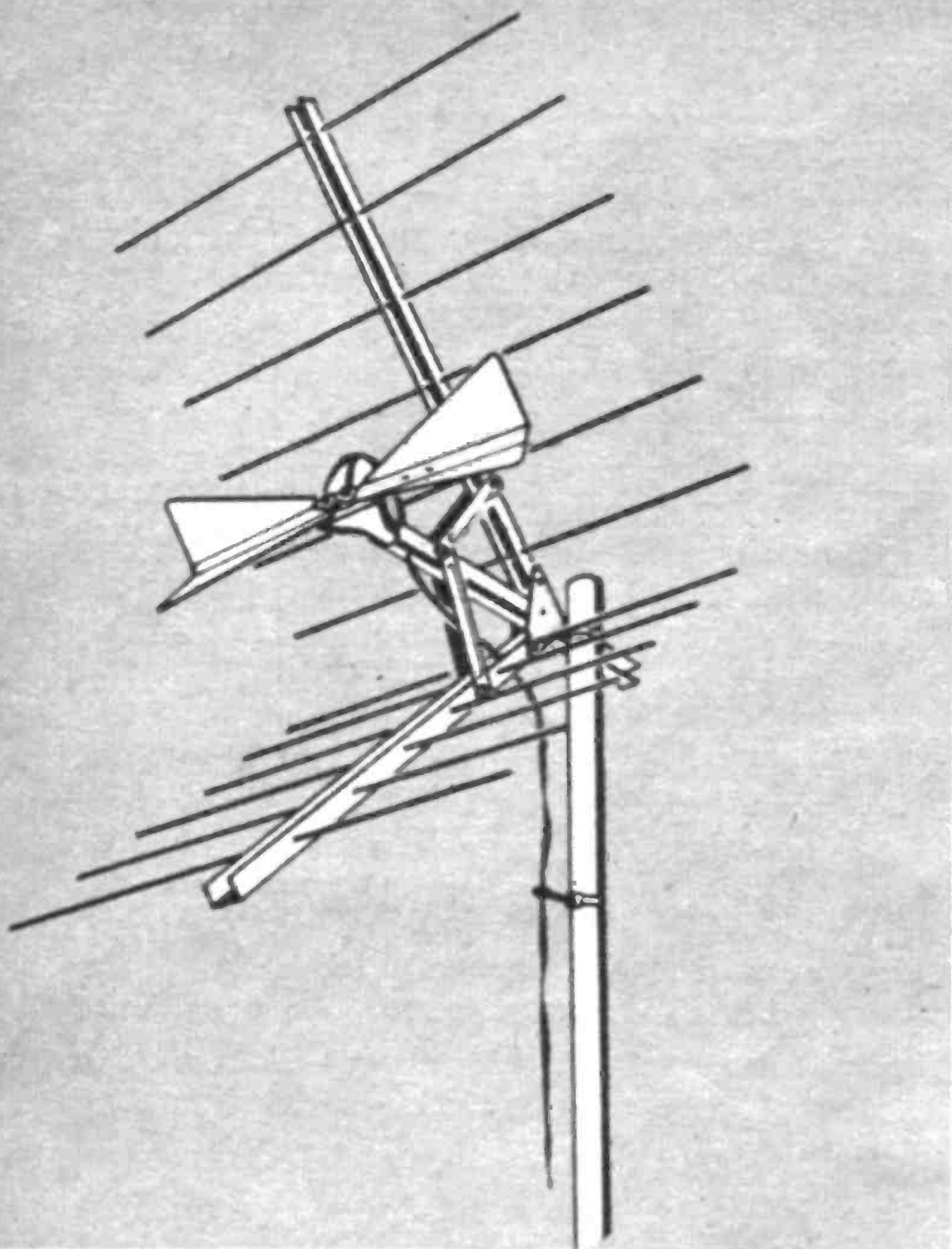
One of the typical UHF antennas is the corner reflector. It can pull reception up to 60 miles.
