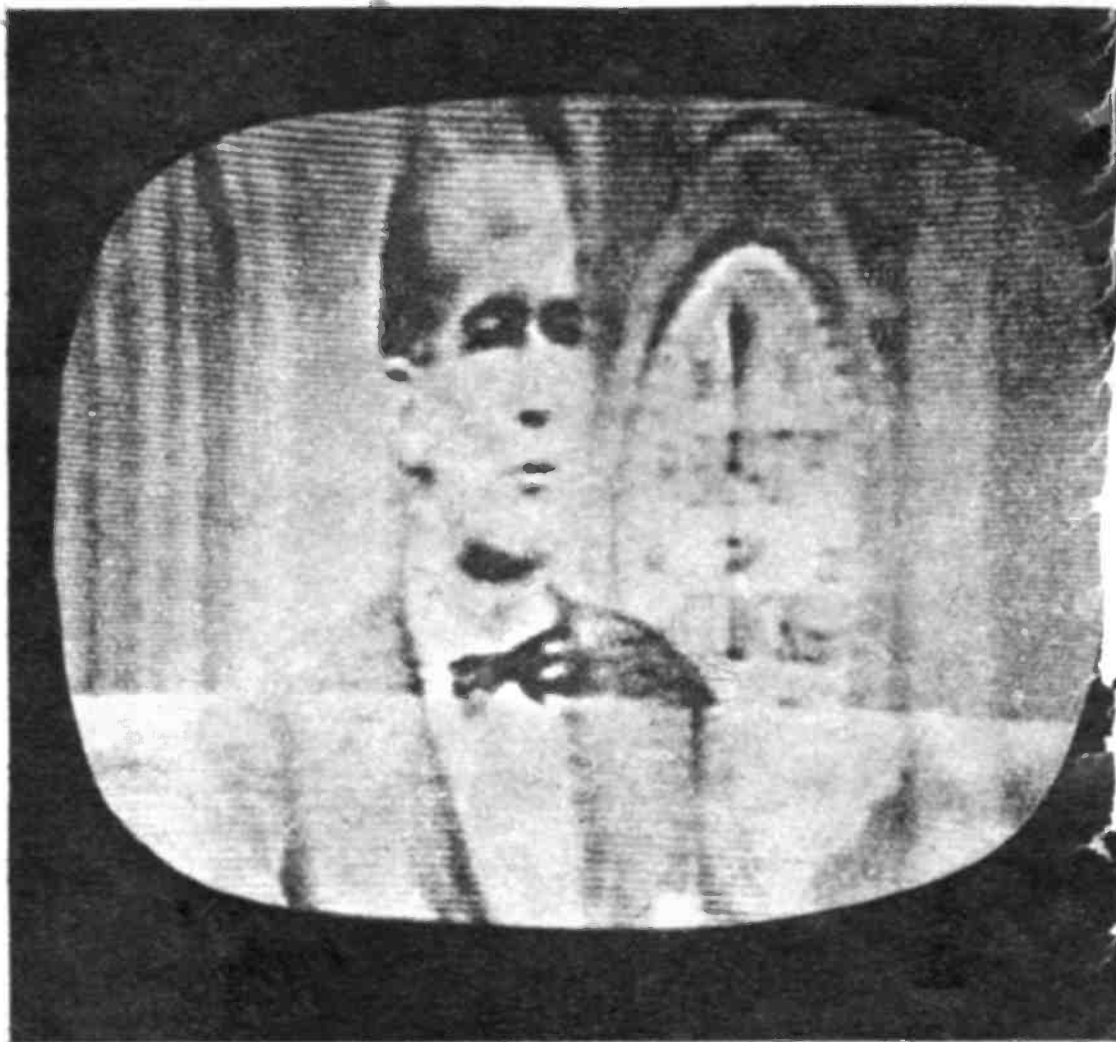
Pointed heads, long legs with whitish haze at bottom of screen indicate gassy vertical output tube.
