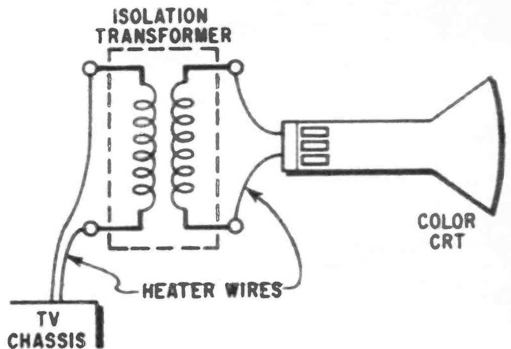
Any correctly rated 1:1 transformer can be installed directly into the heater leads of color CRT.
