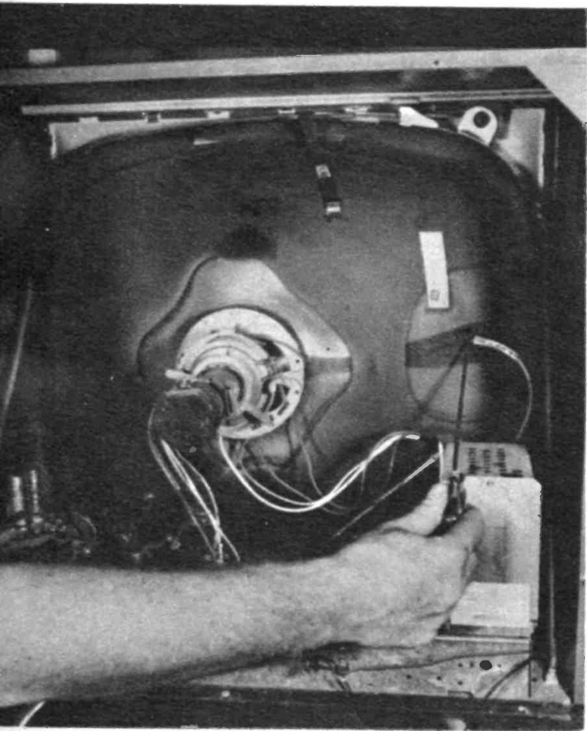
Be careful removing anode button. There are different kinds and sometimes it stores electricity.
