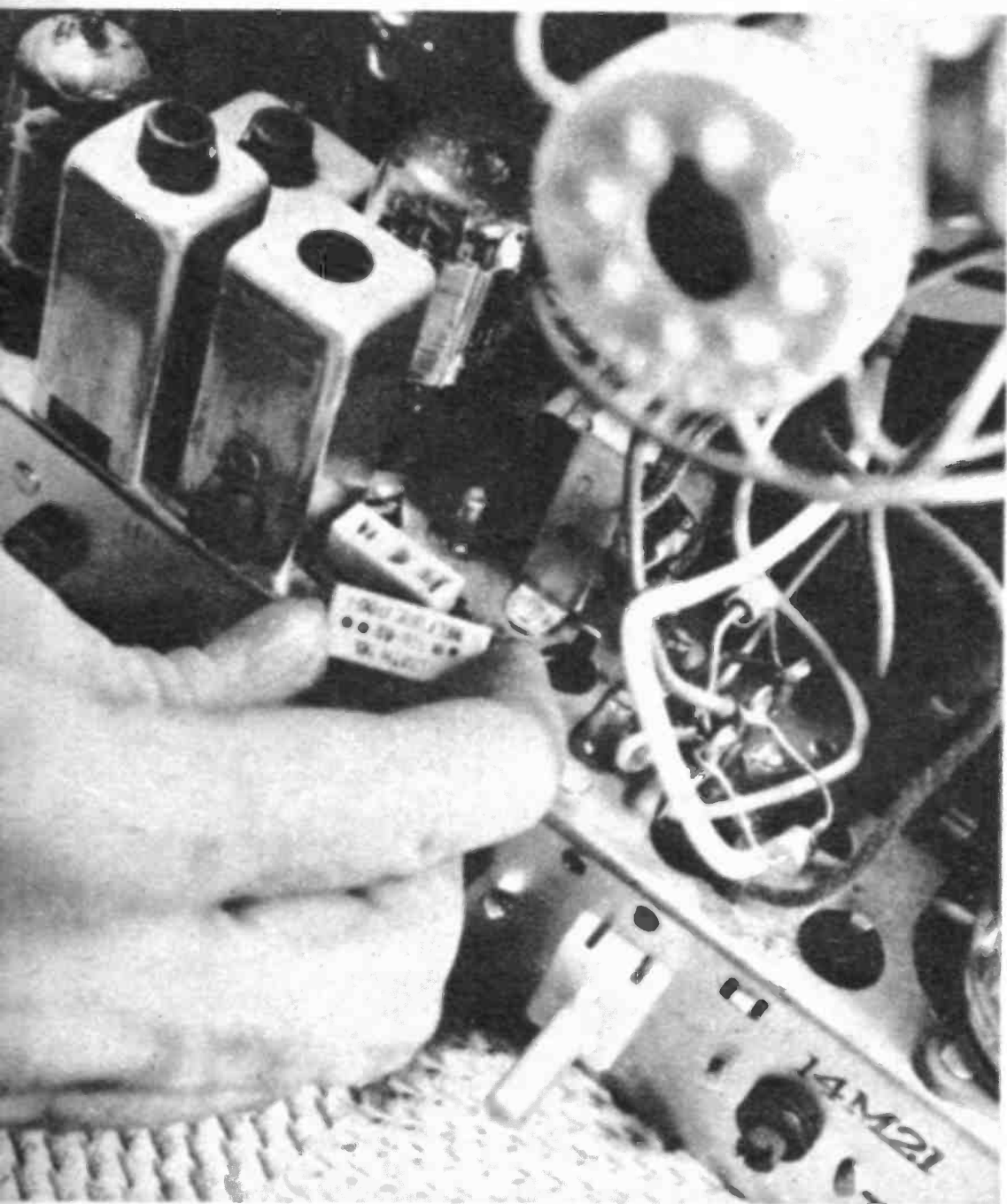
Commonest B plus symptom is blown fusistor. Most times it just opens itself or is caused by short.
