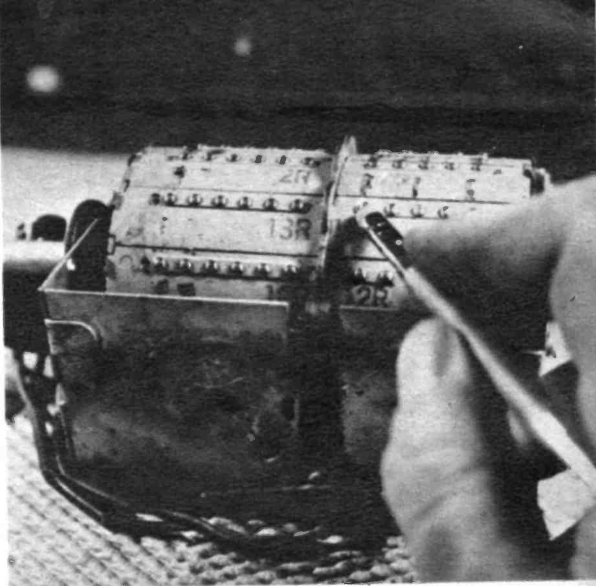
If spray won't work, use ordinary eraser to get the carbon off the contacts and then spray them.
