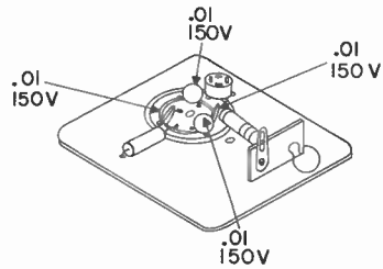
CAPACITANCE BRIDGE
