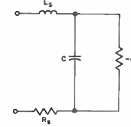
EQUIVALENT CIRCUIT (BIASED IN NEGATIVE CONDUCTANCE REGION)
