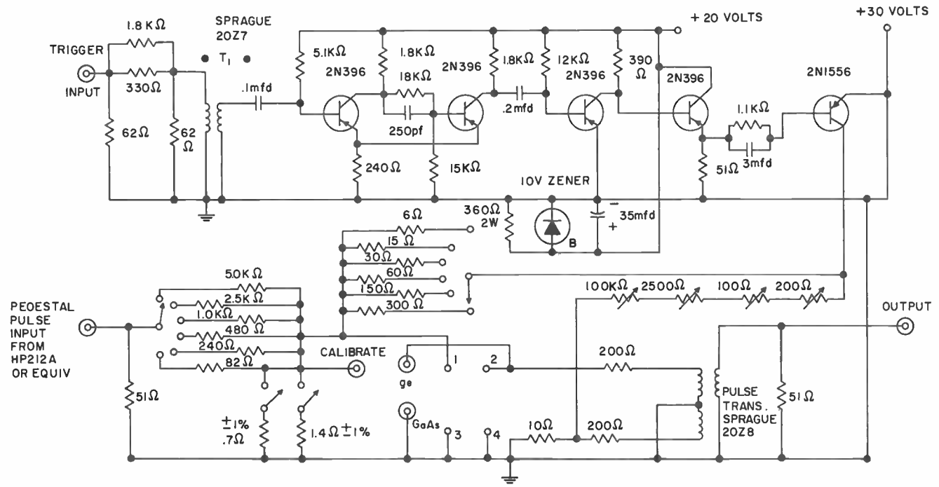
R 8 TEST SET DIAGRAM FIGURE 7.15
