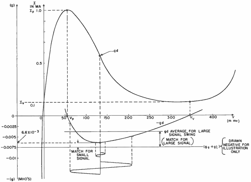
CONDUCTANCE VERSUS VOLTAGE — CHARACTERISTIC FIGURE 3.9
