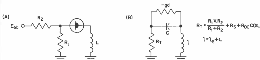
SIMPLE "SERIES" OSCILLATOR AND EQUIVALENT CIRCUIT
