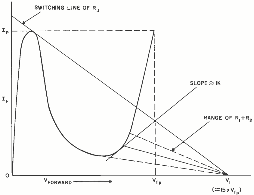
OPERATING REGION AND LOAD LINE
