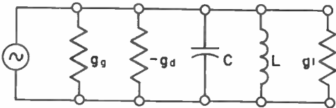
EQUIVALENT CIRCUIT OF A TUNNEL DIODE "PARALLEL" AMPLIFIER
