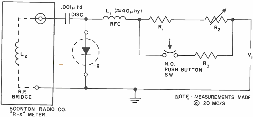
BASIC TUNNEL DIODE CAPACITANCE TEST CIRCUIT
