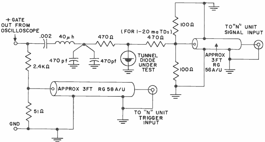
RISETIME TEST SET CIRCUIT DIAGRAM FIGURE 7.17
