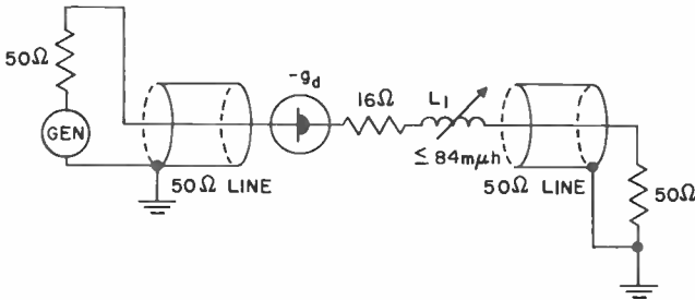
AC CIRCUIT OF 100 Mc/s AMPLIFIER STAGE
