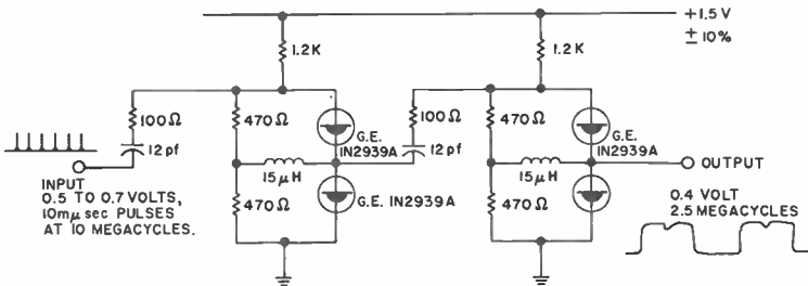
TUNNEL DIODE TWO STAGE COUNTER
