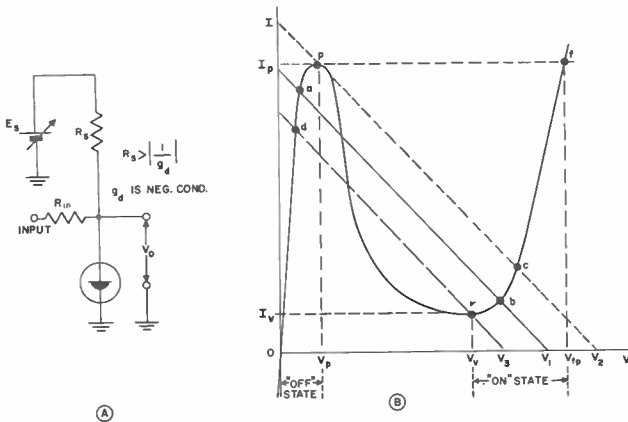
SIMPLE TUNNEL DIODE BISTABLE CIRCUIT
