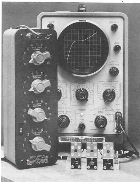
DETERMINATION OF TERMINAL NEGATIVE RESISTANCE
