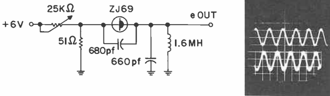
100 Kc/s SINEWAVE OSCILLATOR CIRCUIT AND OUTPUT WAVEFORMS
