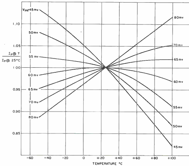
VARIATION OF NORMALIZED I_p WITH TEMPERATURE FOR DIFFERENT VALUES OF V_p
