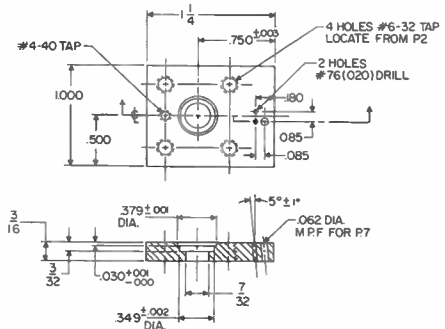
③ BOTTOM PLATE MATERIAL : BRASS
