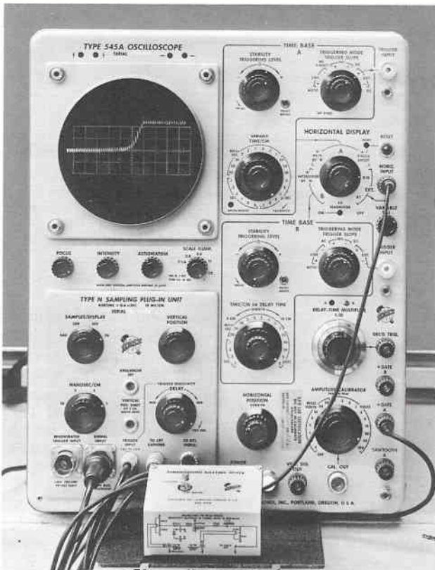
PHOTOGRAPH OF RISE TIME TEST SET UP FIGURE 7.18
