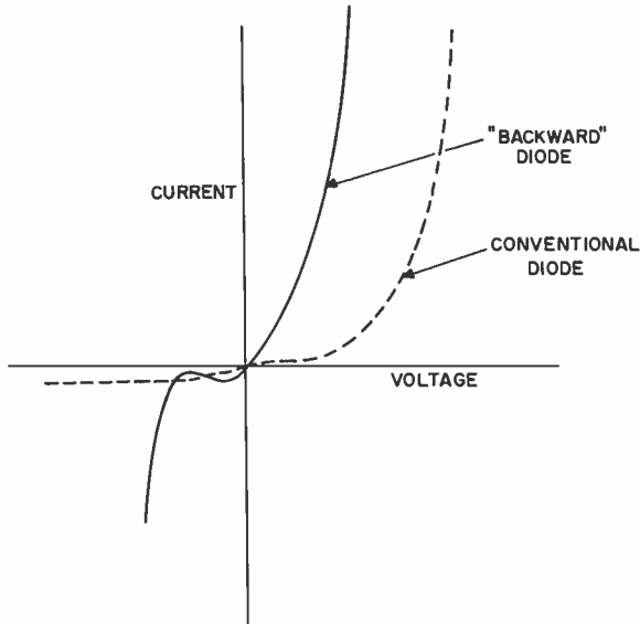
COMPARISON BACKWARD AND CONVENTIONAL DIODE CHARACTERISTIC
