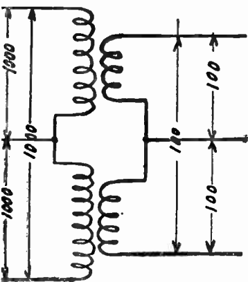
Open Delta or "V"
