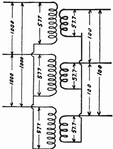
Star-Star Connection of Transformers
