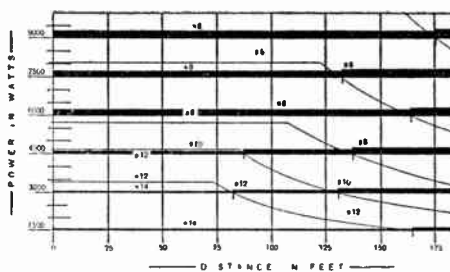
Fig. 19—Conductor Size Based on Voltage Drop (230-Volt Branch Circuit—2½ Drop)
