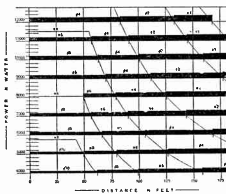
Fig. 20—Conductor Size Based on Voltage Drop. (230-Volt Branch Feeder—1% Drop)
