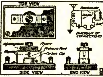
The mechanism of the Electrolytic Detector is almost a duplicate of that of the crystal detector...
