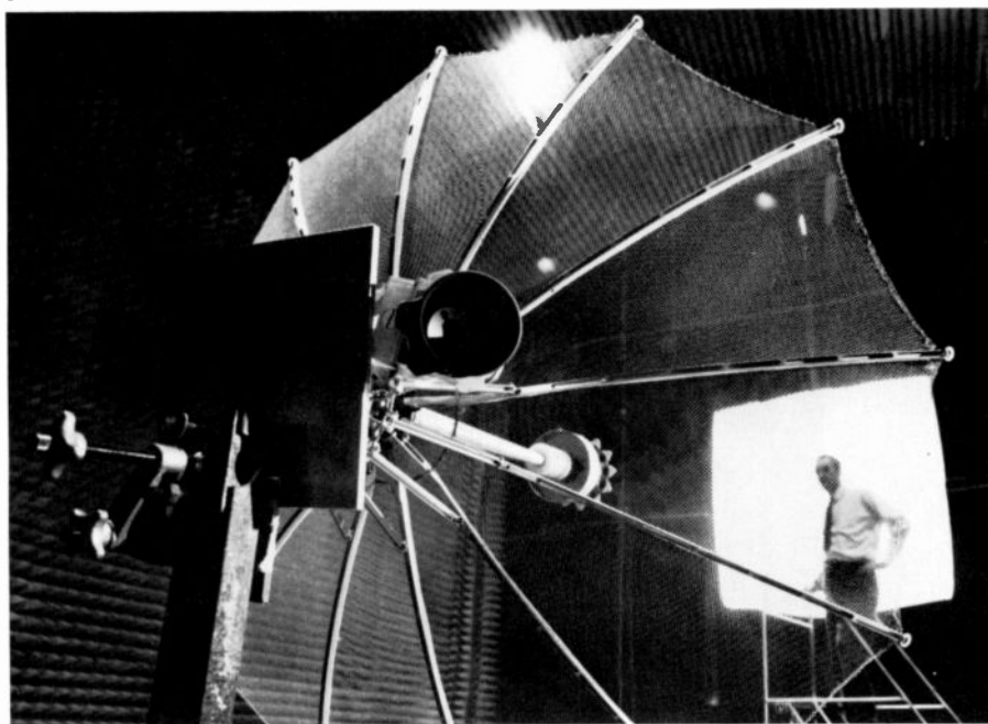
16. An engineer at RCA's Missile and Surface Radar Division, Moorestown, N.J., supervises space chamber tests of a folding antenna of the kind that will transmit color TV and other communications from Apollo 15 astronauts' Lunar Rover "space taxi" as it roams the moon. The antenna, with spined sections of gold mesh, opens and closes like an umbrella.
