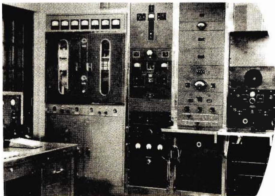
Phasing equipment for directional antenna, speech input equipment, Hammarlund Radio Receiver
