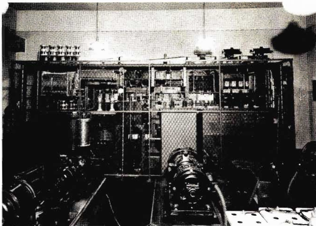
Power Room, rear view of 5kw Western Electric transmitter
